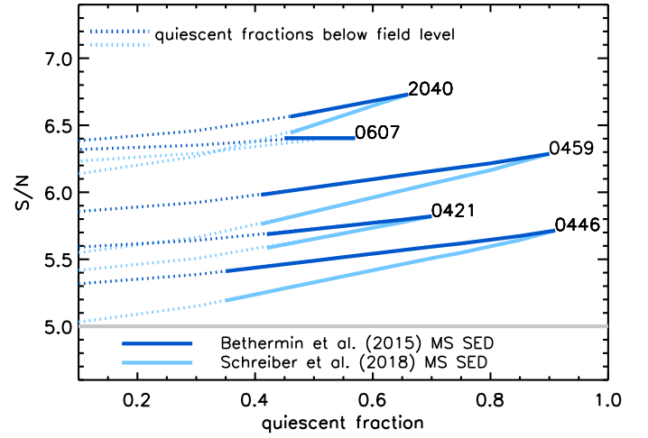
Fig. 11: Retrieved S/N of the cluster SZE detection obtained as a function of the r < 0.45r_{500} quiescent fraction, from the observed value down to the field level (solid lines) at the cluster redshift and mass completeness limit (see Sect. 5.4). Dotted lines show for completeness the retrieved S/N for central quiescent fractions down to 10%. For each cluster, the S/N is shown for both MS SEDs adopted to convert SFRs to 95, 150 GHz fluxes, as indicated. The gray line marks the S/N > 5 limit of our original sample selection. According to the modeling in Sect. 5.4, all five clusters would have been included in our S/N > 5 sample even if environmental quenching were negligible.
