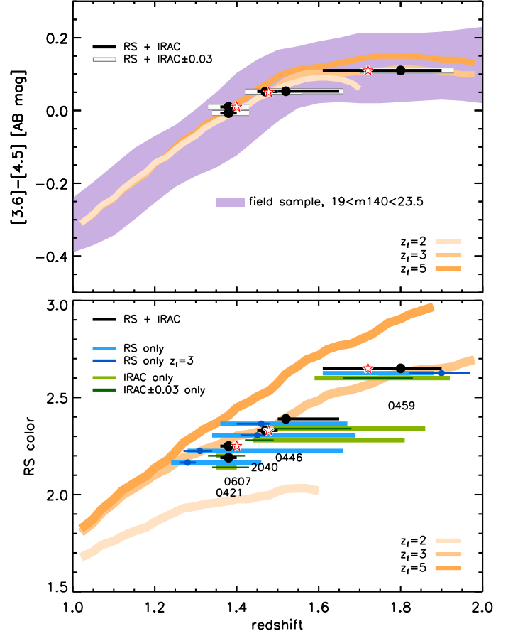
Fig. 5: Photometric redshift constraints for all clusters (black points with 1\sigma errorbars reported in both panels) as determined with the simultaneous modeling of the red sequence (RS) and [3.6]-[4.5] color in Sect. 4. Red stars show the spectroscopic redshifts for SPT-CLJ2040 and SPT-CLJ0607, as well as the best current constraint for SPT-CLJ0459 (see Sect. 4). Bottom panel – Adopted model RS m814-m140 color at M^* vs. redshift, for formation redshifts 2 < z_f < 5 (orange lines). Light blue bars show the 1\sigma constraints from modeling only the RS color (dark blue assuming z_f = 3 ). Light green bars show constraints from the [3.6]-[4.5] color alone. Top – Adopted model [3.6]-[4.5] color vs. redshift, for 2 < z_f < 5 as in the bottom panel. The shaded area shows for reference the 16^{\text{th}} - 84^{\text{th}} percentile range of [3.6]-[4.5] color vs. redshift for field galaxies in the magnitude range of our samples ( m140 \leq 23.5 ). Dark green (bottom panel) and white (top panel) bars show the impact on the best-fit redshift (from IRAC color alone and RS + IRAC color, respectively) of a \pm 0.03 AB mag systematic offset on the [3.6]-[4.5] color.
