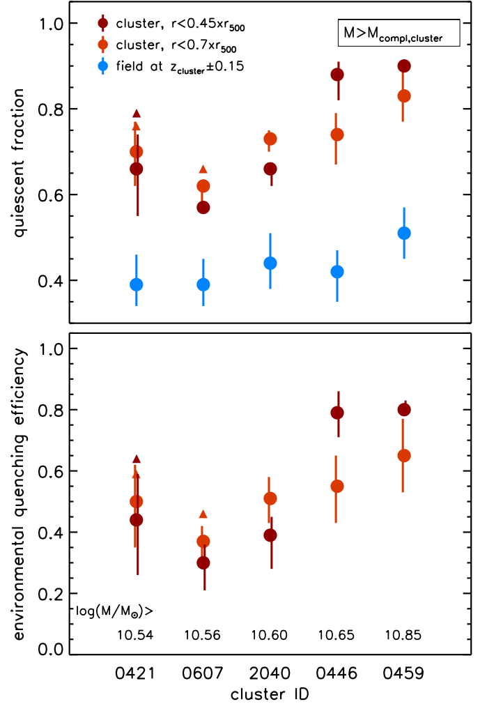
Fig. B.1: Top : Quiescent fraction of cluster galaxies within r < 0.45r_{500} (dark red) and r < 0.7r_{500} (light red) above the mass completeness limit of each cluster as reported in the bottom panel. Error bars account for uncertainties in the quiescent vs. star-forming classification as described in Sect. 5.3. Blue symbols show the quiescent fraction in corresponding photo- z selected control field samples (see Sect. 5.3). Bottom : Environmental quenching efficiency as derived from cluster and field quiescent fractions in the top panel. Color coding reflects the top panel. In both panels empty triangles show, where applicable, the quiescent fraction and derived quenching efficiency assuming that galaxies lacking a quiescent vs. star-forming classification are all quiescent (rather than all star-forming, see Sect. 5.2, Table 2).
