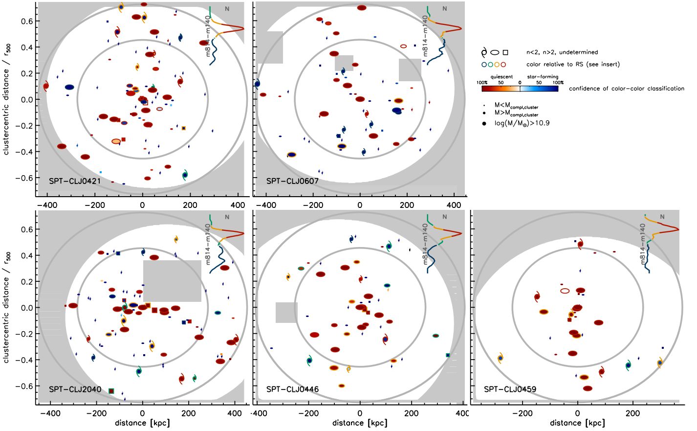
Fig. 9: Projected distribution of candidate cluster members. All candidate members are shown regardless of their statistical background subtraction weight. Each symbol has two colors. The color of the symbol boundary scales with the m814-m140 color of each galaxy relative to the cluster RS color (see insert). The internal symbol color, in red or blue shade according to the galaxy classification as quiescent or star-forming, scales with the reliability of this classification only accounting for the distance of the galaxy colors from the adopted selection dividing line and the relevant photometric errors. Symbol shape reflects the estimated Sérsic index as indicated. Masked areas and regions deemed to be outside of our uniform coverage are gray shaded. The two circles show the limiting radii of the adopted cluster regions ( r < 0.45r_{500} , r < 0.7r_{500} ).
