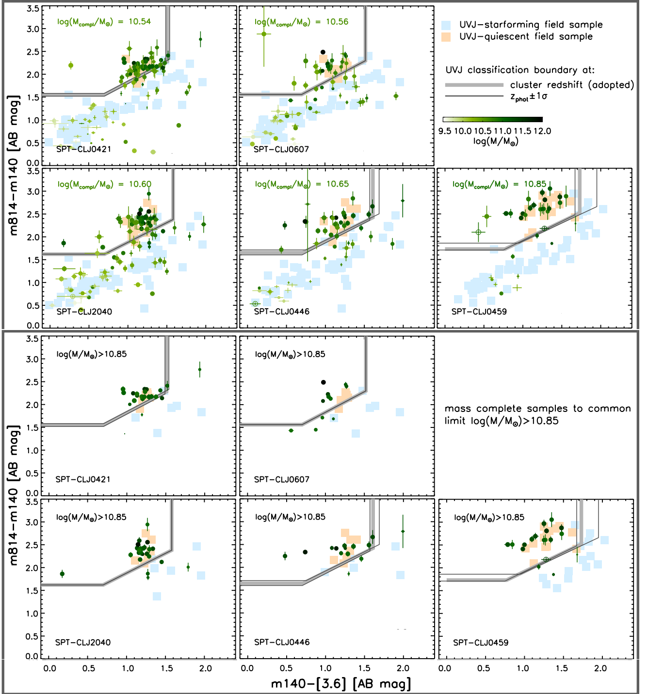
Fig. 6: Adopted quiescent vs. star-forming galaxy classification. The observed m814-m140 vs. m140-[3.6] color-color diagram of candidate members (green points) is shown for all clusters in the r/r_{500} < 0.7 region (the effective area covered for each cluster is indicated). The upper set of panels show m140 -selected (not mass complete) candidate member samples (the mass completeness limit for each cluster is indicated). The lower set of panels show galaxies down to the common stellar mass completeness limit for all clusters, \log(M/M_{\odot}) = 10.85 . Symbol size of green points scales with the statistical background-subtraction weights as in Fig. 1. Symbol color scales with stellar mass as shown by the color bar. Empty symbols show points for which a m140-[3.6] color was inferred using the 4.5\mu\text{m} flux (see Sect. 5.2). Light red and blue squares show, respectively, UVJ-quiescent and UVJ-starforming galaxies from the control field sample with the same magnitude (top panels) or mass (bottom panels) threshold as candidate cluster members, and with a photometric redshift within \pm 0.1 from the cluster redshift. The thick light-gray line shows the adopted quiescent vs. star-forming separation in the observed m814-m140 vs. m140-[3.6] color plane. For clusters without a final spectroscopic redshift confirmation (see Sect. 4), the thin dark-gray lines show the separation that would be adopted if assuming a redshift at the edges of the black+white error bars in Fig. 5 (top).
