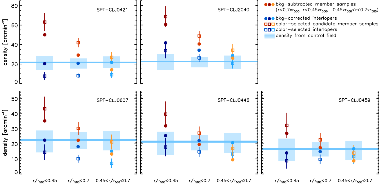
Fig. 3: Projected number density of candidate cluster members (shades of red) and interlopers (blue) in the five clusters as measured in three cluster regions, as indicated. Empty squares show densities for color-selected samples (see Sect. 3.1), and filled circles show how member number density decreases – and interloper density increases – after applying the statistical subtraction of residual background contamination described in Sect. 3.2. The blue line shows the average density of control field galaxies in the same magnitude range adopted for the cluster, with the light-blue shaded areas showing the density variation ( 16^{\text{th}} – 84^{\text{th}} percentiles) in apertures corresponding to the three probed regions. The relative flatness of the interloper density profiles constrains the cluster member sample incompleteness due to member misclassification (see Sect. 3.3).
