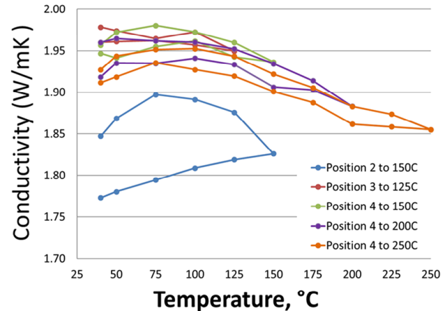
Sample: MK2-B19, All Thermal Conductivity Data
