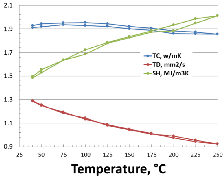
Sample: MK2-B19, small sensor, location 4
