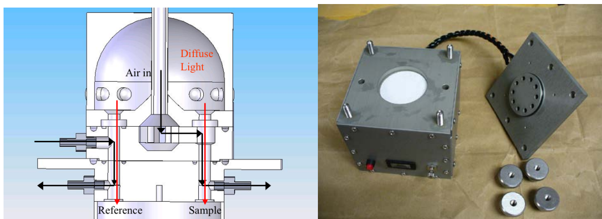
Figure 1. Above is a schematic of the instrument and photo.
