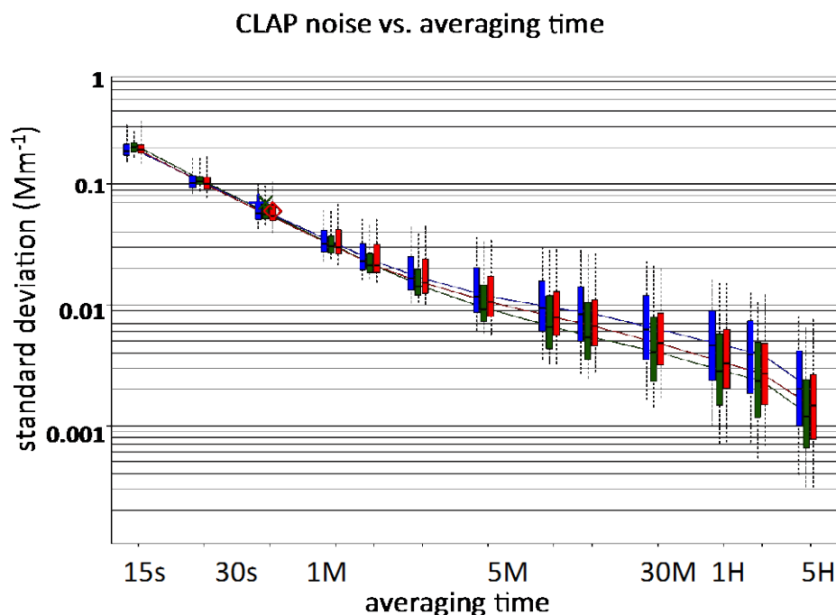
Figure 2. This figure shows an Allen plot showing the sensitivity of 194 CLAP detectors with signal integration time. The signal noise is about 0.1 Mm -1 after 30 seconds of averaging.
