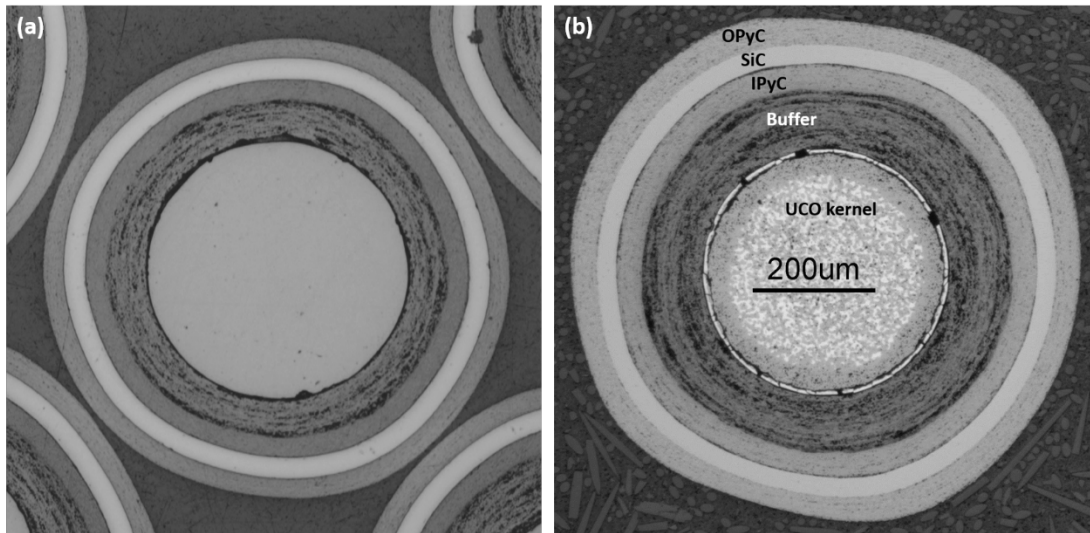
Figure 2. (a) UO_2 TRISO particle with 500 \mu m diameter kernel. (b) UCO TRISO particle with 425 \mu m diameter kernel.
