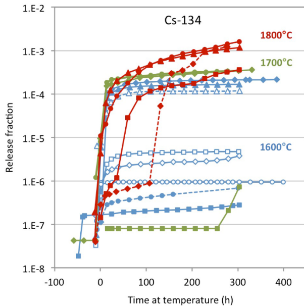
Figure 8. Combined results of ^{134}\text{Cs} release during AGR-1 UCO fuel safety tests in dry helium at 1600 to 1800^\circ\text{C} . Burnup of the fuel specimens ranged from 13.4 to 19.1% FIMA [121].
