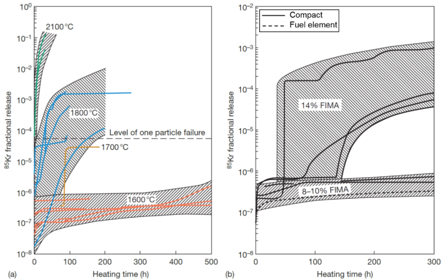
Figure 5. Summary of ^{85}\text{Kr} release fractions during post-irradiation heating tests from the German program (adapted from Ref. 21).
