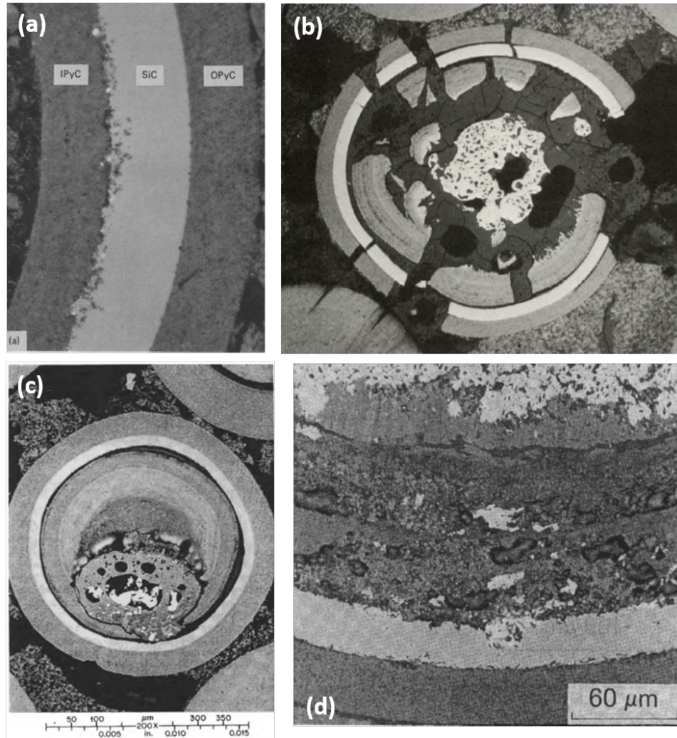
Figure 4. Examples of particle failure mechanisms and coating corrosion. (a) Pd corrosion of SiC in UCO particle [61]. (b) Pressure vessel failure in UO 2 particle [62]. (c) Kernel migration in UO 2 [63]. (d) Predominantly rare-earth corrosion of SiC in UC 2 particle [60]). Images used by permission.
