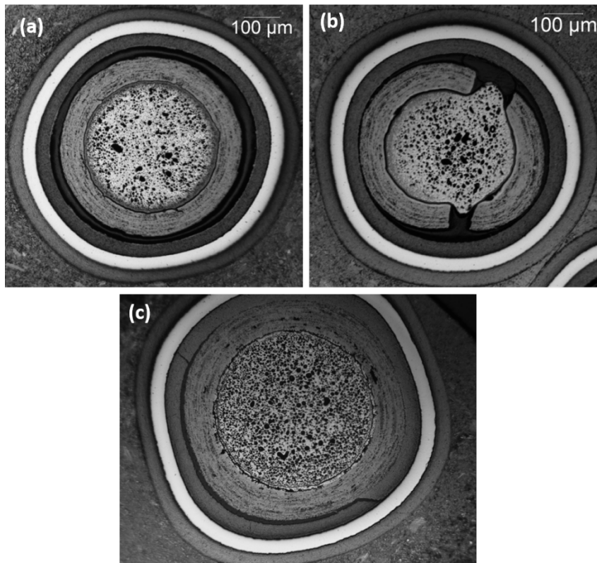
Figure 7. Irradiated UCO particles from the AGR-1 experiment. Particle taken from compacts with an average burnup of 13.7% FIMA ((a) and (b)) and 15.7% FIMA (c).
