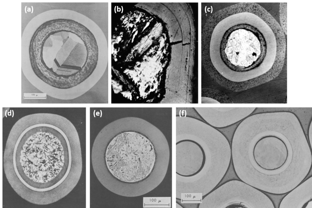
Figure 3. Coated particles from the first decade of development. (a) Early example of a BISO particle. (b) Particles with “laminated” pyrocarbon layer structure demonstrating arresting of crack propagation at the lamination interfaces. (c) Particle with “Triplex” structure (porous buffer layer followed by laminar and columnar pyrocarbon layers). (d) Fertile (Th,U)C_2 particle used in Dragon first charge, consisting of PyC-SiC-PyC structure. (e) Carbide particle with single PyC coating layer used in Peach Bottom first core. (f) “Duplex” (Th,U)C_2 particle used in AVR first core load. Images from References 33,35, used by permission.
