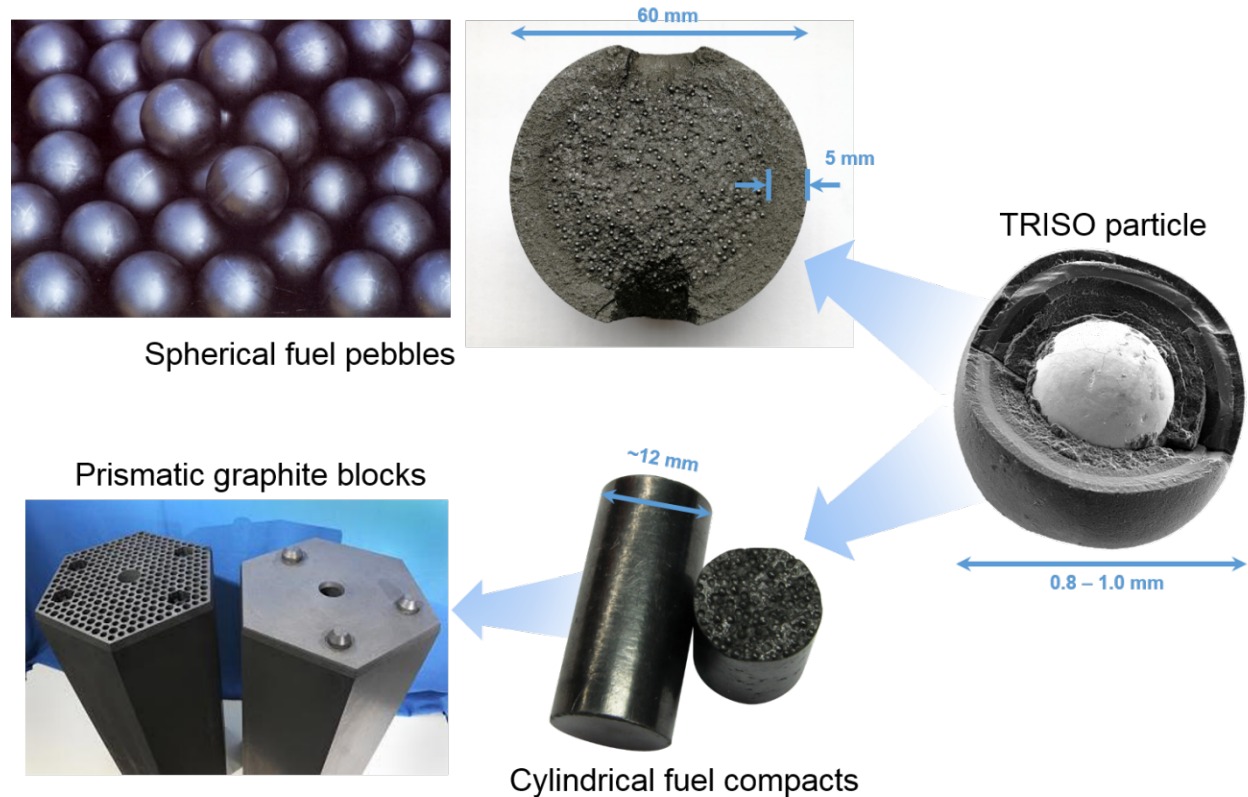
Figure 1. Micrograph of a coated particle with exposed kernel and coating layers [9], examples of spherical (pebble) and cylindrical (compact) fuel forms, and prismatic graphite blocks. Images supplied courtesy of the US DOE, INET, and X Energy, LLC.
