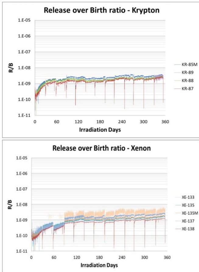
Figure 6. R/B ratio of Kr and Xe isotopes in the HTR-PM fuel irradiation in Petten.
