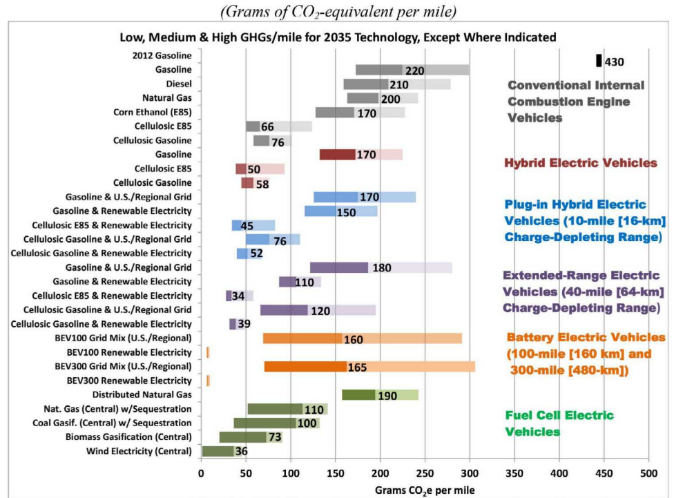
Figure 1. Well-to-Wheels Greenhouse Gases Emissions for 2035 Mid-Size Car. Figure from DOE Program Record Offices of Bioenergy Technologies, Fuel Cell Technologies, and Vehicle Technologies, 5/10/2013. Fuel Cell Electric Vehicles powered by hydrogen from renewable sources have the potential to be one of the cleanest alternative technologies.
