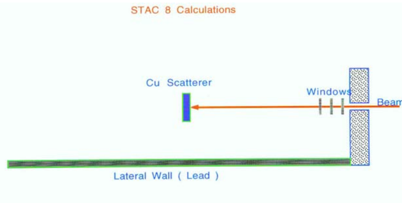
Figure 1 EGS4 and STAC8 Geometry for Bremsstrahlung and Synchrotron Radiation Scattering Calculations
