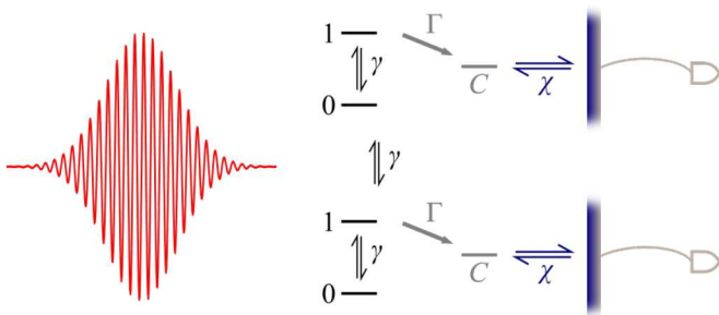
FIG. 5. System comprising two elements described by Fig. 3(b). The elements collectively interact with the field and may exchange population through the field. In systems with more elements, the field couples each element with each other element.
