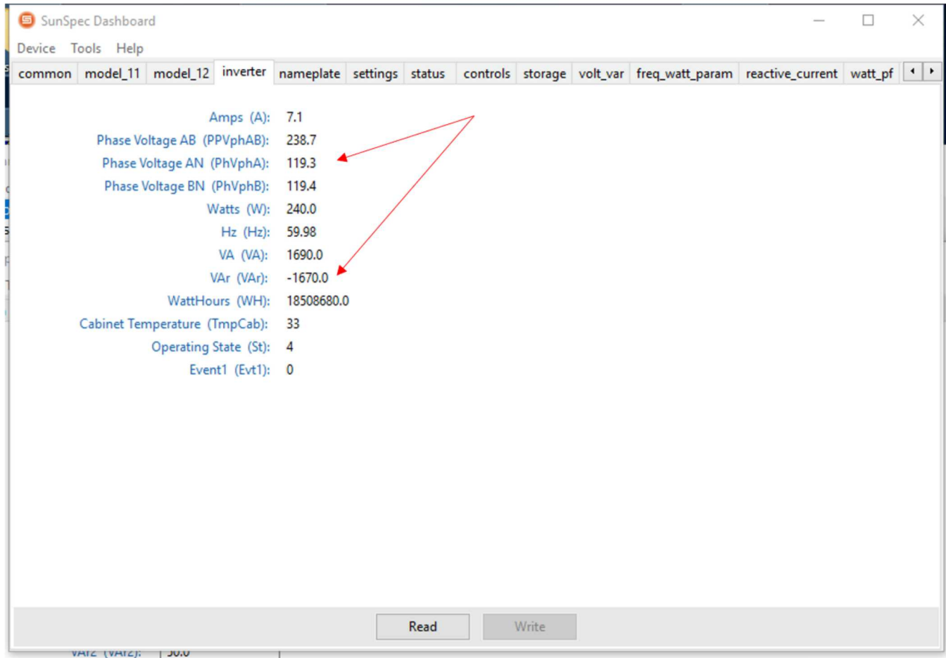
Figure 57: SunSpec Dashboard reading DER with inverted VV curve
