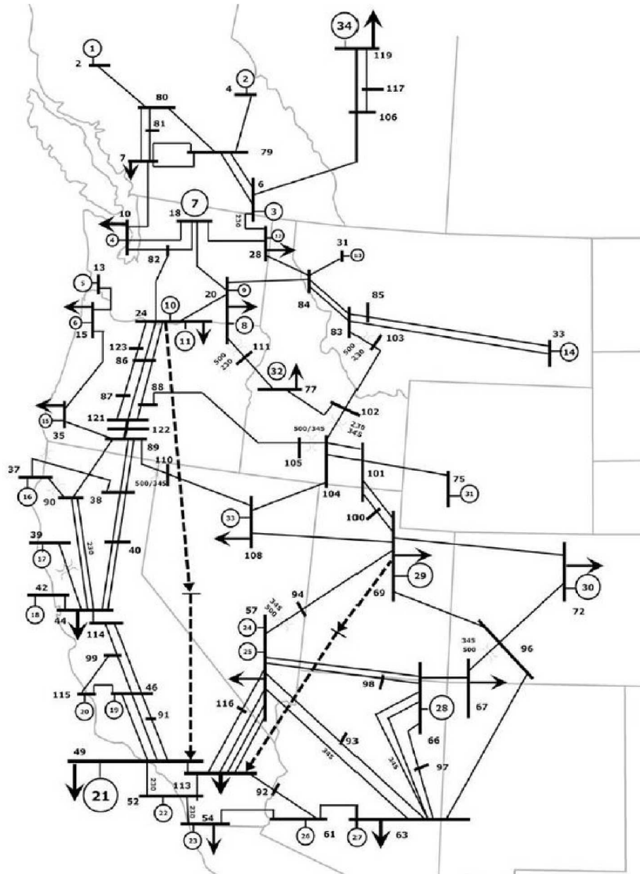
Figure 58: Western North American Power System model used for the power system studies.
