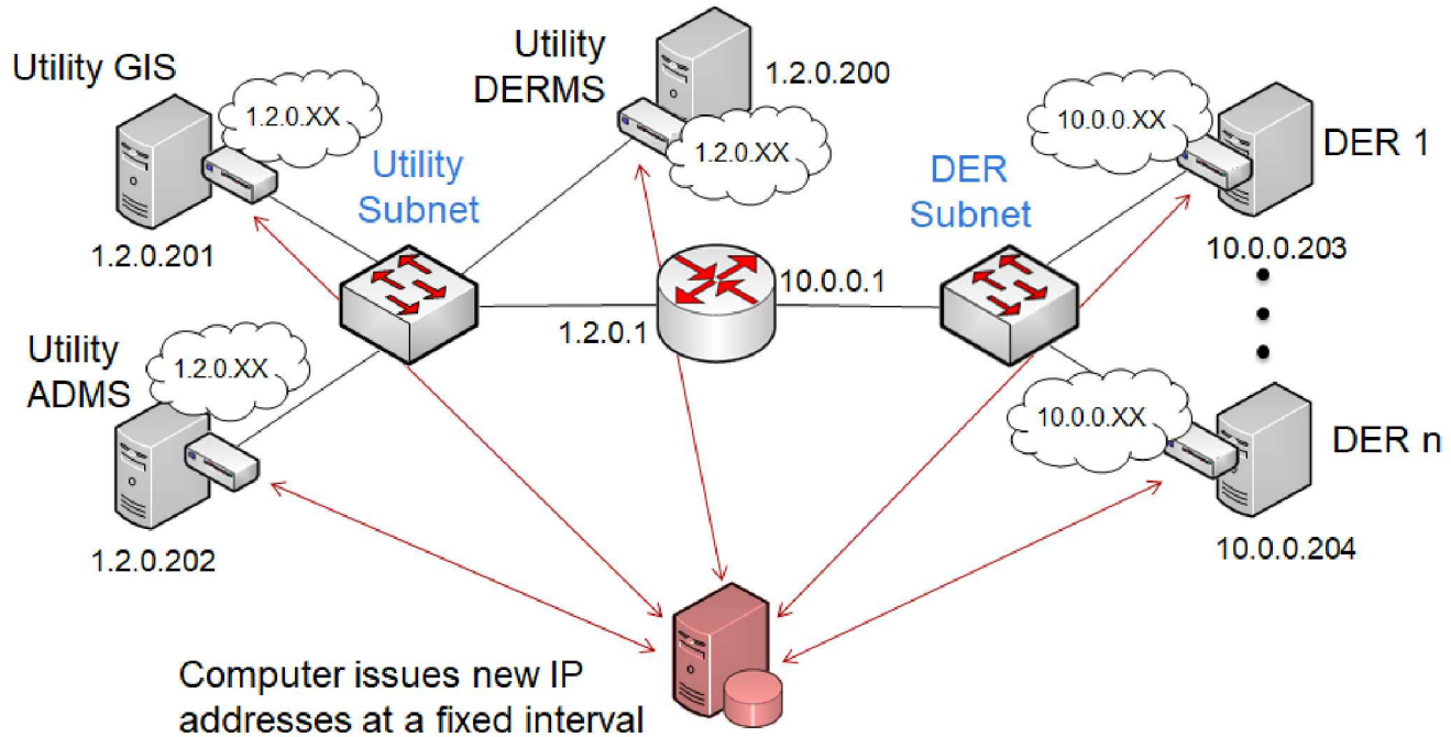
Figure 36: Implementation of Moving Target Defense on a DER communication network.
