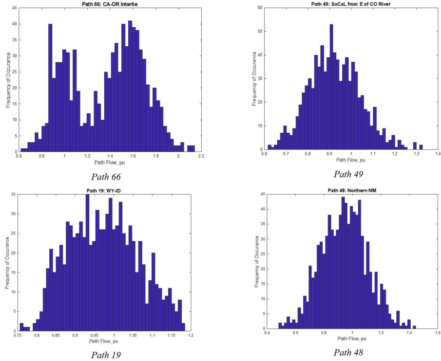
Figure 60: Histograms of select path flows in the WECC when the system dispatch is randomly (uniformly) adjusted within \pm 15\% from its dispatch during peak load conditions.
