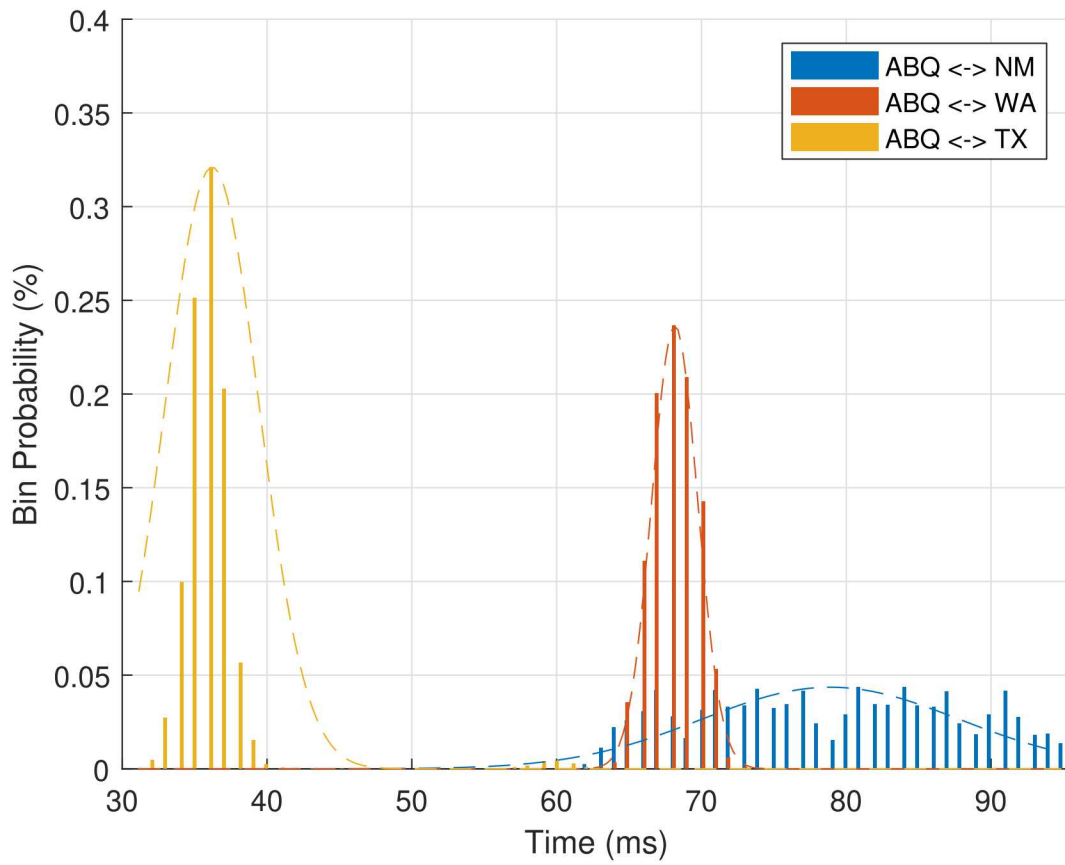
Figure 46: Differences in Communication Time from Geographically Separated Phasor Measurement Units to ABQ
