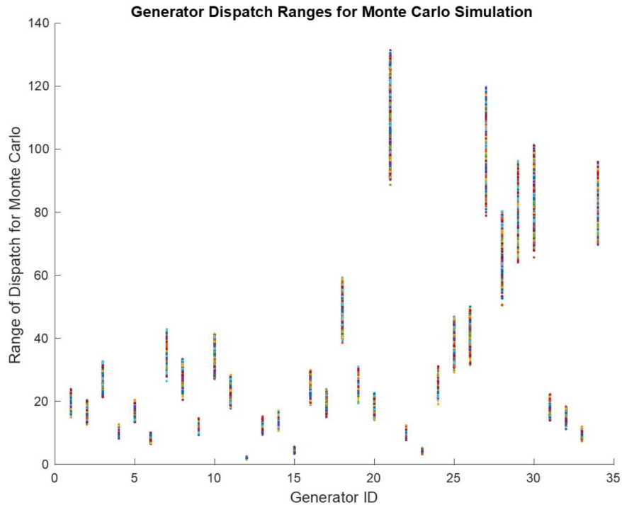
Figure 59: Generator plant dispatch ranges for a case corresponding to generation dispatch of 110.6 GW and max load of 106 GW.
