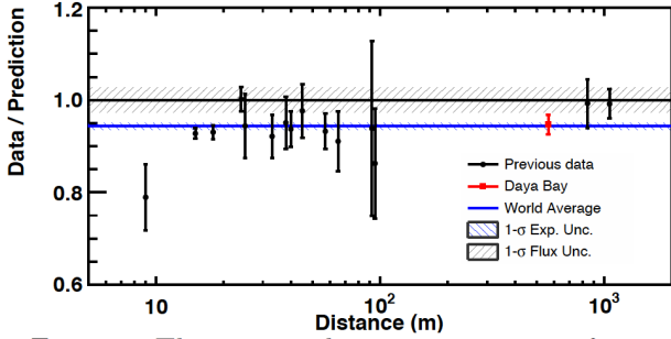
Figure 1: Comparison of previously measured reactor antineutrino fluxes over theoretical predictions with a recent Daya Bay flux measurement (from [6]). Predictions are based on models for the emission of reactor antineutrinos from [1, 2]. The measured deficit relative to prediction is known as the “reactor antineutrino anomaly” [3].
