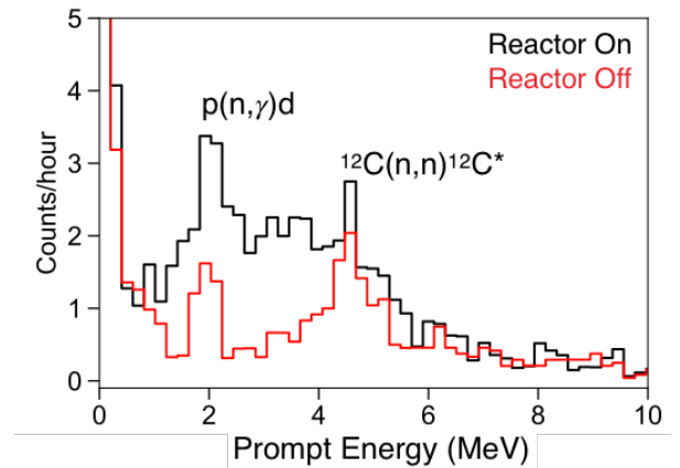
Figure 33: The prompt energy spectra for correlated events with the Reactor On and Reactor Off, for the first 24 hours of data in each case. Both spectra show prominent prompt energy peaks near 2.2 MeV and 4.4 MeV, but the spectra difference between the two data sets has the expected general shape of a reactor antineutrino spectrum.
