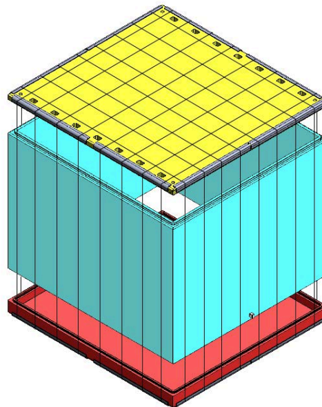
Figure 18: The acrylic containment tank consist of three pieces: a 64 mm thick base (red), four 64 mm thick walls bonded together (aqua), and a 51 mm thick lid (yellow). Sixteen cable loops compress the O-rings between the wall and base. Aluminum angles and Teflon cushions (grey) distribute the force evenly over the acrylic.
