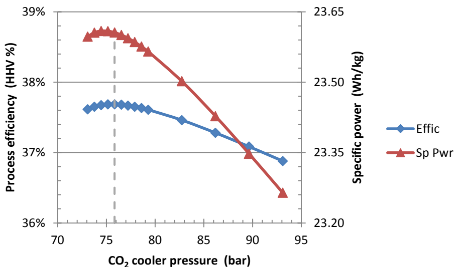
Figure 7 Process efficiency versus CO 2 cooler pressure
