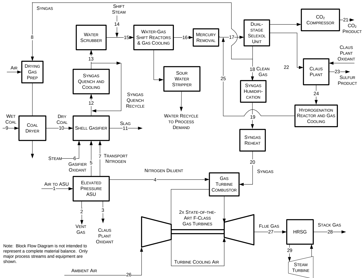
Figure 2 Reference IGCC power plant with carbon capture
