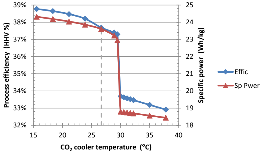
Figure 8 Process efficiency versus CO 2 cooler temperature
