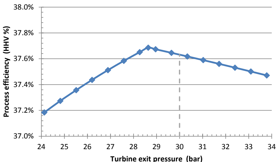
Figure 3 Efficiency versus turbine exit pressure
