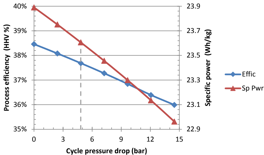
Figure 9 Process efficiency versus cycle pressure drop
