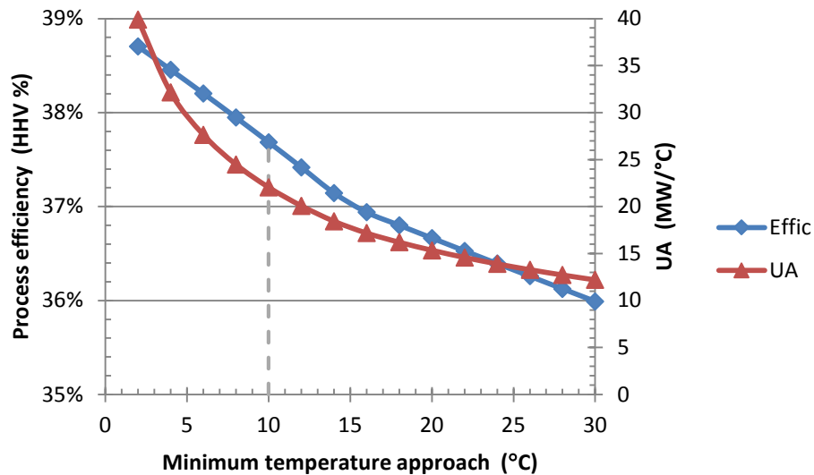
Figure 10 Process efficiency versus minimum approach temperature
