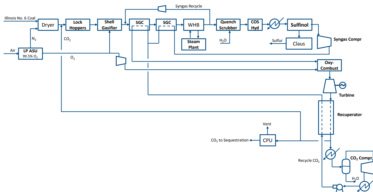
Figure 1 Coal-fired direct-fired sCO 2 power plant
