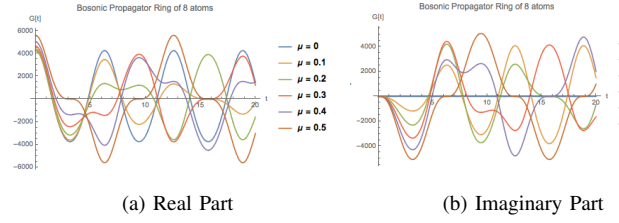
Fig. 12: Real and Imaginary parts of the boson propagator of a carbon nanoring for fixed position x=0 .
