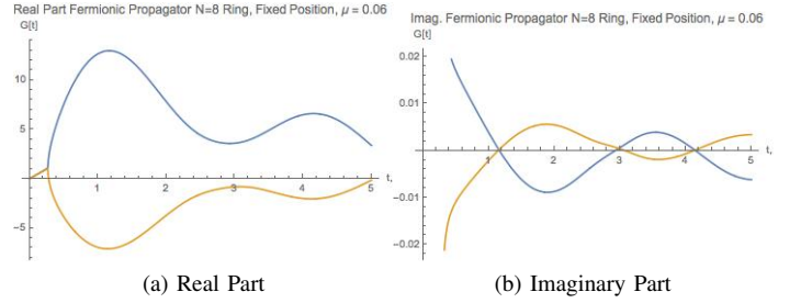
Fig. 13: Real and Imaginary parts of the fermion propagator of a carbon nanoring for fixed position x=0 .
