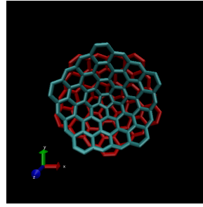
Fig. 9: Two overlaid cones with one cone rotating with respect to the other in the VMD animation environment. View from underneath the cones.
