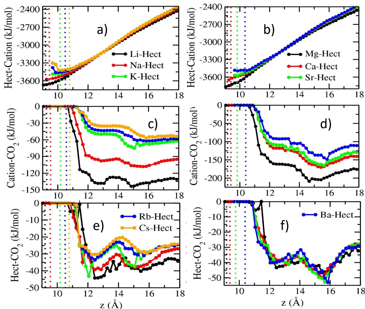
Figure 4. Computed variation in interaction energies between 3 different pairs (a) and b) are Hectorite–Cation (top), c) and d) are Cation–CO 2 (middle), e) and f) are Hectorite–CO 2 (bottom) as functions of interlayer spacing using hectorite with different of mono- and di-valent cations at 323 K and 90 bar. Dotted vertical lines indicate the collapsed interlayer distances for every cations used in our study.
