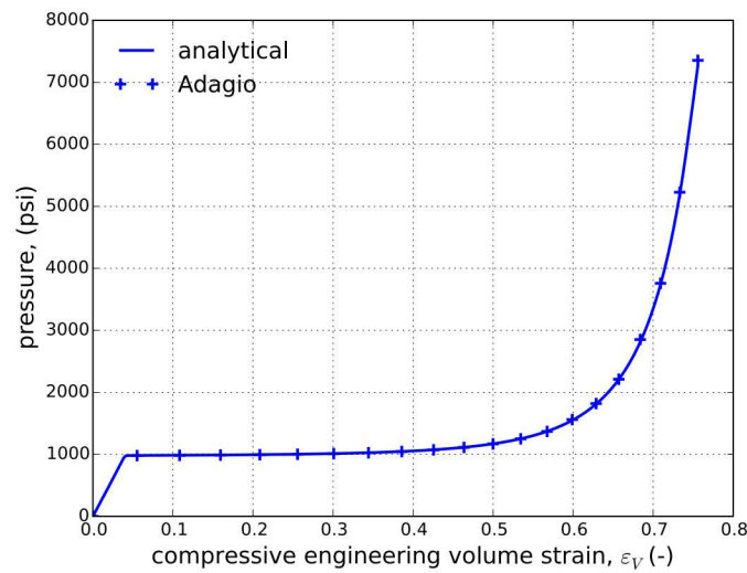
Figure 5.108: Pressure vs. engineering volume strain ( \varepsilon_v ) response of the foam plasticity model through a hydrostatic compression cycle
