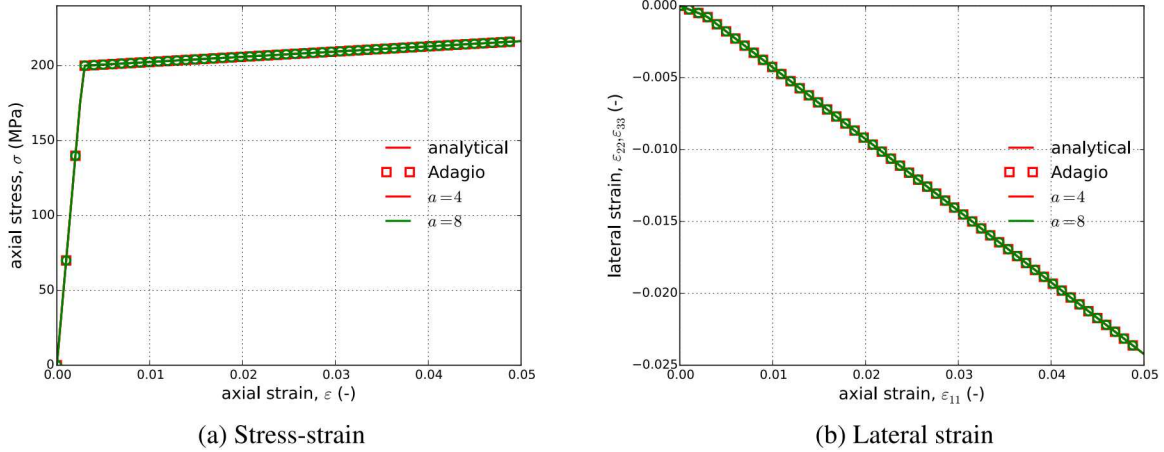
Figure 5.45: (a) Axial stress-strain and (b) lateral strain results of the Hosford plasticity model determined analytically and numerically for the case of yield surface exponents a = 4, 8 .
