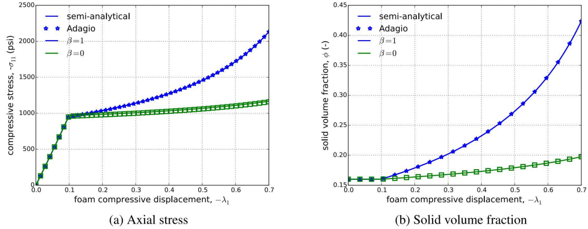
Figure 5.111: (a) Axial stress and (b) maximum solid volume fraction, \phi , evolution obtained as a function of applied compressive displacement and determined via the foam damage model considering both associated ( \beta = 0 ) and radial ( \beta = 1 ) flow assumptions semi-analytically and numerically.
