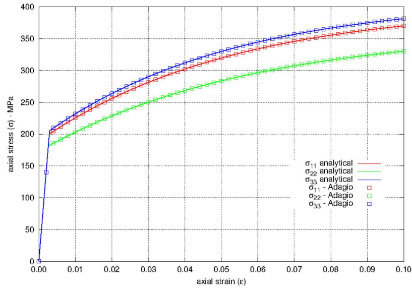
Figure 5.55: Stresses when loading in the e_1 , e_2 , and e_3 -directions using the Hill model with a Voce hardening law.
