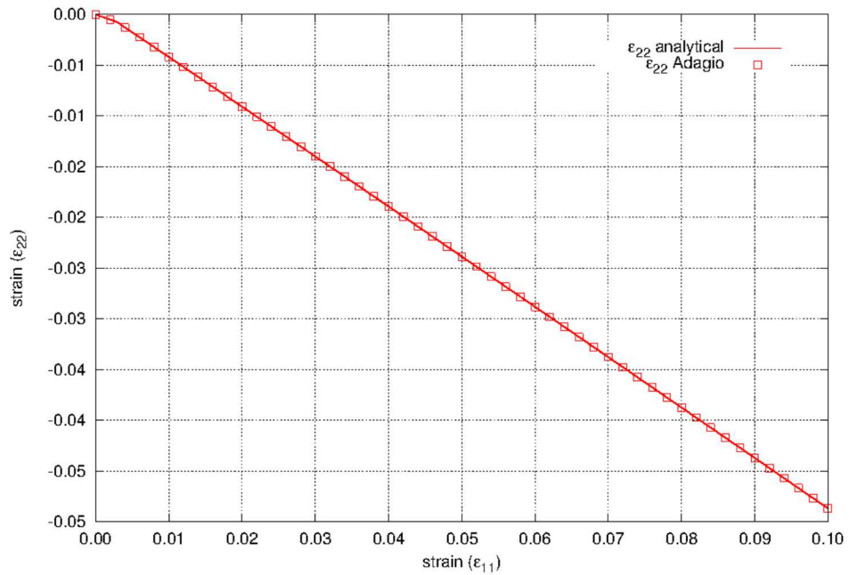
Figure 5.29: The lateral strain as a function of axial strain for the multilinear elastic-plastic model with an analytical Voce law for the hardening model.
