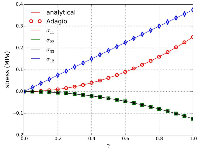
Figure 5.12: Analytical and numerical results for the simple shear case.
