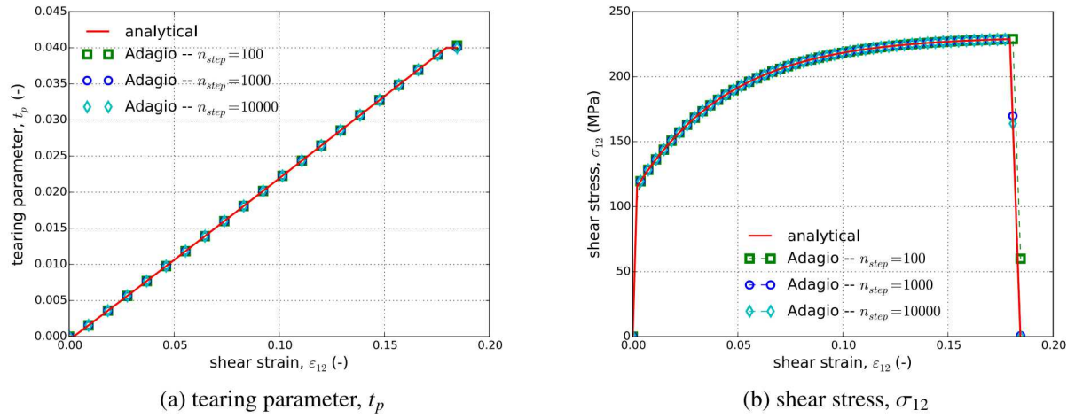
Figure 5.32: Analytical and numerical results of the tearing parameter and shear stress evolution through a pure shear loading path as a function of the shear strain, \varepsilon_{12} .
