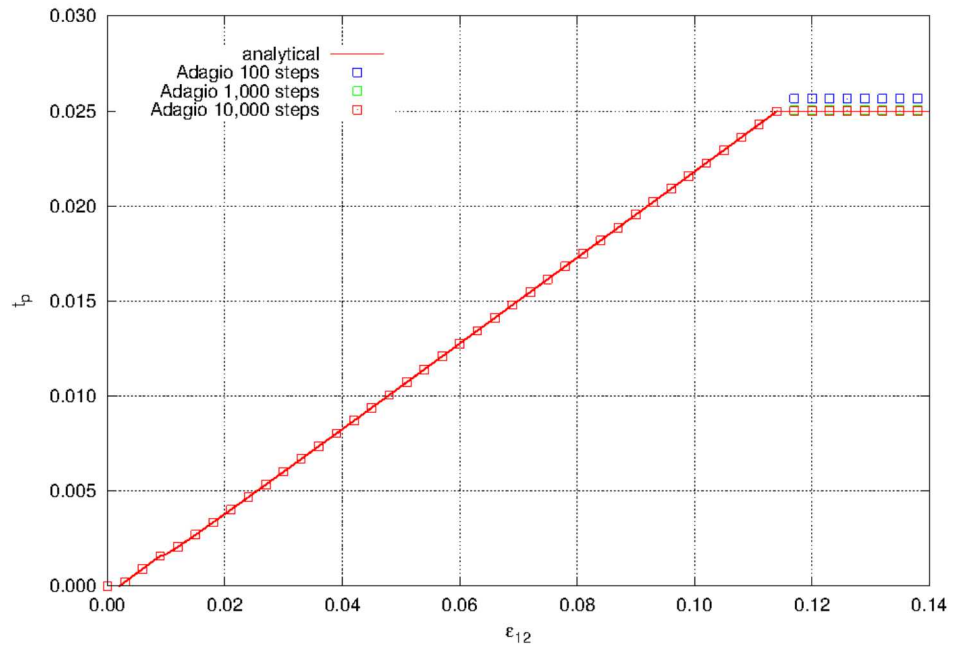
Figure 5.25: The tearing parameter, t_p , in pure shear. The maximum tearing parameter depends on the time discretization or step size.
