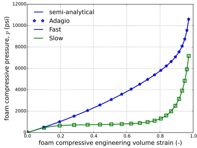
Figure 5.110: Pressure-engineering volume strain results of viscoplastic foam model subjected to a hydrostatic loading at both fast and slow rates determined semi-analytically and numerically.
