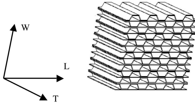
Figure 5.119: Orientation of the T , L and W vectors for 38 pc aluminum honeycomb.
