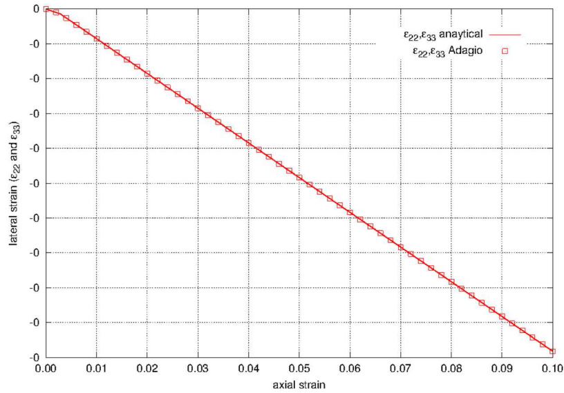
Figure 5.18: Lateral strains for uniaxial stress loading in the x_1 direction for the elastic-plastic model with linear hardening.
