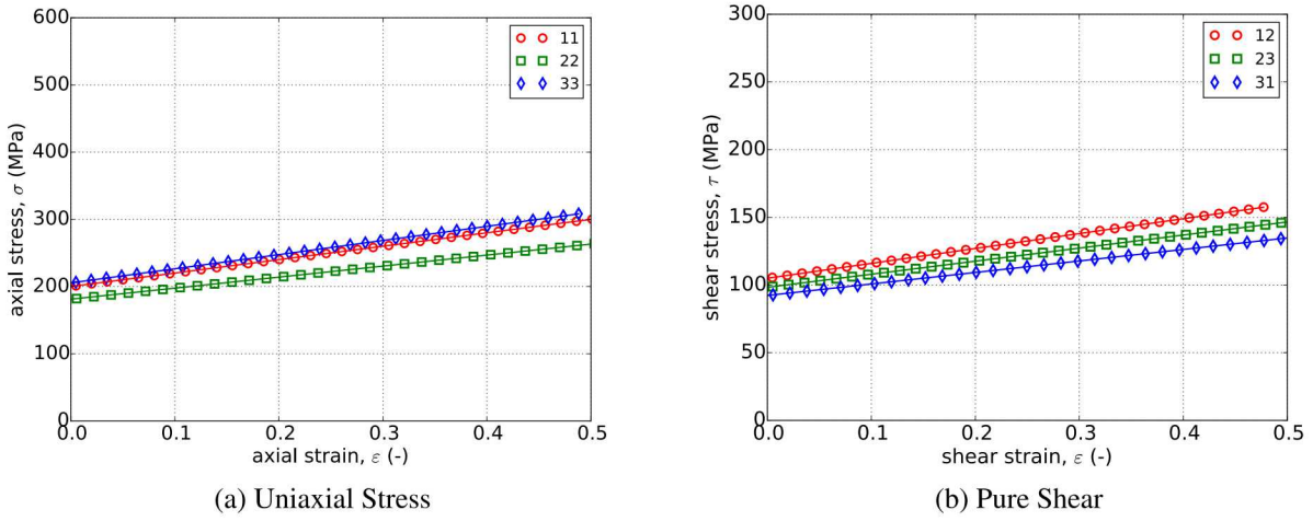
Figure 5.73: Analytical and numerical (a) uniaxial stress-strain and (b) pure shear responses of the Barlat plasticity model with rate-independent, linear hardening. Solid lines are analytical while open symbols are numerical.
