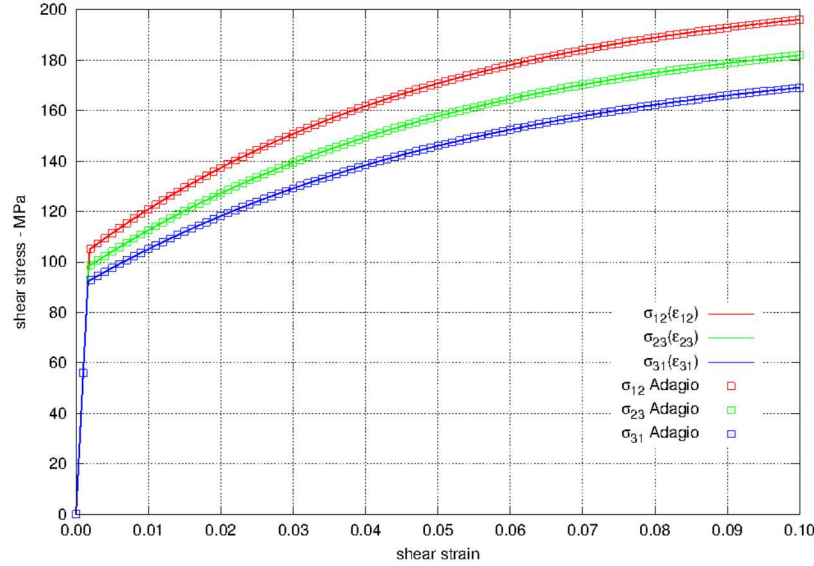
Figure 5.59: Shear stress versus shear strain using the Hill model with a Voce hardening law. Results are for shear in the three orthogonal planes of the material coordinate system.
