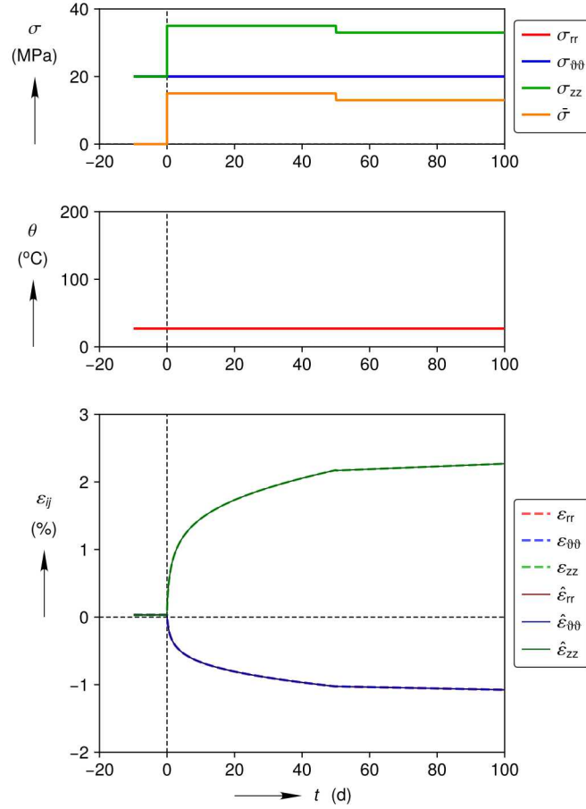
Figure 5.87: Triaxial Compression Verification Test
