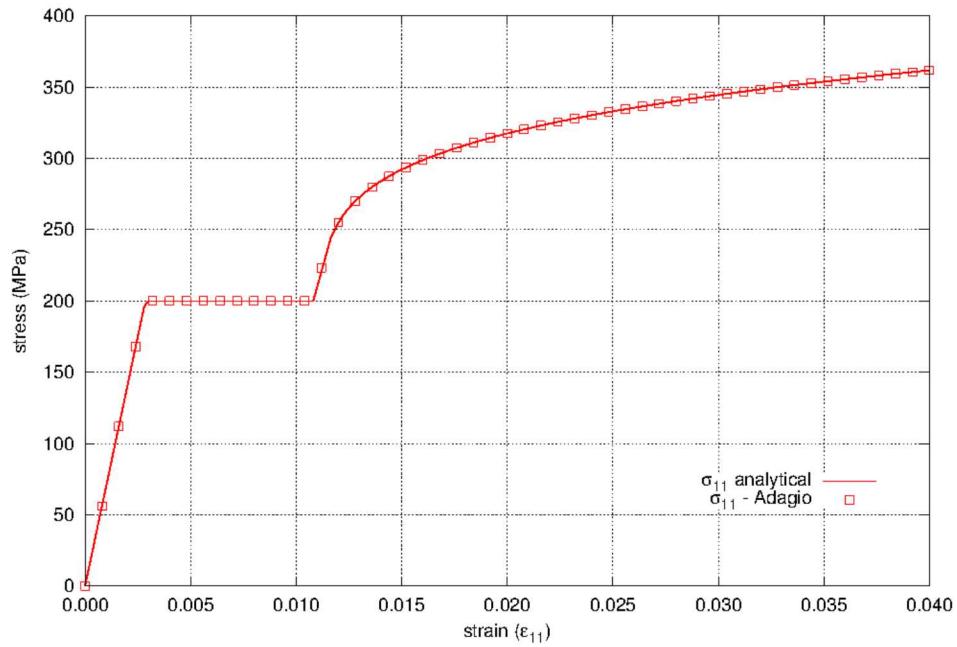
Figure 5.21: The axial stress as a function of axial strain for the elastic-plastic power-law hardening model.
