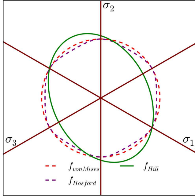
Figure 5.54: Example anisotropic Hill yield surface, f_{Hill}(\sigma_{ij}, \bar{\epsilon}^p = 0) , presented in the deviatoric \pi -plane fit to 2090-T3 aluminum. Comparison von Mises ( J_2 ) and Hosford (with a = 8 ) surfaces are also presented.
