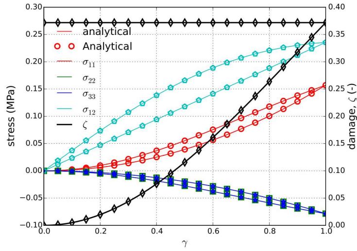
Figure 5.99: Analytical and numerical results of the stress and damage state for the simple shear case.
