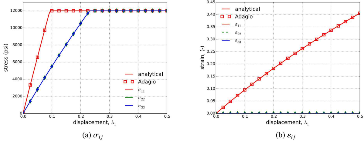
Figure 5.126: Analytical and numerical results of the normal stress and strain components through a tension uniaxial strain loading path as a function of the applied displacement, \lambda_1 .
