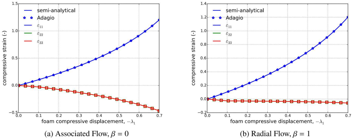
Figure 5.112: Diagon strain evolution through a uniaxial displacement loading of the foam damage model considering (a) associated ( \beta = 0 ) and (b) radial ( \beta = 1 ) flow determined semi-analytically and numerically.
