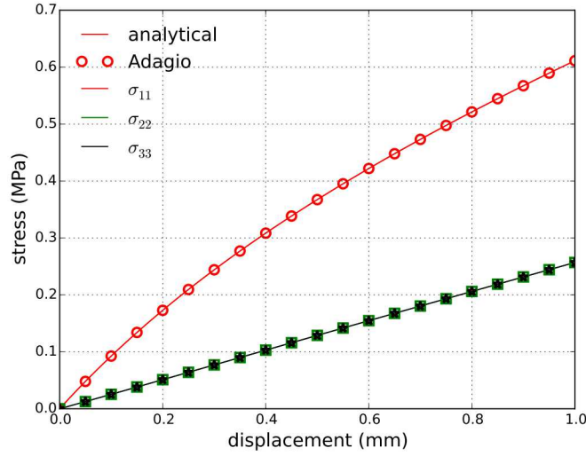
Figure 5.11: Analytical and numerical results for the uniaxial stretch case.
