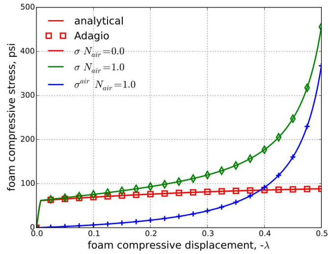
Figure 5.107: Foam stress determined analytically and numerically for both N_{\text{air}} = 0.0 and N_{\text{air}} = 1.0 cases for the low density foam model during displacement controlled hydrostatic compression
