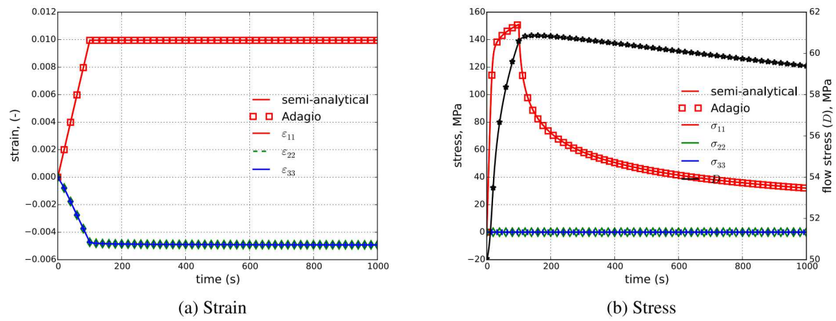
Figure 5.83: Semi-analytical and numerical results of (a) strain and (b) external and internal ( D ) stress evolution during a stress relaxation test with the viscoplastic model.
