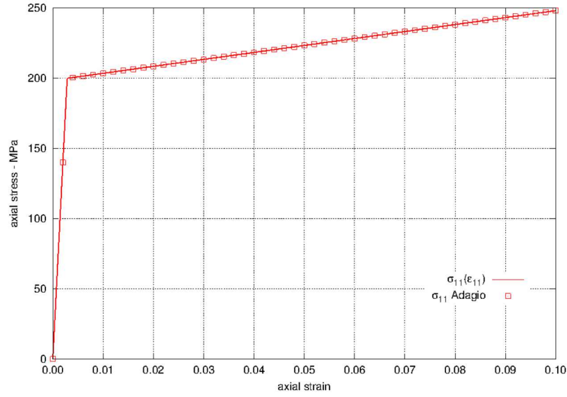
Figure 5.17: Axial stress for loading in the x_1 direction for the elastic-plastic model with linear hardening.
