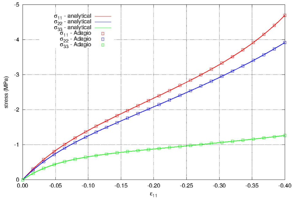
Figure 5.94: The normal stresses for biaxial strain in compression using the hyperfoam model. The results show agreement with the analytical results. The material properties for the model are given in Table 5.31.
