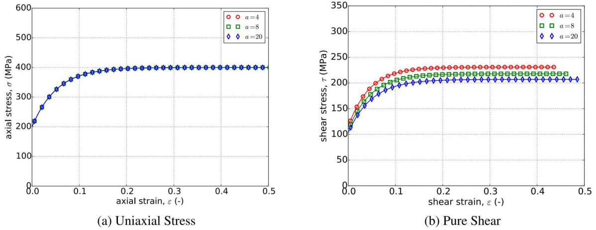
Figure 5.49: Analytical and numerical (a) uniaxial stress-strain and (b) pure shear responses of the Hosford plasticity model with rate-independent, Voce hardening. Solid line are analytical while open symbols are numerical.
