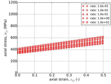
(a) Linear Hardening – 11
