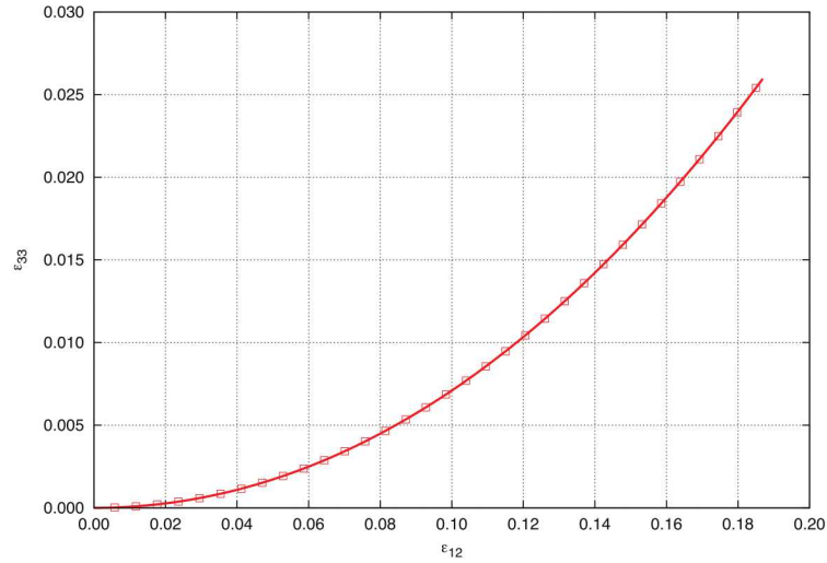
Figure 5.10: Analytical and numerical results for the neo-Hookean model subjected to a pure shear stress. The curve gives the logarithmic strain component, \varepsilon_{33} = \frac{1}{2} \ln B . The solid lines are the analytical results and the boxes are results from Sierra/SM.
