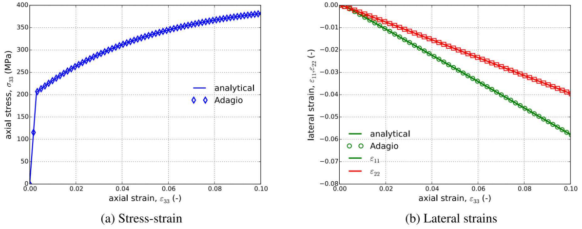
Figure 5.71: Analytical and numerical (a) stress-strain and (b) lateral strain responses of 2090-T3 aluminum with Voce hardening and the Barlat plasticity model. The material is rotated such that the loading is aligned with the “3” direction.
