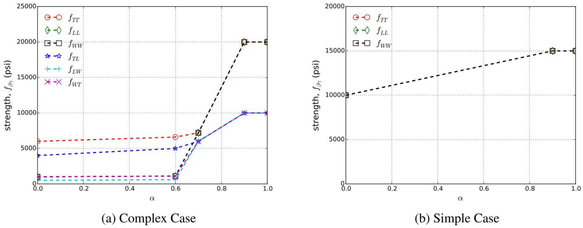
Figure 5.120: Input strength/hardening curves, f_{\beta\gamma} , for use in verification tests of the orthotropic rate model.
