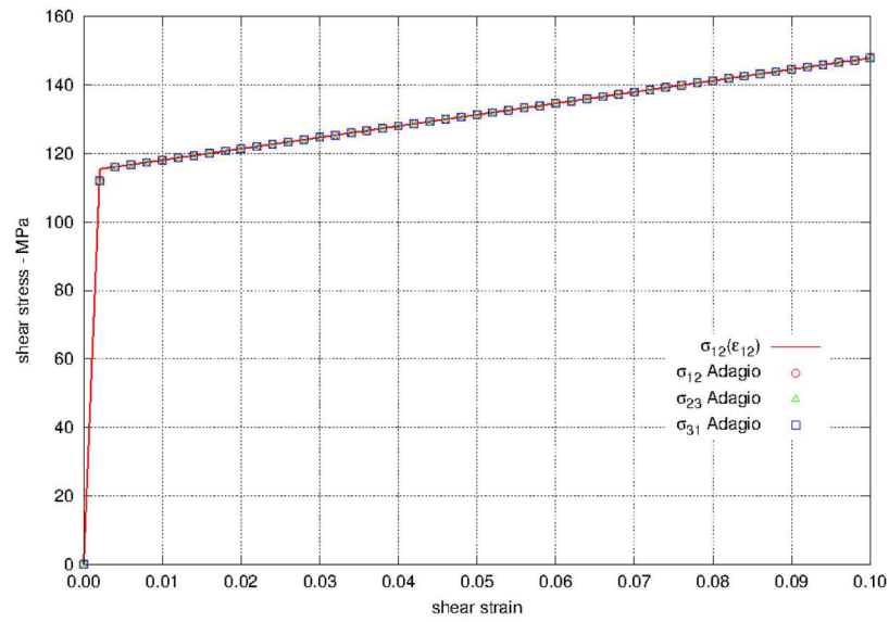
Figure 5.19: Shear stress versus shear strain using the elastic-plastic model. Results are for shear in the x_1 - x_2 plane, x_2 - x_3 plane, and x_3 - x_1 plane.
