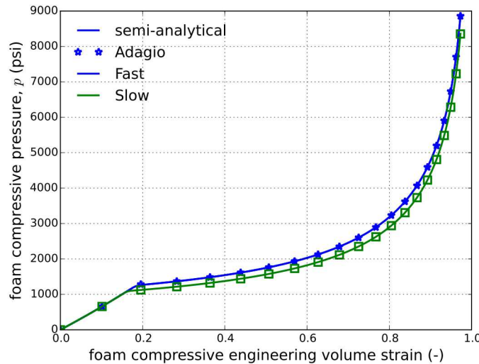
Figure 5.114: Pressure-engineering volume strain results of the foam damage model subjected to a hydrostatic loading at both fast and slow rates determined semi-analytically and numerically.
