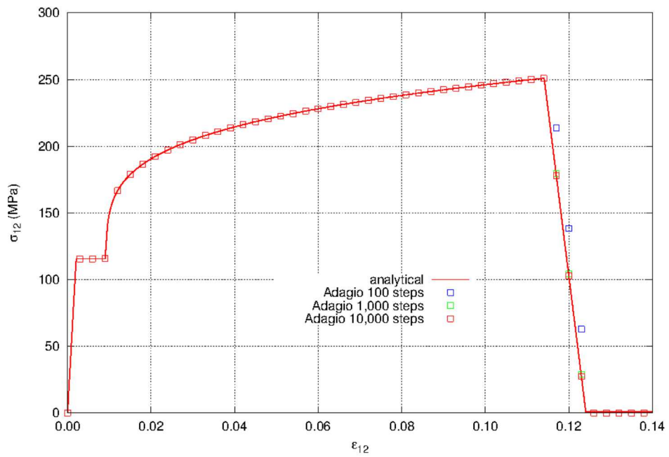
Figure 5.26: Shear stress vs. shear strain for the ductile fracture model in pure shear. The post failure reduction in stress depends on the time discretization or step size.
