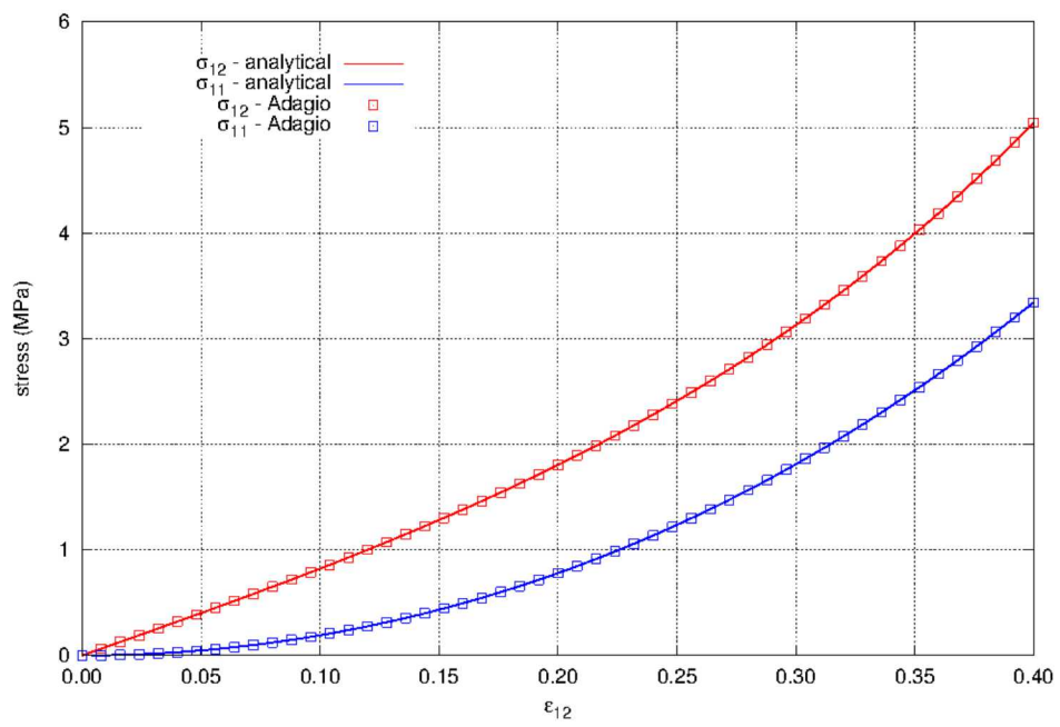
Figure 5.96: The shear and normal stresses for the hyperfoam model in pure shear. The material properties for the model are given in Table 5.31.
