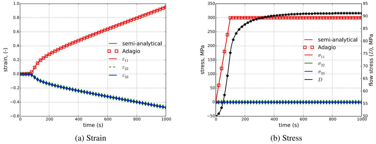
Figure 5.82: Semi-analytical and numerical results of (a) strain and (b) external and internal, ( D ), stress evolution during a creep test with the viscoplastic model.
