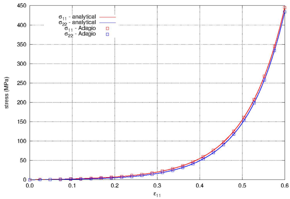
Figure 5.90: The axial and lateral stresses for uniaxial strain in tension using the hyperfoam model. The results show agreement with the analytical results. The material properties for the model are given in Table 5.31.
