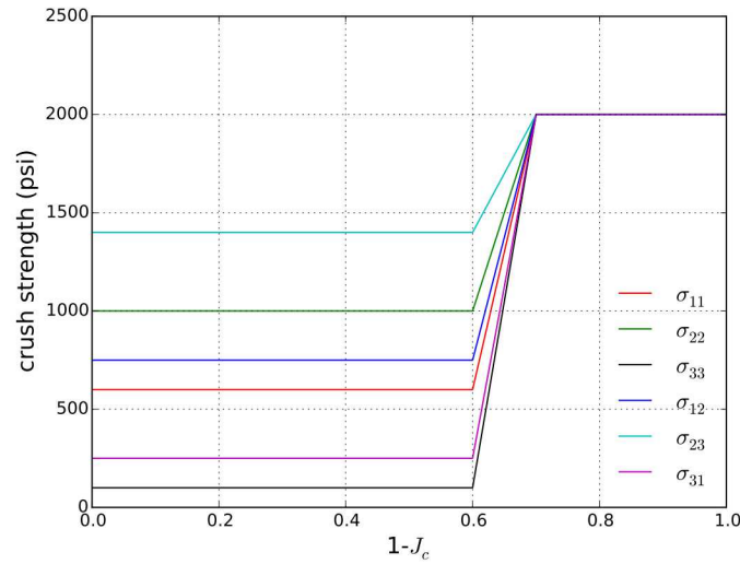
Figure 5.117: Input crush curves used for uniaxial crush analysis.
