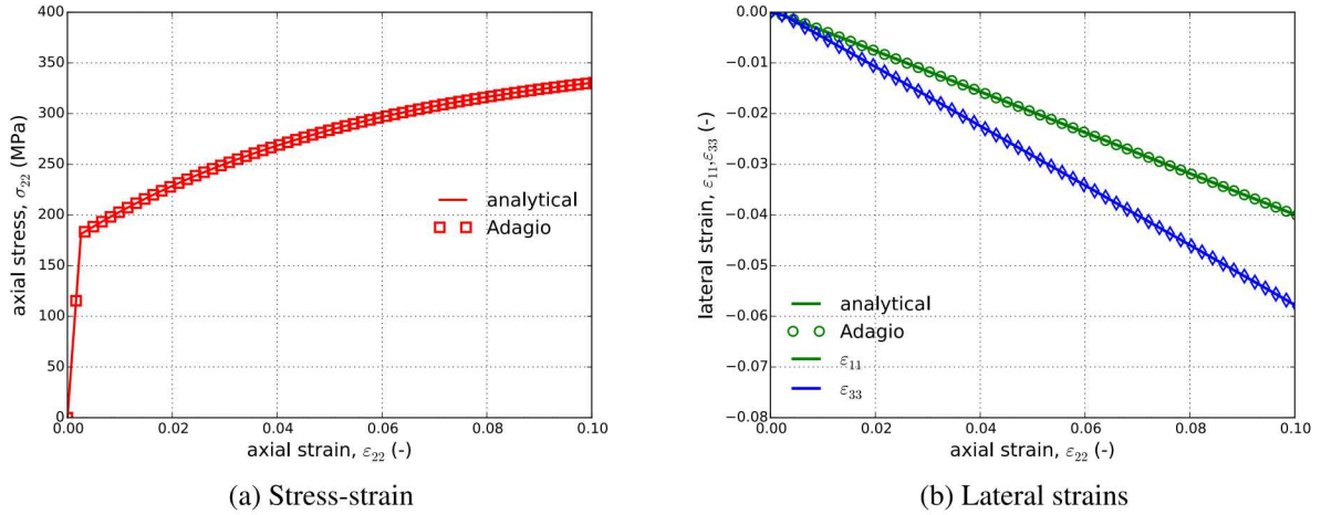
Figure 5.70: Analytical and numerical (a) stress-strain and (b) lateral strain responses of 2090-T3 aluminum with Voce hardening and the Barlat plasticity model. The material is rotated such that the loading is aligned with the “2” direction.
