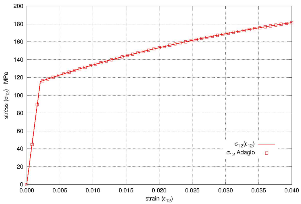
Figure 5.30: The shear stress as a function of shear strain for the multilinear elastic-plastic model with an analytical Voce law for the hardening model.
