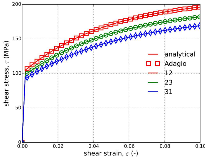
Figure 5.72: Shear stress-strain results for 2090-T3 aluminum determined analytically and numerically by the Barlat plasticity model with Voce Hardening
