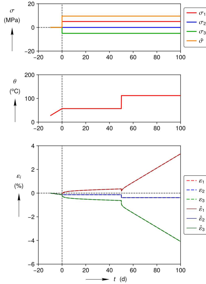
Figure 5.88: Pure Shear Verification Test
