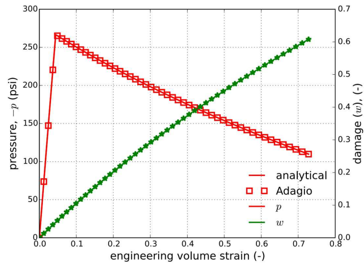
Figure 5.115: Pressure and damage evolutions as function of engineering volume strain results of the foam damage model subject to a tensile hydrostatic loading determined analytically and numerically. Note, conventionally with this model pressure is defined positive in compression.
