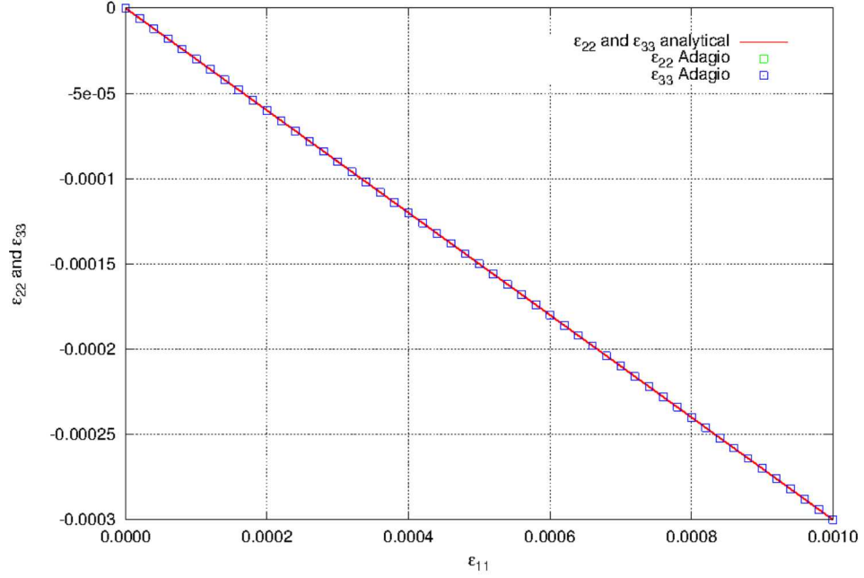
Figure 5.2: The lateral strain components \varepsilon_{22} and \varepsilon_{33} in uniaxial stress using the elastic model.
