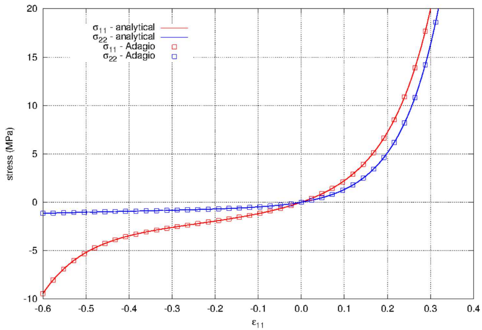
Figure 5.92: The axial and lateral stresses for uniaxial strain in both tension and compression using the hyperfoam model. The results show agreement with the analytical results and that the response of the material is very different in tension and compression. The material properties for the model are given in Table 5.31.
