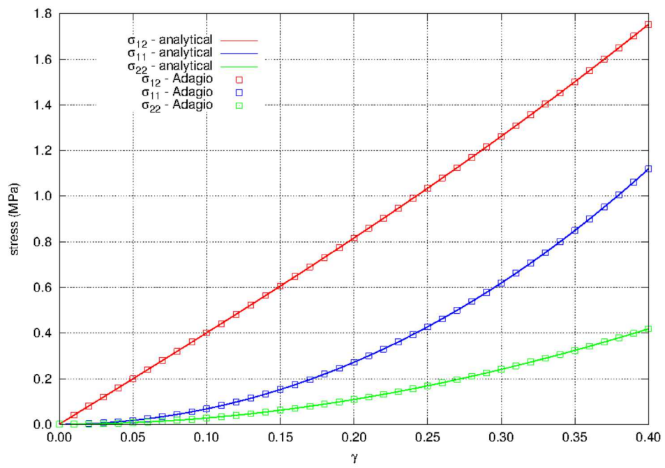
Figure 5.97: The shear and normal stresses for the hyperfoam model in simple shear. The material properties for the model are given in Table 5.31.
