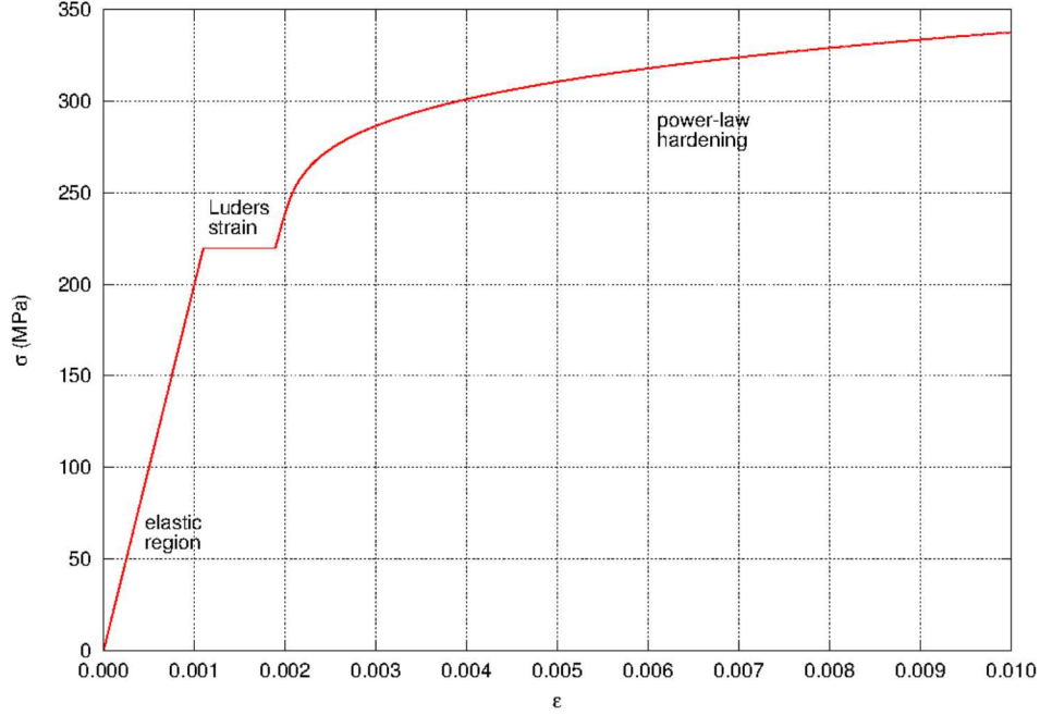
Figure 5.20: Typical stress-strain response for the power-law hardening model.
