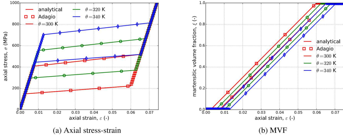
Figure 5.103: (a) Axial stress-strain response and (b) martensitic volume fraction, \xi , evolution determined analytically and via adagio for three different ambient temperatures \theta = 300, 320 and 340 K.
