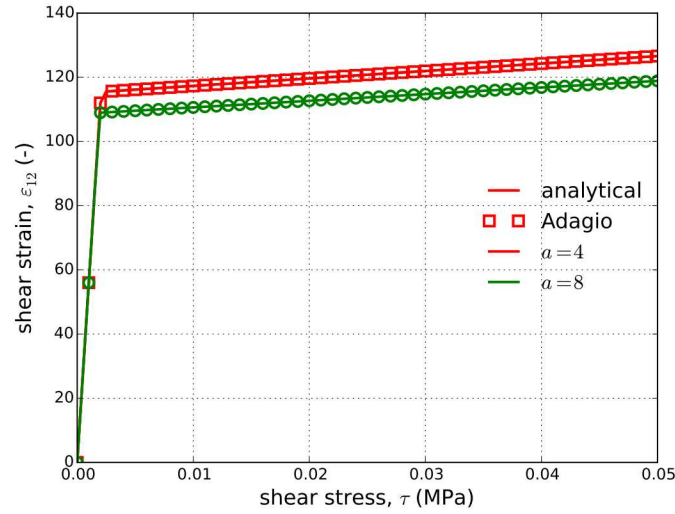
Figure 5.46: Shear stress-strain results of the Hosford plasticity model determined analytically and numerically for the case of yield surface exponents a = 4, 8 .
