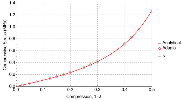
Figure 5.15: Stress determined analytically and numerically for the Gent model during displacement controlled hydrostatic compression.
