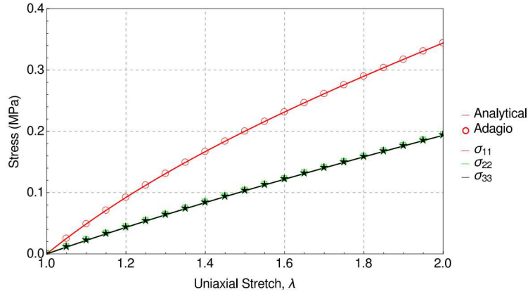
Figure 5.13: Analytical and numerical results for the uniaxial stretch case.
