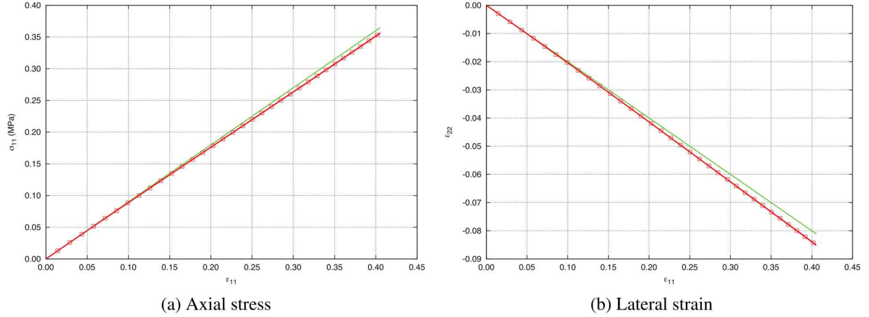
Figure 5.8: Analytical and numerical results for the (a) uniaxial stress and (b) lateral strain. The green line gives the linear elastic response.
