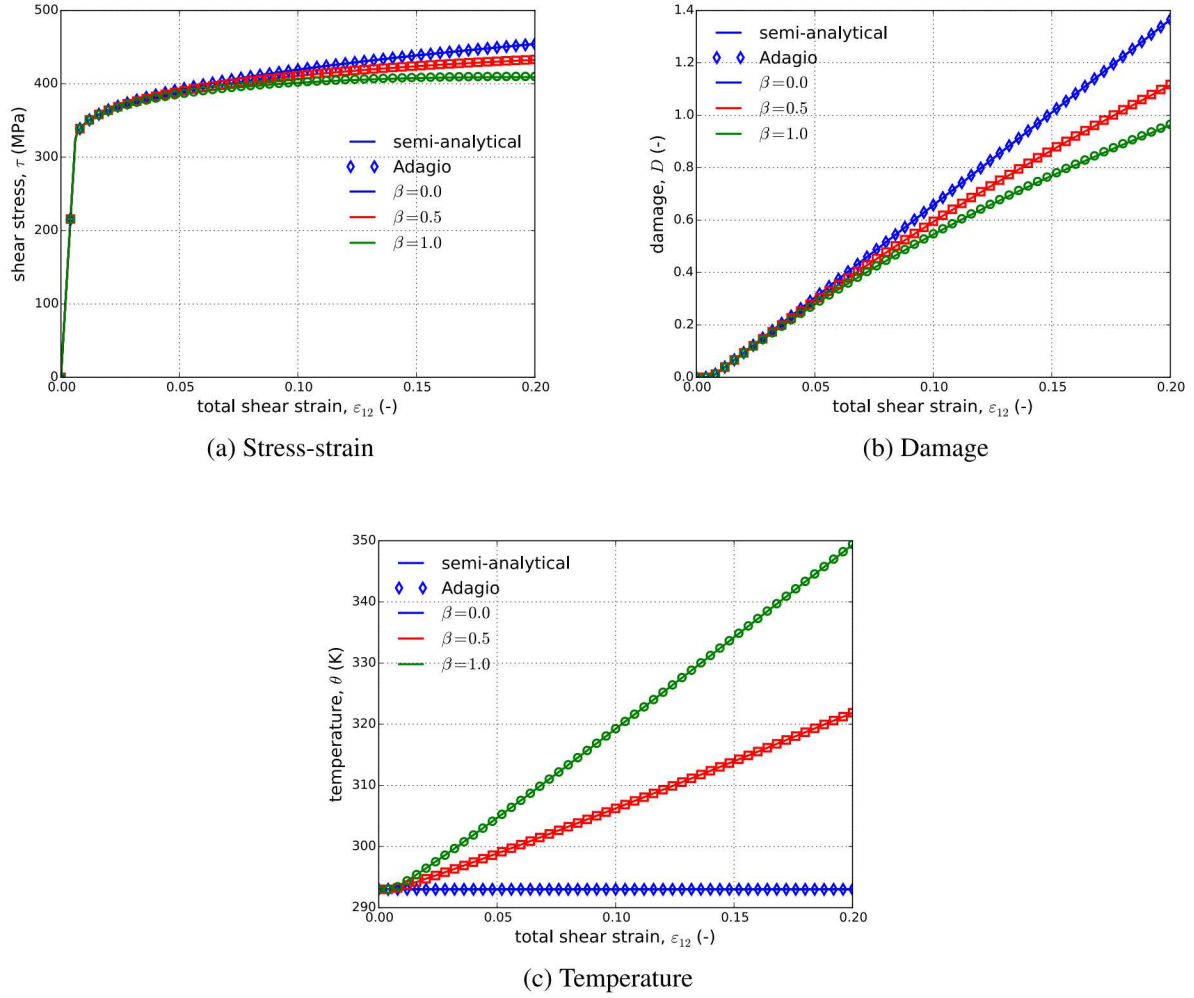
Figure 5.36: Semi-analytical and numerical (a) stress-strain (b) damage and (c) temperature evolutions of the Johnson-Cook model subjected to a pure shear loading with three different plastic work conversion ratios, \beta . The strain rate for all three cases is \dot{\epsilon} = 1\text{s}^{-1} .
