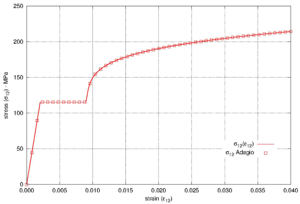
Figure 5.23: The shear stress as a function of shear strain for the elastic-plastic power-law hardening model.
