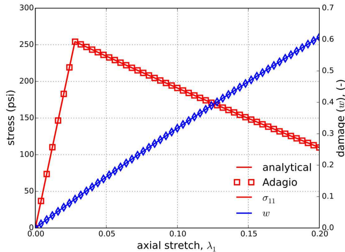
Figure 5.113: Response of the foam damage model through a uniaxial stress, displacement controlled tension simulation. Stress in the loading direction, \sigma_{11} , and damage measure, w , against the applied displacement, \lambda_1 , are shown.
