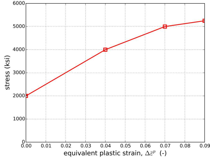
Figure 5.27: An example of a multilinear elastic-plastic stress-strain curve.
