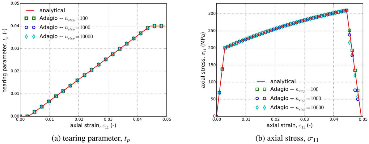
Figure 5.31: Analytical and numerical results of the tearing parameter and axial stress evolution through a uniaxial tension loading path as a function of the axial strain, \varepsilon_{11} .
