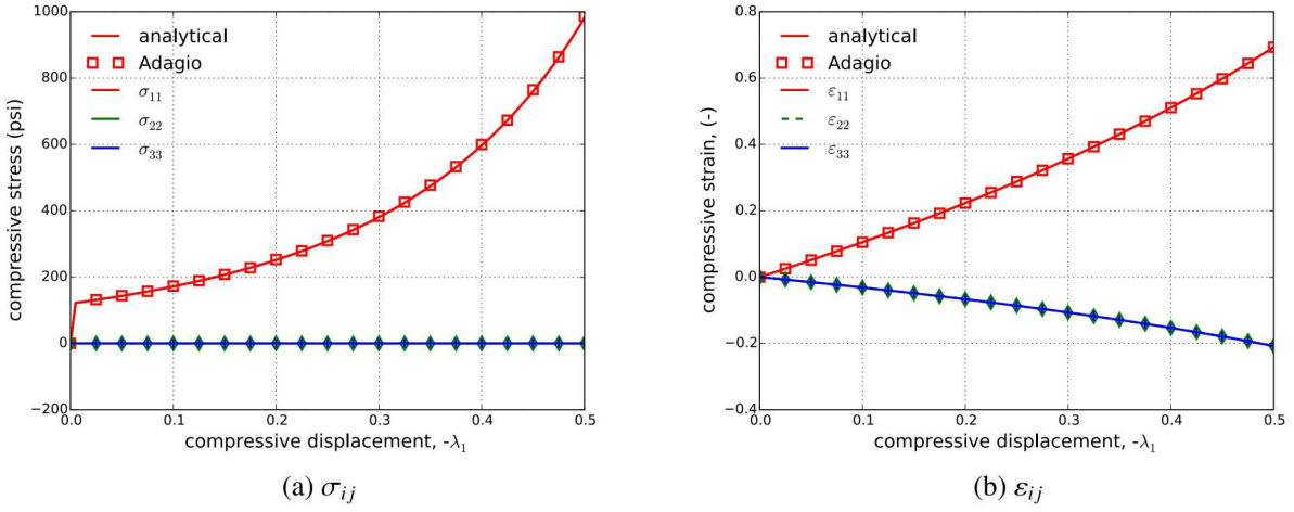
Figure 5.125: Analytical and numerical results of the normal stress and strain components through a compressive uniaxial stress loading path as a function of the applied displacement, \lambda_1 .
