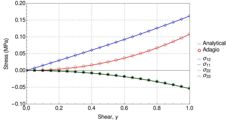
Figure 5.14: Analytical and numerical results for the simple shear case.
