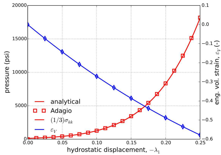
Figure 5.127: Analytical and numerical pressure-volume strain response of the wire mesh model through a hydrostatic compression loading as a function of the applied displacement, \lambda_1 .
