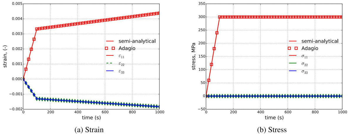
Figure 5.80: Semi-analytical and numerical results of (a) strain and (b) stress evolution during a creep test.
