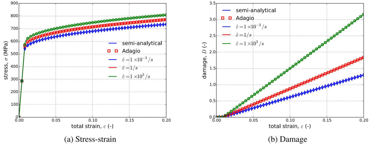
Figure 5.33: Semi-analytical and numerical (a) stress-strain and (b) damage evolutions of the Johnson-Cook model subjected to a uniaxial loading at three different applied strain rates. In these results, \beta = 0 such that heat associated with plastic work is allowed to transfer to the environment.
