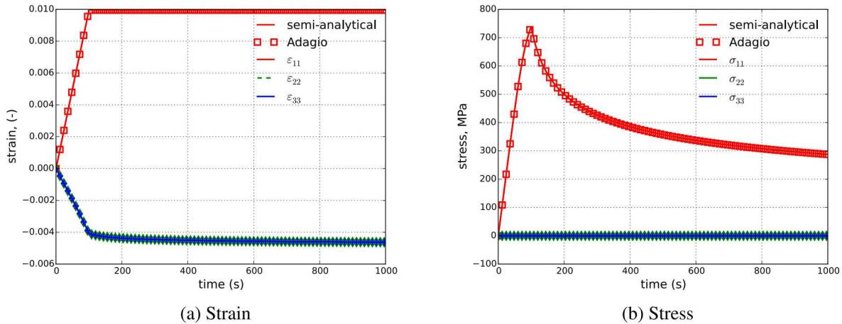
Figure 5.81: Semi-analytical and numerical results of the (a) strain and (b) stress evolution during a stress relaxation test.
