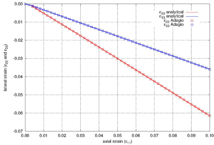
Figure 5.56: Lateral strain as a function of axial strain for the Hill model of 2090-T3 aluminum. Loading is in the e_1 -direction and the hardening law is a Voce law.
