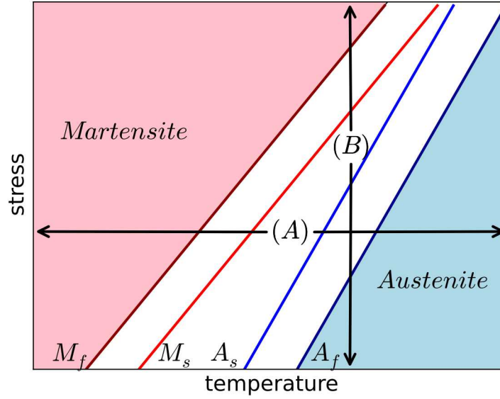
Figure 5.102: Representative phase diagram of shape memory alloys highlighting characteristic loading paths ((A) and (B)), transformation surfaces, and phases.
