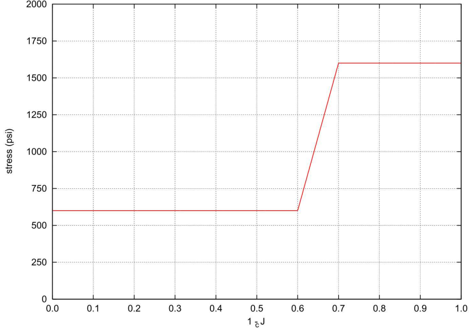
Figure 5.116: An example of an input crush curve for an aluminum honeycomb.
