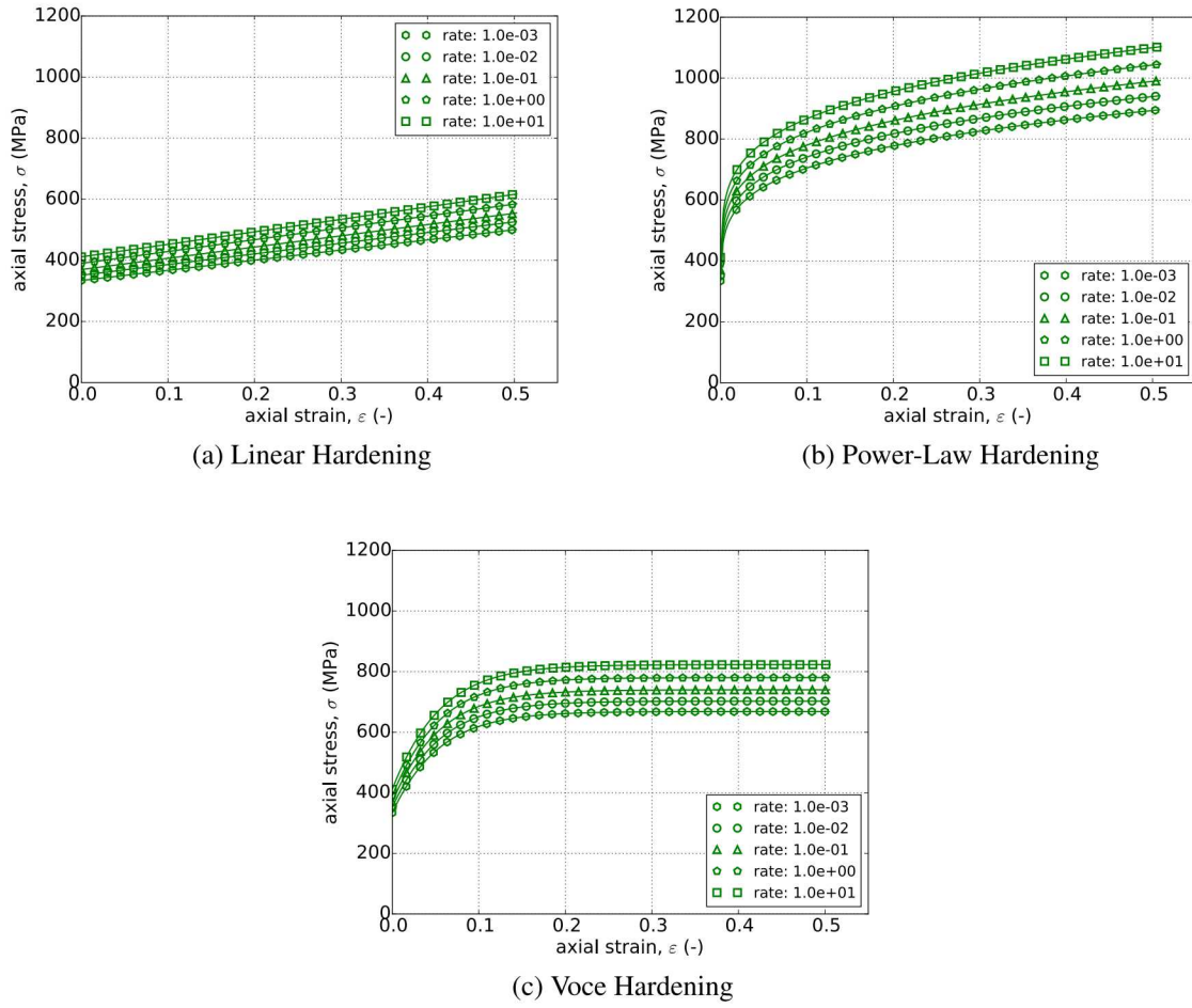
Figure 5.52: Analytical and numerical uniaxial stress-strain response of the Hosford plasticity model ( a = 8 ) with rate-dependent, power-law breakdown type hardening with (a) linear (b) power-law and (c) Voce rate-independent hardening. Solid lines are analytical results while open symbols are numerical.
