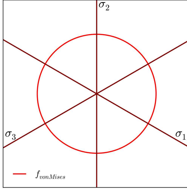
Figure 5.16: Example von Mises yield surface ( J_2 ) used by the elastic-plastic model presented in the deviatoric \pi -plane. In this case the surface is plotted for \alpha_{ij} = 0 and \bar{\epsilon}^p = 0 .
