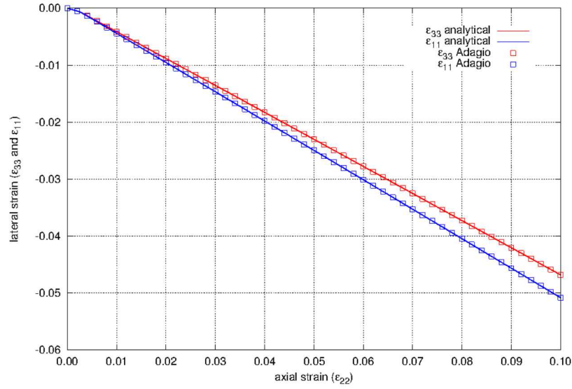
Figure 5.57: Lateral strain as a function of axial strain for the Hill model of 2090-T3 aluminum. Loading is in the e_2 -direction and the hardening law is a Voce law.
