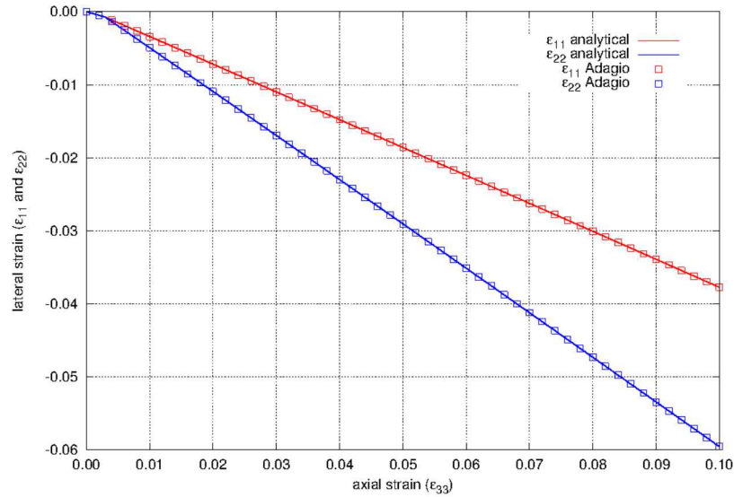
Figure 5.58: Lateral strain as a function of axial strain for the Hill model of 2090-T3 aluminum. Loading is in the e_3 -direction and the hardening law is a Voce law.
