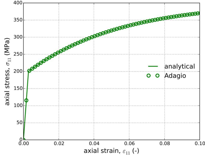
Figure 5.68: Axial stress-strain response determined analytically and numerically for 2090-T3 aluminum using the Barlat plasticity model with Voce hardening.
