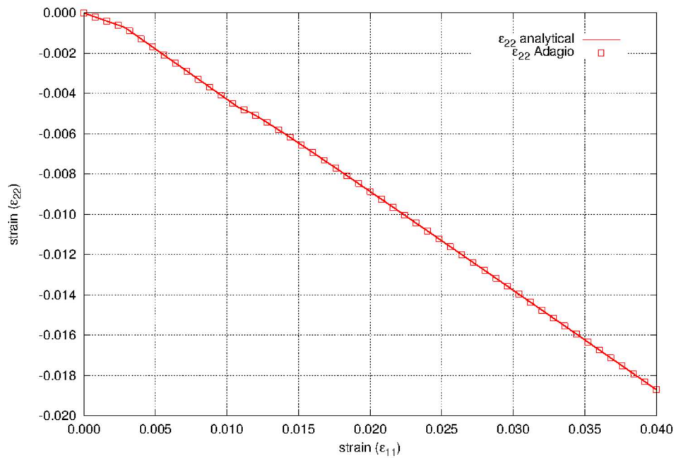
Figure 5.22: The lateral strain as a function of axial strain for the elastic-plastic power-law hardening model.
