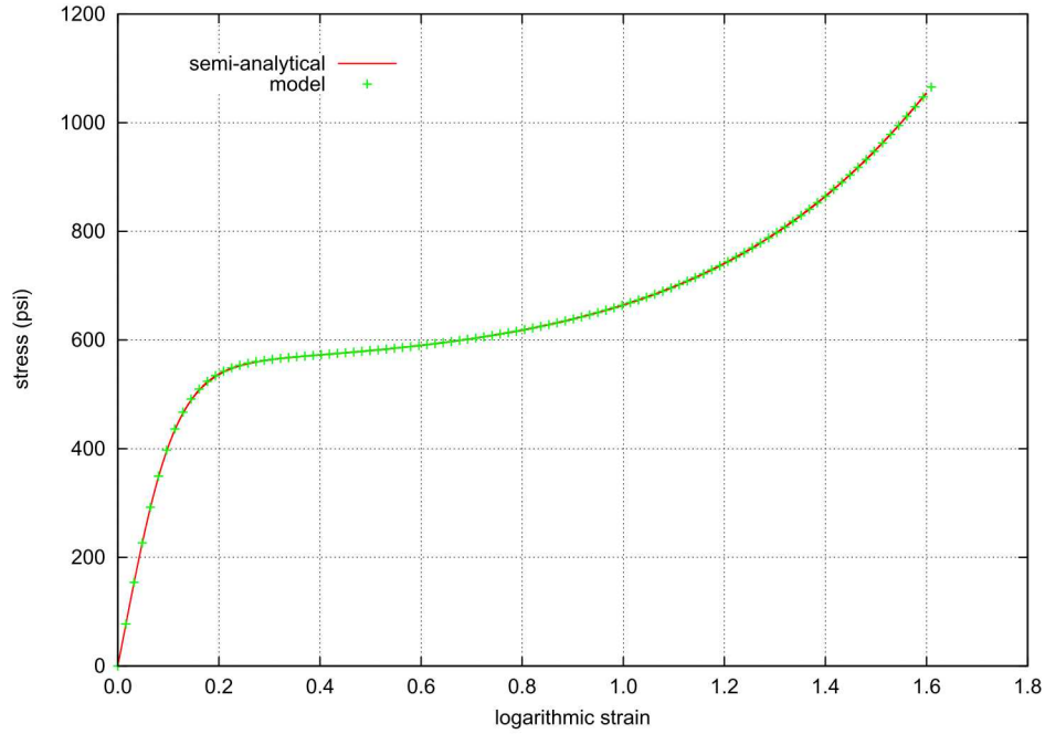
Figure 5.109: Verification of the viscoplastic foam model in uniaxial compression showing the axial stress as a function of the logarithmic strain.
