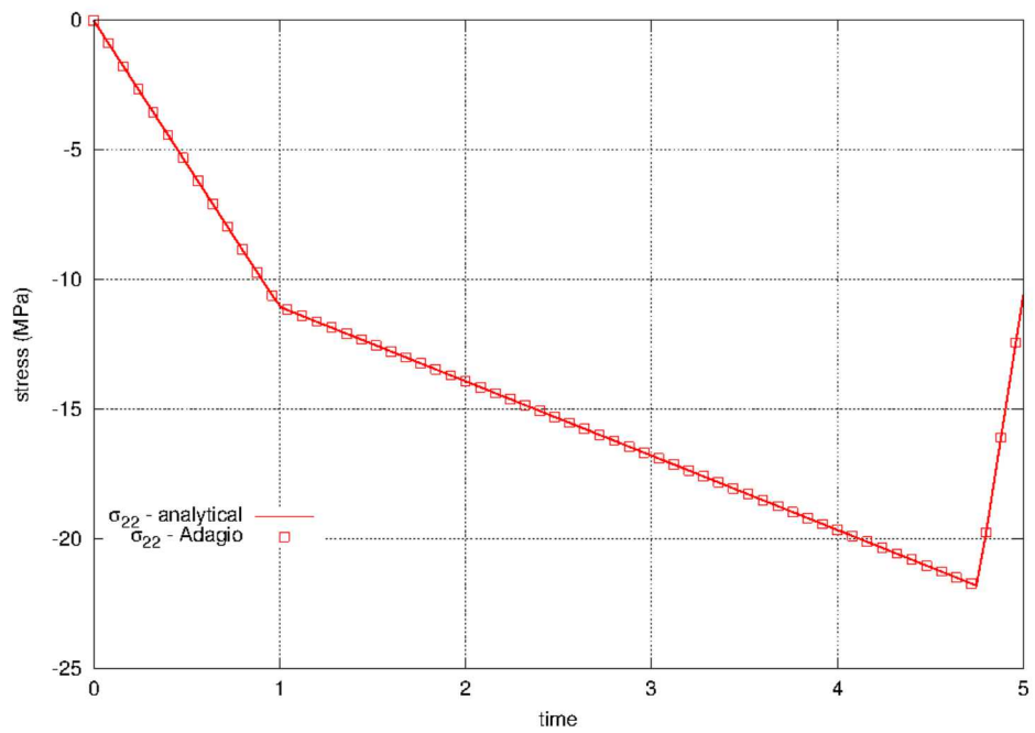
Figure 5.101: Axial stress, \sigma_{22} , over the course of the prescribed triaxial loading path.
