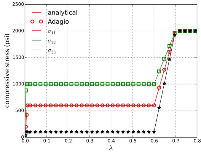
Figure 5.118: Analytical and numerical results for uniaxial crush cases.
