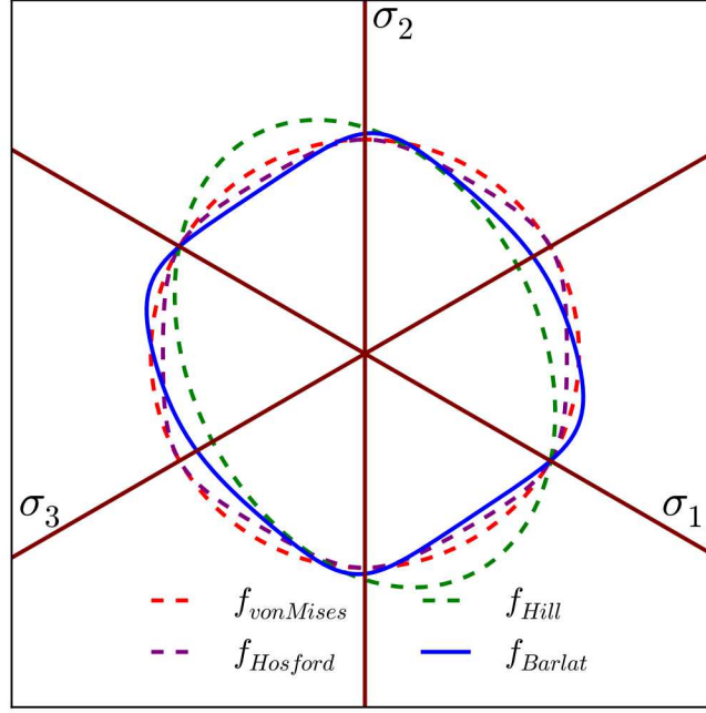
Figure 5.67: Example Barlat yield surface, f_{Barlat}(\sigma_{ij}, \bar{\epsilon}^p = 0) , of 2090-T3 aluminum presented in the deviatoric \pi -plane. Comparison von Mises ( J_2 ), Hosford (with a = 8 ), and Hill surfaces are also presented for comparison.
