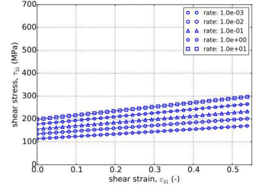
(c) Linear Hardening – 31
