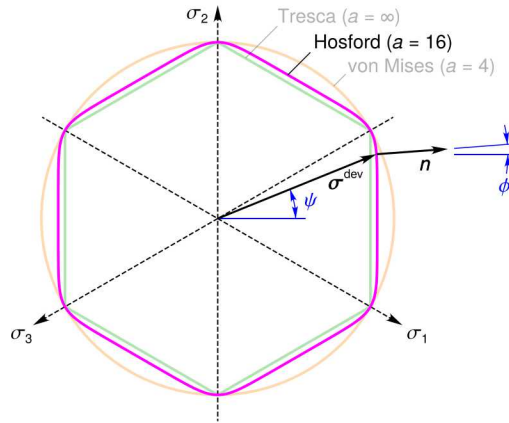
Figure 5.84: Hosford equivalent stress surface in the \pi -plane.
