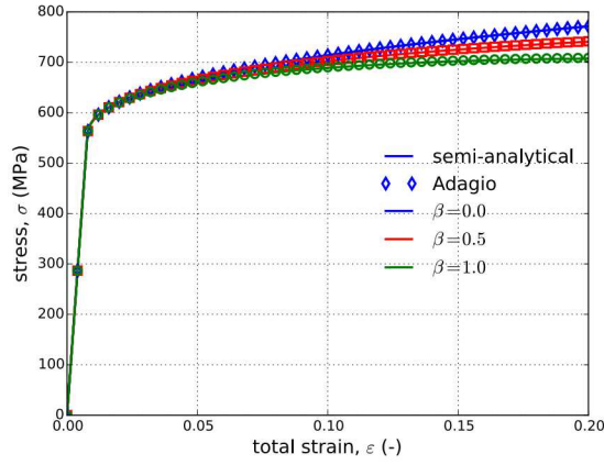
(a) Stress-strain
