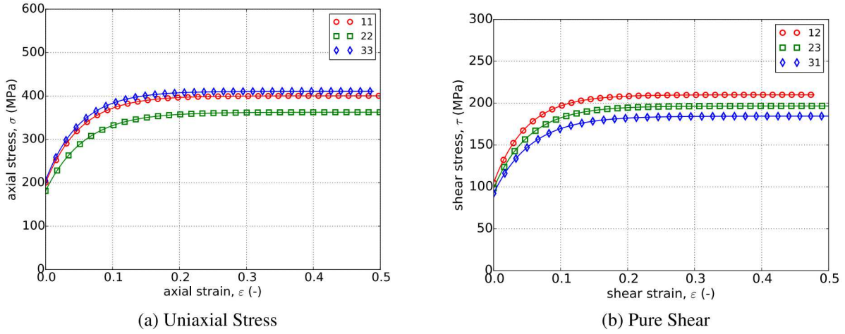
Figure 5.62: Analytical and numerical (a) uniaxial stress-strain and (b) pure shear responses of the Hill plasticity model with rate-independent, Voce hardening. Solid lines are analytical while open symbols are numerical.
