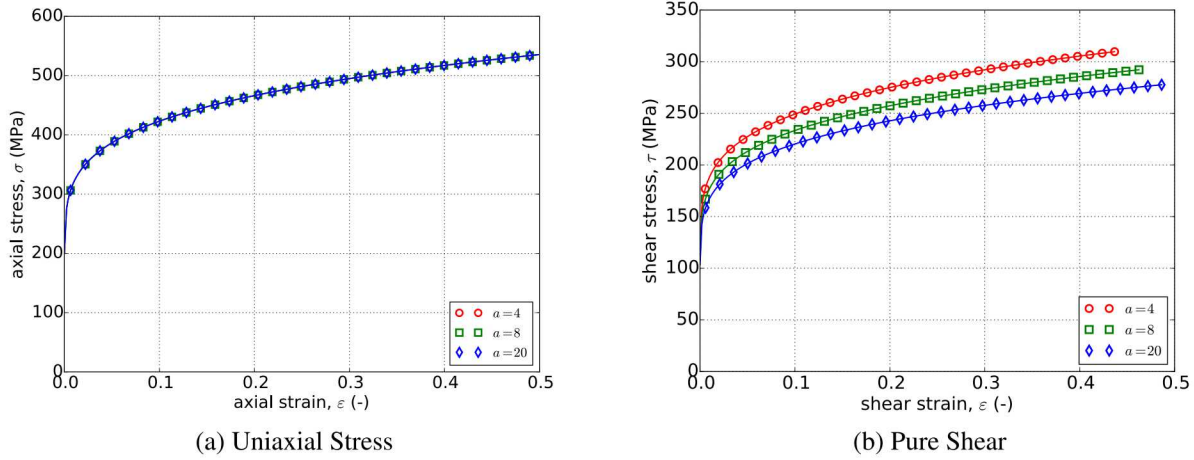
Figure 5.48: Analytical and numerical (a) uniaxial stress-strain and (b) pure shear responses of the Hosford plasticity model with rate-independent, power-law hardening. Solid line are analytical while open symbols are numerical.
