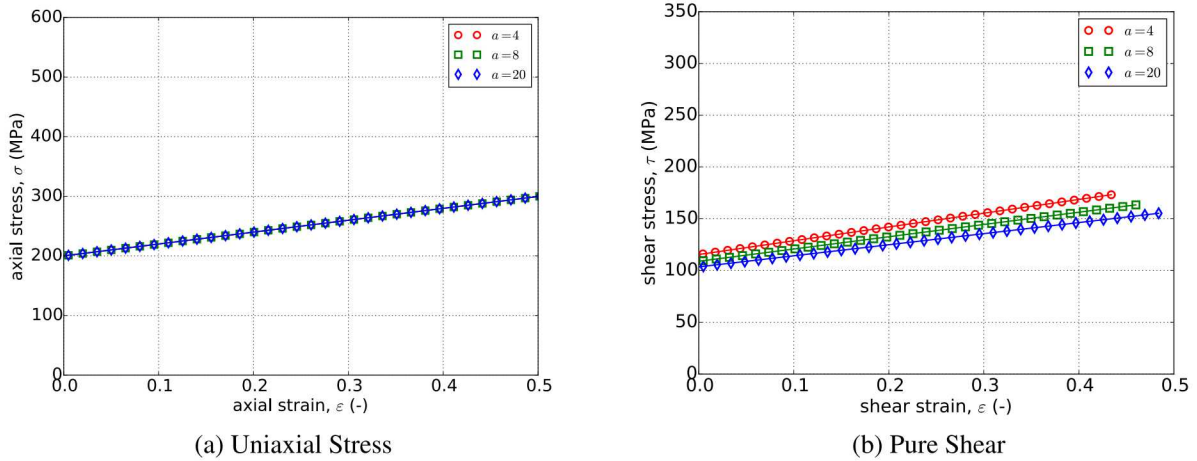
Figure 5.47: Analytical and numerical (a) uniaxial stress-strain and (b) pure shear responses of the Hosford plasticity model with rate- independent , linear hardening. Solid line are analytical while open symbols are numerical.
