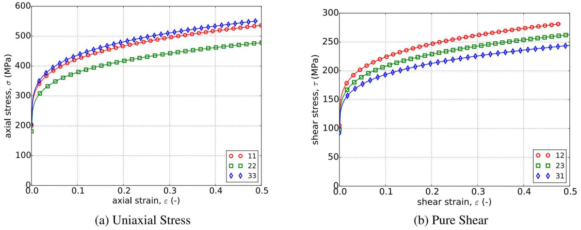
Figure 5.61: Analytical and numerical (a) uniaxial stress-strain and (b) pure shear responses of the Hill plasticity model with rate-independent, power-law hardening. Solid lines are analytical while open symbols are numerical.
