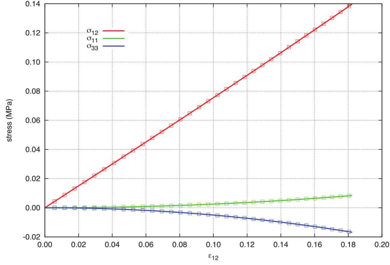
Figure 5.9: Analytical and numerical results for the neo-Hookean model subjected to a pure shear strain. The solid lines are the analytical results and the boxes are results from Sierra/SM.
