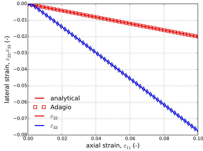
Figure 5.69: Lateral strain as a function of axial strain of 2090-T3 aluminum with Voce hardening as determined by the Barlat plasticity model both analytically and numerically.
