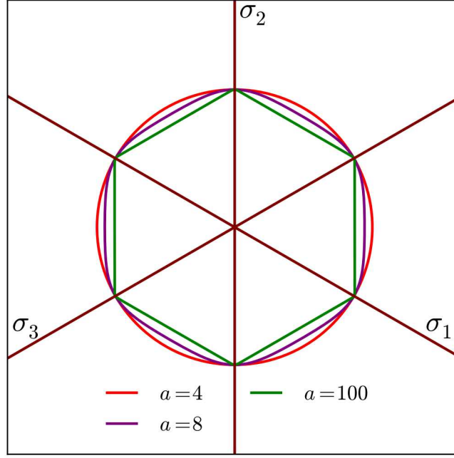
Figure 5.44: Example Hosford yield surfaces, f(\sigma_{ij}, \bar{\epsilon}^p = 0; a) , presented in the deviatoric \pi -plane. The presented surfaces correspond to the different yield exponents a = 4, 8 , and 100 .
