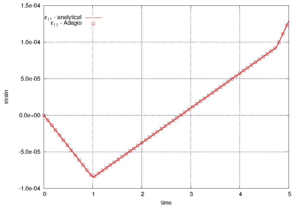
Figure 5.100: Lateral strain, \varepsilon_{11} and \varepsilon_{33} , over the course of the prescribed triaxial loading path.
