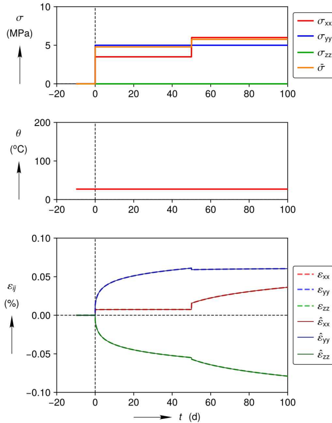
Figure 5.89: Unequal Biaxial Compression Verification Test
