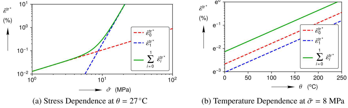
Figure 5.85: Stress and temperature dependence of the transient strain limit for Calibration 3B.
