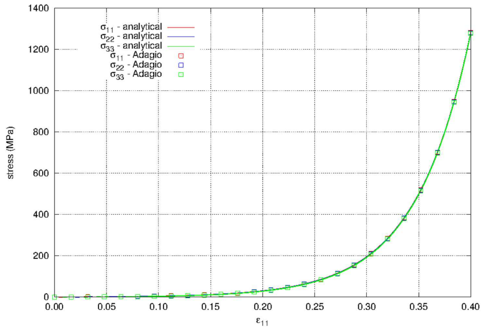
Figure 5.93: The normal stresses for biaxial strain in tension using the hyperfoam model. The results show agreement with the analytical results. The material properties for the model are given in Table 5.31.
