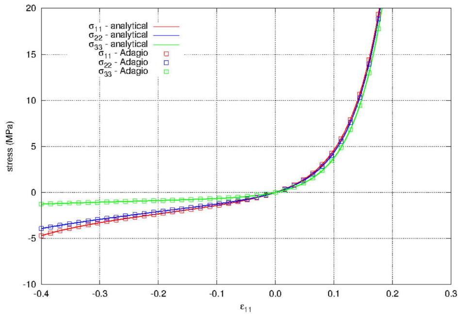
Figure 5.95: The normal stresses for biaxial strain in both tension and compression using the hyperfoam model. The results show agreement with the analytical results and that the response of the material is very different in tension and compression. The material properties for the model are given in Table 5.31.
