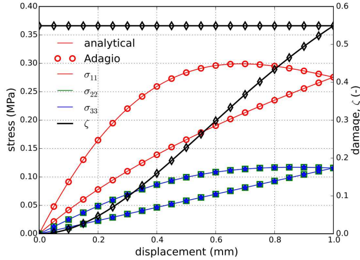
Figure 5.98: Analytical and numerical results of the stress and damage state for the uniaxial stretch case.
