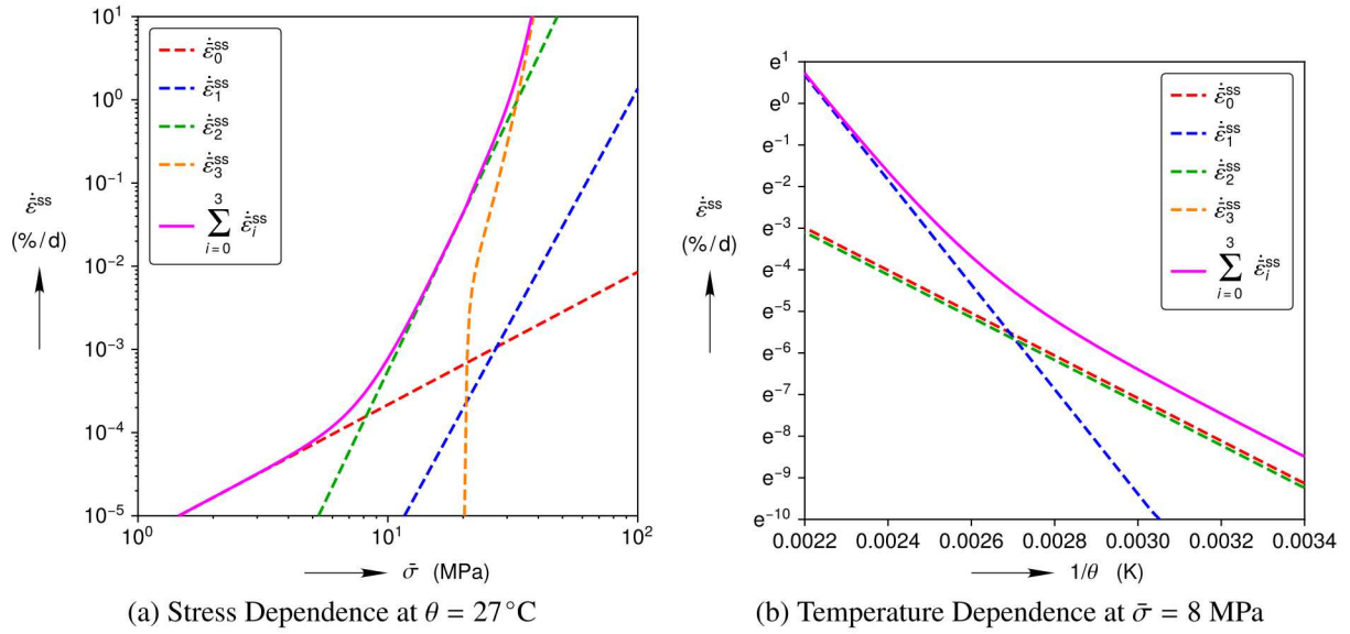
Figure 5.86: Stress and temperature dependence of the steady-state strain rate for Calibration 3B.
