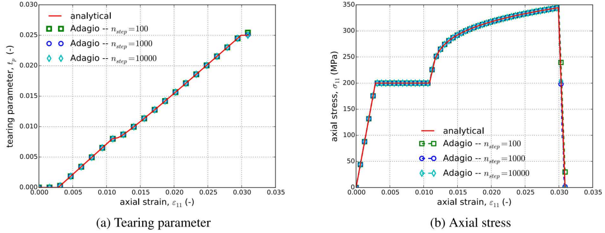
Figure 5.24: The (a) tearing parameter, t_p , and (b) axial stress-strain response for the ductile fracture model in uniaxial stress. The post failure reduction in stress depends on the time discretization or step size.
