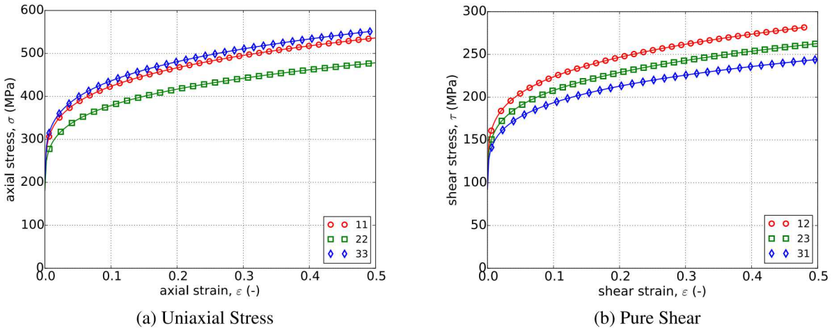
Figure 5.74: Analytical and numerical (a) uniaxial stress-strain and (b) pure shear responses of the Barlat plasticity model with rate-independent, power-law hardening. Solid lines are analytical while open symbols are numerical.
