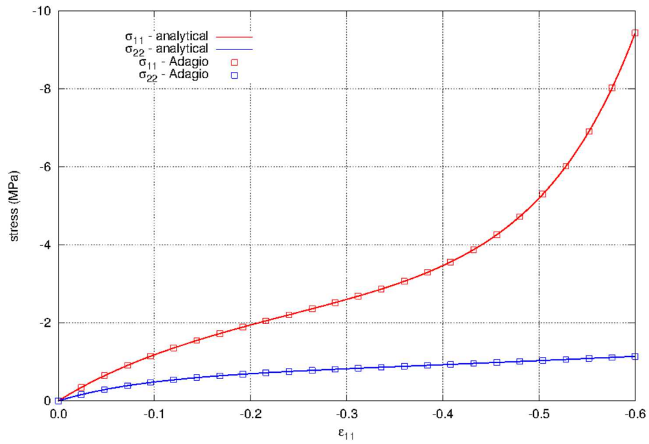
Figure 5.91: The axial and lateral stresses for uniaxial strain in compression using the hyperfoam model. The results show agreement with the analytical results. The material properties for the model are given in Table 5.31.
