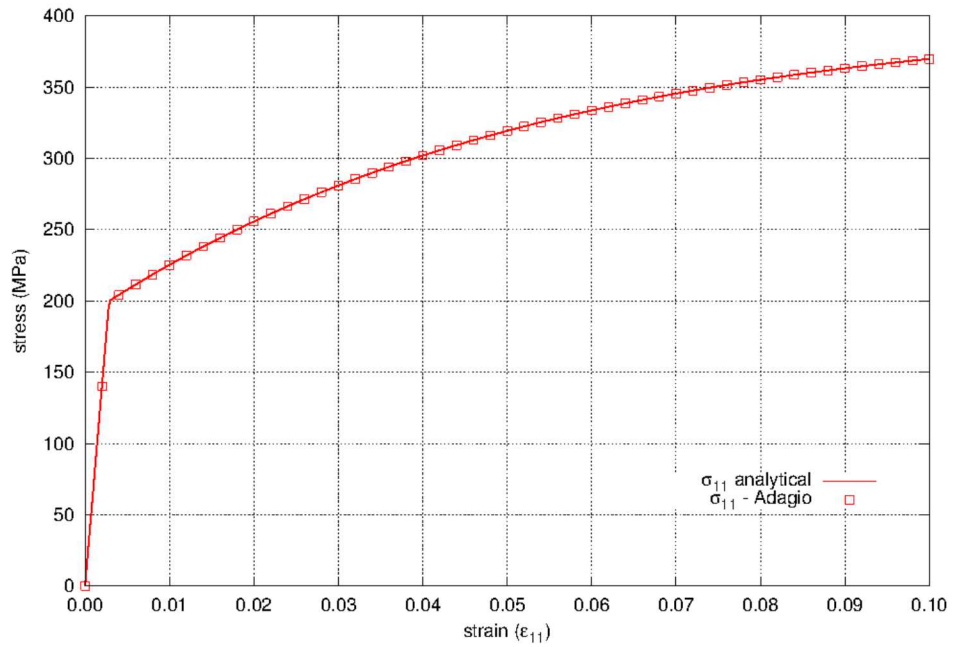
Figure 5.28: The axial stress as a function of axial strain for the multilinear elastic-plastic model with an analytical Voce law for the hardening model.
