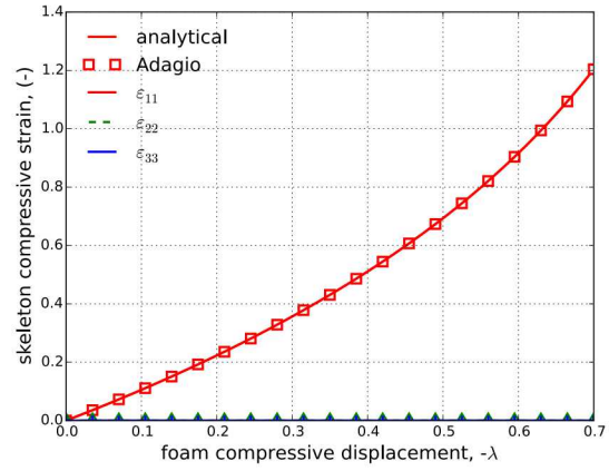
(b) Skeleton strain
