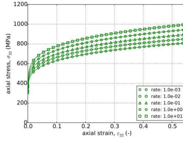
(e) Power-Law Hardening – 22
