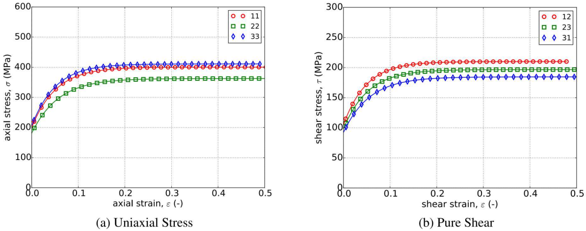
Figure 5.75: Analytical and numerical (a) uniaxial stress-strain and (b) pure shear responses of the Barlat plasticity model with rate-independent, Voce hardening. Solid lines are analytical while open symbols are numerical.
