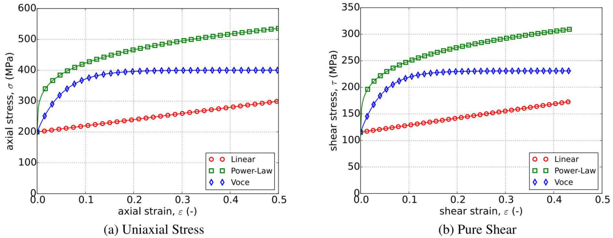
Figure 5.37: Analytical and numerical (a) uniaxial stress-strain and (b) pure shear responses of the J_2 plasticity model with linear, power-law, and Voce rate- independent isotropic hardening. Solid lines are analytical while open symbols are numerical.
