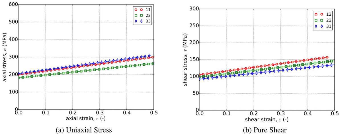
Figure 5.60: Analytical and numerical (a) uniaxial stress-strain and (b) pure shear responses of the Hill plasticity model with rate- independent , linear hardening. Solid lines are analytical while open symbols are numerical.
