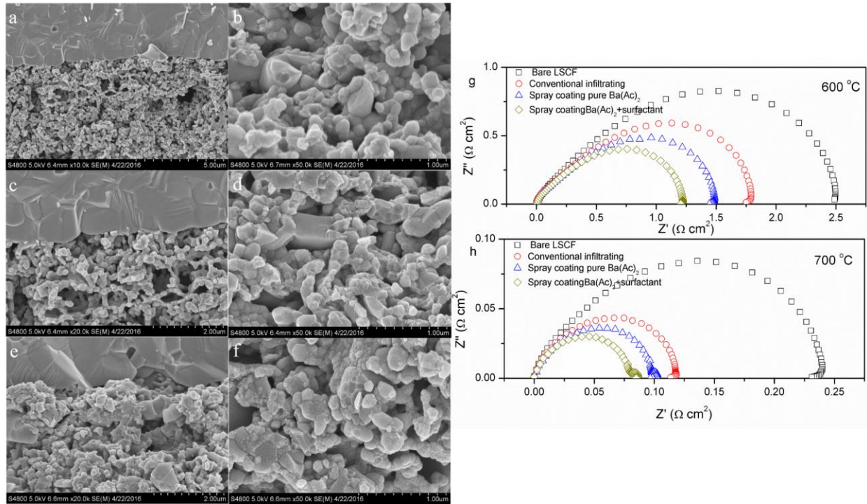
Fig.2. The cross-section SEM images for LSCF electrode with different infiltrating method: (a-b) conventional infiltrating with pure barium acetate solution, (c-d) spray-coating with pure barium acetate solution and (e-f) spray-
