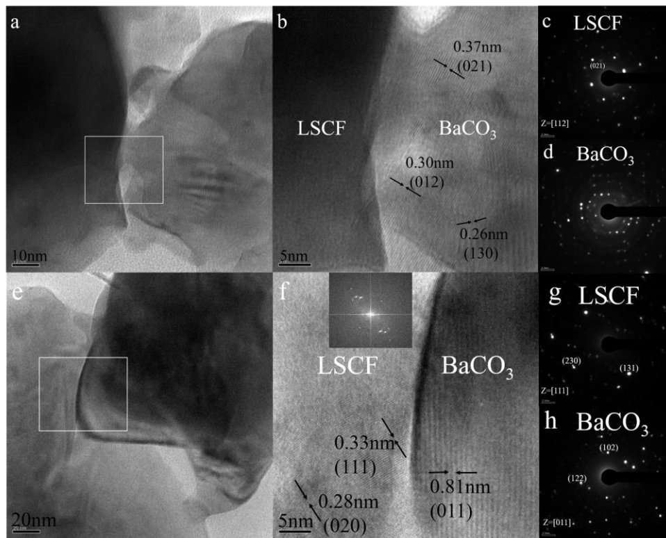
Fig.5. The TEM and SAED images for (a-d) modified \text{Ba}(\text{Ac})_2 solution and (e-h) pure \text{Ba}(\text{Ac})_2 solution spray coated LSCF electrode after 600 hour long term stability test at 600 °C. The lattice parameter and indexed crystal structure for LSCF and \text{BaCO}_3 are also labeled.
