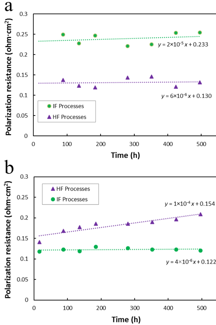
Fig.7. Area specific polarization resistances variation with operation time of (a) baseline cell and (b) BaCO 3 -infiltrated cell as a function of operation time. All impedance spectra were measured under direct current density of 0.25 Acm -2 . Linear fitting data are shown as dotted lines with equations. The polarization resistances of high frequency (HF) processes and intermediate frequency (IF) processes were determined by fitting the impedance data to the equivalent circuit model consisting of R_o , L , and two RQ elements.
