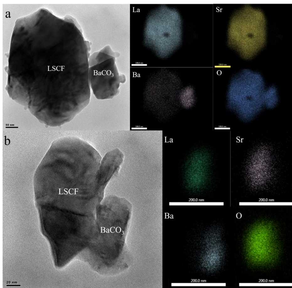
Fig.3. TEM images for LSCF and BaCO 3 particles derived from (a) pure Ba(Ac) 2 solution and (b) modified Ba(Ac) 2 solution. The energy dispersive spectrometer (EDS)-mapping images of La, Sr, Ba and O element are also presented.
