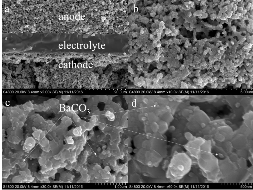
Fig.8. SEM images for MSRI full cell after 500 h discharge long term test. (a) Cross section image for whole cell, (b) LSCF-SDC cathode backbone that infiltrated with BaCO 3 and (c-d) enlarged area for cathode that isolated coated with BaCO 3 nanoparticles.
