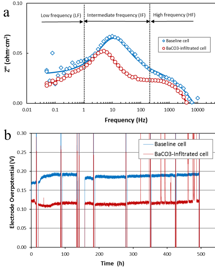
Fig.6. (a) Bode plot of the baseline cell and BaCO 3 -infiltrated cell. The impedance spectra were measured under direct current density of 0.25 \text{ Acm}^{-2} after 24 h operation at 750^\circ\text{C} . Solid lines are of simulated data fitted with the equivalent circuit model consisting of R_o , L , and two RQ elements. (b) Electrode overpotential variation with operation time of the baseline cell and BaCO 3 -infiltrated cell, monitored under the current density of 0.25 \text{ Acm}^{-2} at 750^\circ\text{C} . The electrode overpotential is derived by subtracting ohmic contribution from overall cell overpotential, which is the difference between Nernst potential (open circuit potential) and measured cell potential. The vertical lines in overpotential indicate the points when the cells were brought to open circuit condition for intermittent impedance measurements.
