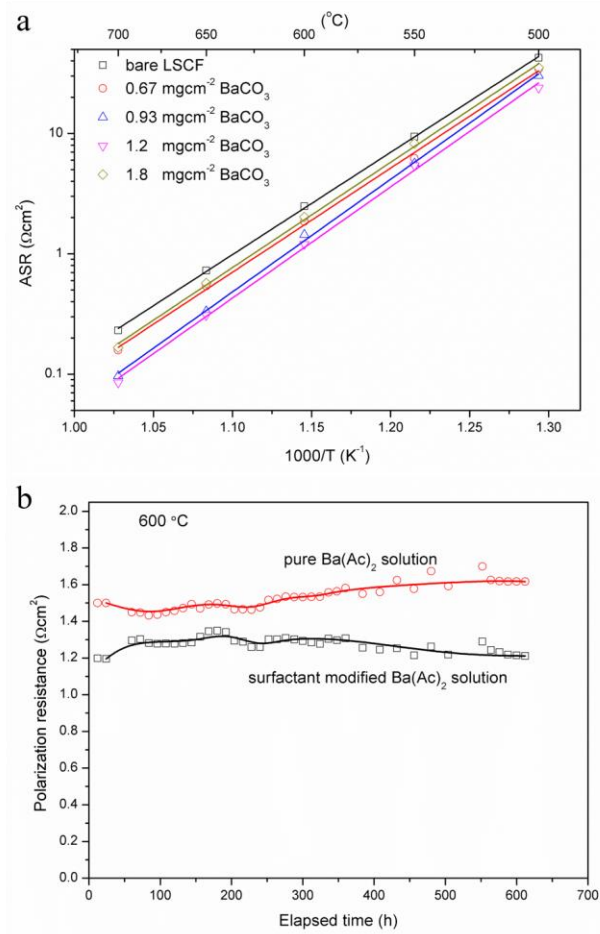
Fig.4. (a) The Arrhenius relationship between area-specific interfacial polarization resistance (ASR) and temperature for LSCF electrodes spray coated with different loadings of \text{BaCO}_3 . And (b) the polarization resistance evolution of the LSCF electrode spray coated with pure and surfactant modified \text{Ba}(\text{Ac})_2 solution after extended testing at 600 ^\circ\text{C} for 600 hours.
