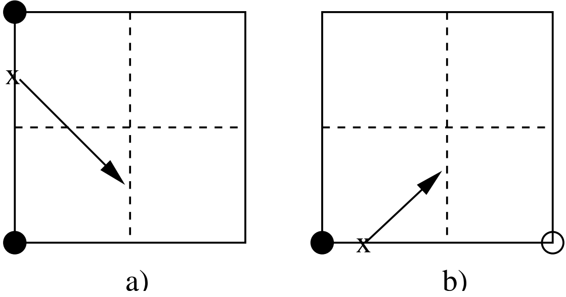
Figure 5.3. Linear profile skew upwind scheme: a) all nodes on the intersected element face are upwind of the subface, b) omit nodes on intersected element face that are downwind of the subface.
