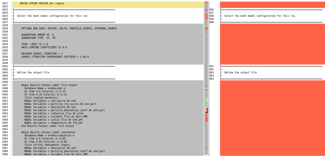
Figure 3.3. Example of input deck with Syrnix (left), and example with MPMD (right).
