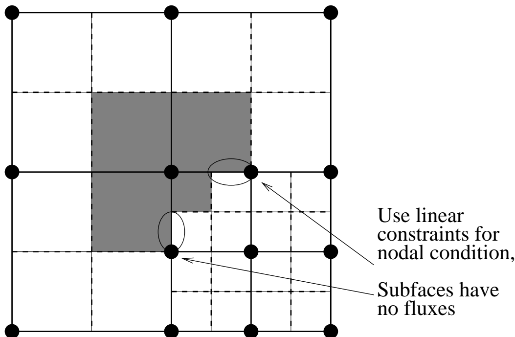
Figure 5.20. Control volume definition on an h-adapted mesh with hanging nodes. (Four-patch of parent elements with refinement in bottom-right element.)
