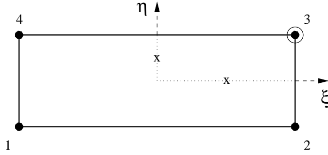
Figure 5.15. Control volume faces in a single element. Contributions to the the control volume centered about node 3.
