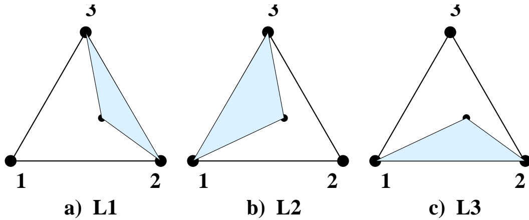
Figure 5.8. Triangular natural coordinate system, shaded area corresponds to opposite node.
