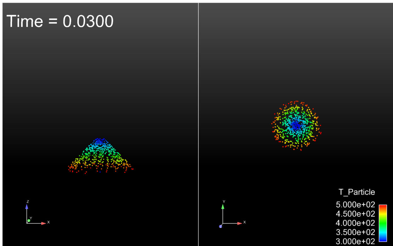
Figure 4.17. Example of particle spread from a conical shaped particle spray nozzle at early times. This nonstandard spray form was generated through the particle creation from file data mechanism. Here particle temperatures are set to be a function of their position with the hottest particles leaving the nozzle near the circular base of the cone.
