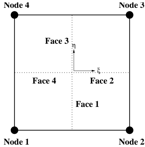
Figure 5.6. Quadrilateral element topology and numbering
