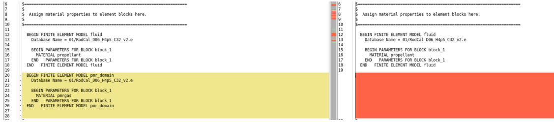
Figure 3.1. Example of input deck with Syrnix (left), and example with MPMD (right).
