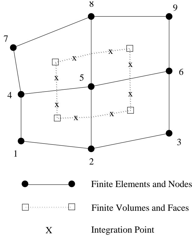
Figure 5.1. Control Volume is Centered about Finite-Element Node
