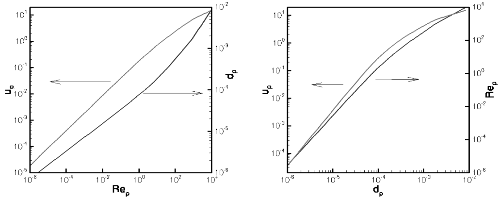
Figure 4.8. Terminal velocities for particles as a function of diameter and particle Reynolds numbers determined from 4.95 and 4.96.
