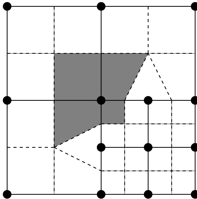
Figure 5.21. Control volume definition on an h-adapted mesh with transition control volumes about the hanging nodes. (Four-patch of parent elements with refinement in bottom-right element.)
