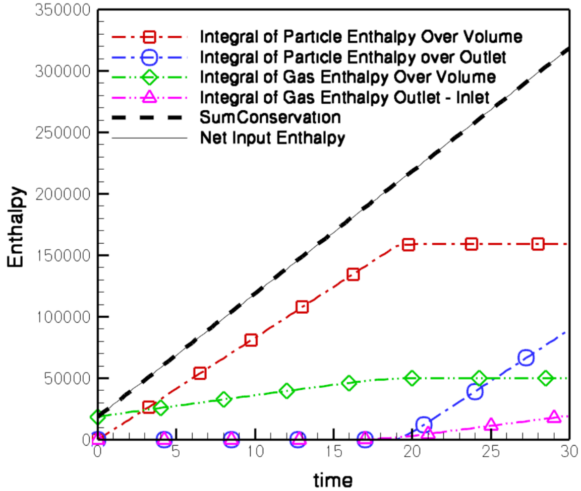
Figure 4.4. The enthalpy over time in nonreacting channel flow with hot particles injected. The net input enthalpy includes the initial domain enthalpy and the enthalpy of all of the injected particles over time. Squares show the enthalpy associated with particles in the domain. Circles show the enthalpy of the particles that have left the domain. Diamonds show the enthalpy associated with fluid in the domain. Triangles show the excess enthalpy of fluid that has left the domain (difference between the outlet enthalpy and inlet that was accounted for in the net input category). The sum of the categories indicated by symbols is shown to agree with the net input enthalpy indicating overall conservation of enthalpy.
