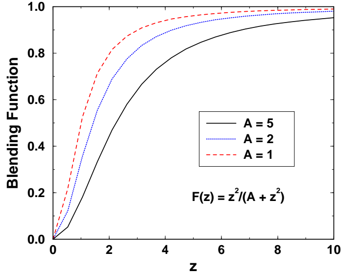
Figure 5.2. Cell-Peclet number blending function.
