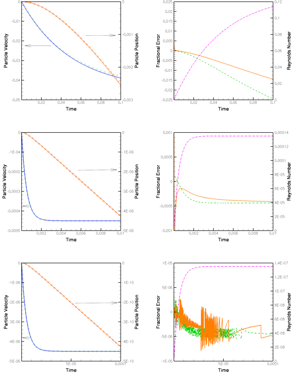
Figure 4.1. The Fuego-computed particle velocity and trajectory are compared with predictions from 4.97 and 4.98 in the left panels. The error in each prediction is shown in the right panel along with the particle Reynolds number. Parameters for the particle evolution are from 4.3 with d_p from top row to bottom row being d_p = 3 \cdot 10^{-2} , d_p = 3 \cdot 10^{-3} , and d_p = 3 \cdot 10^{-4} , respectively. In the right-hand panes the solid cures represent the position error, the dashed curves represent the velocity error and the dash-dot-dot curve shows the particle Reynolds number.
