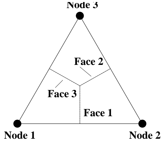
Figure 5.7. Triangular element topology and numbering
