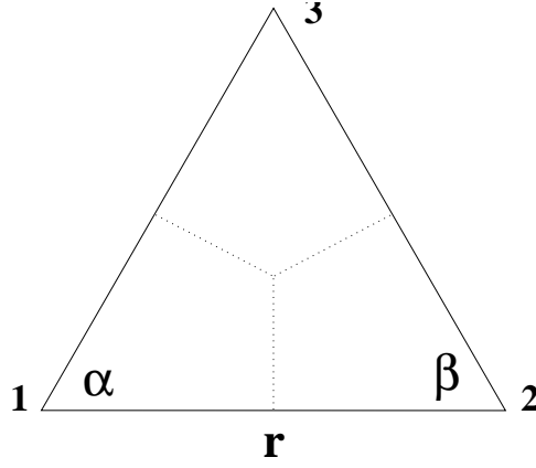
Figure 5.18. Triangular element geometry in defined by edge length and two vertex angles.
