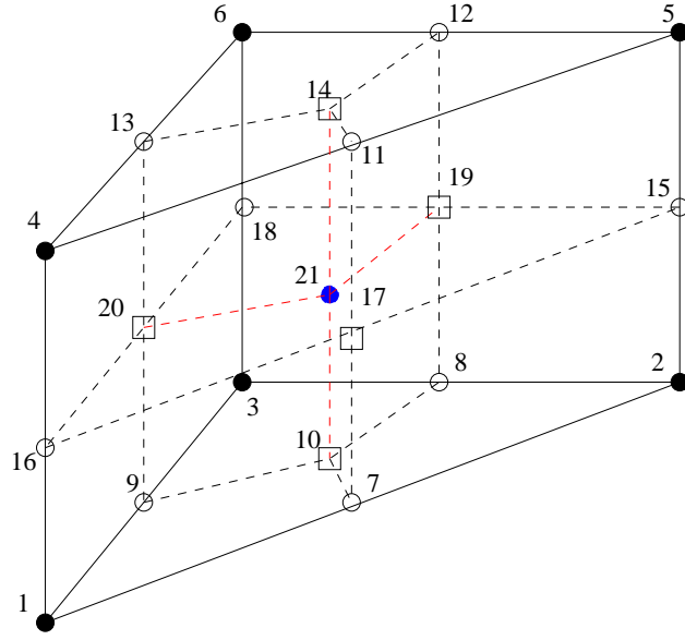
Figure 5.13. Wedge subcontrol points numbering
