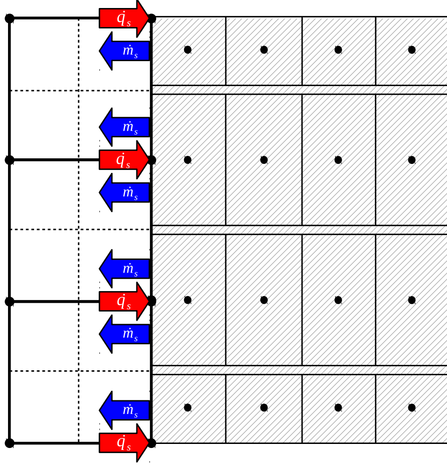
Figure 3.7. Representative mesh layout for 1-D composite fire boundary condition
