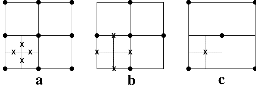
Figure 5.16. Flux integration points (X) determine nodal (•) contributions to the coefficient stencil: a) mid-face rule of CVFEM, b) edge -operator, c) centroid -operator (one-point integration).
