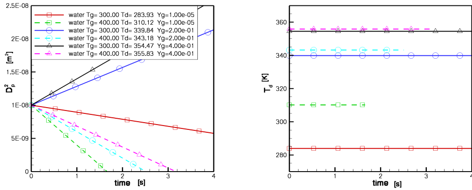
Figure 4.9. Water droplet evaporation and condensation with initial temperatures set to the wet bulb temperature. Left plot exhibits the linear d^2 -law behavior while the right hand plot shows the droplet temperatures as constant (no heating).
