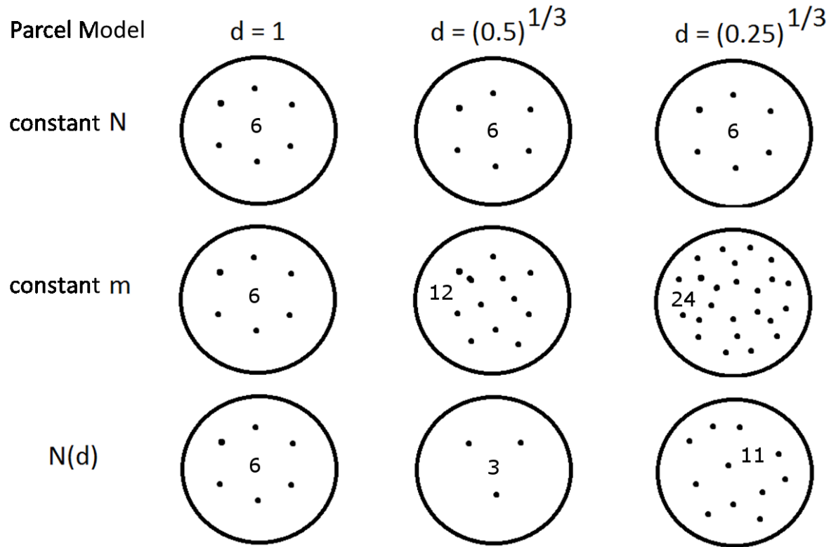
Figure 4.15. For a Lagrangian particle spray, the number of particles contained within a parcel for three representative particle diameters using constant number, constant mass, and user defined number of particles per parcel. Circles represent parcels with the points inside representing the number of particles contained in the parcel.
