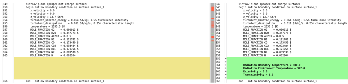
Figure 3.6. Example of input deck with Syrnix (left), and example with MPMD (right).
