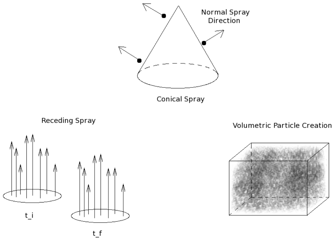
Figure 4.16. Examples of particle insertion types that can be used with particle insert from file mechanism
