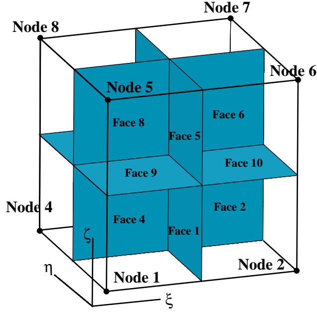
Figure 5.9. Hexahedral element topology and numbering
