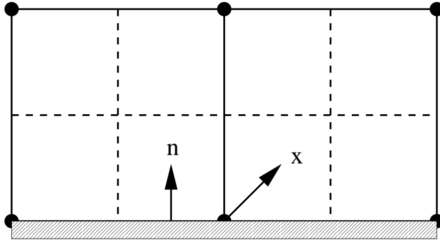
Figure 5.5. Integration locations for a wall boundary.
