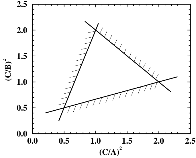
Figure 5.19. Limits of Edge-Length Ratio for Positive Coefficients in 3D CVFEM.
