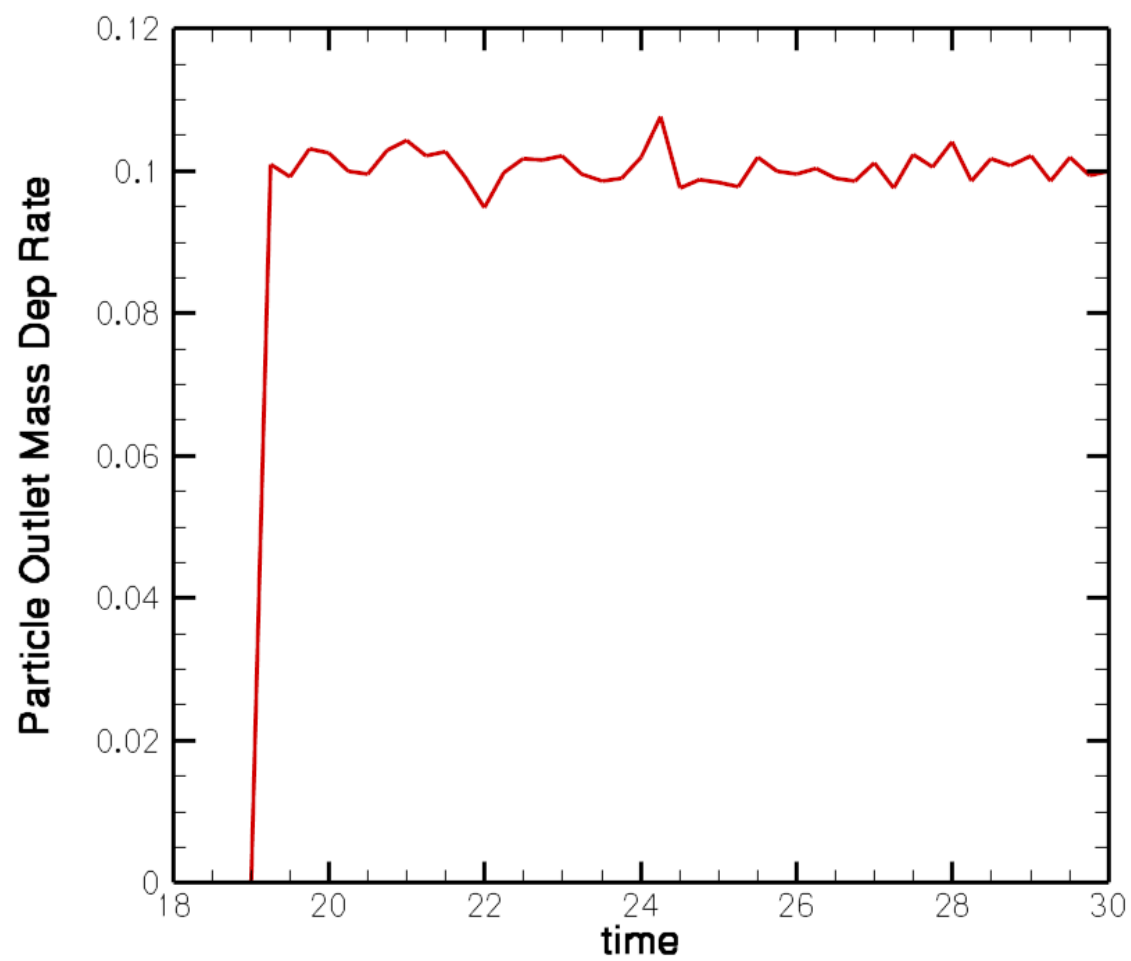
Figure 4.5. The mass deposition rate integrated over the outlet is shown as a function of time. The corresponding particle inlet mass flux is 0.1.
