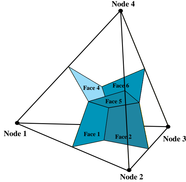
Figure 5.11. Tetrahedral element topology and numbering
