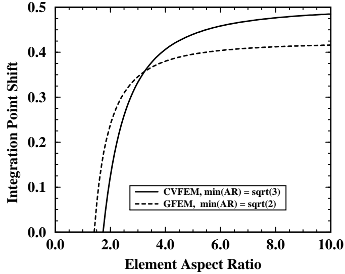
Figure 5.17. Integration point locations must be shifted out towards the element-edge with increasing element aspect ratio.
