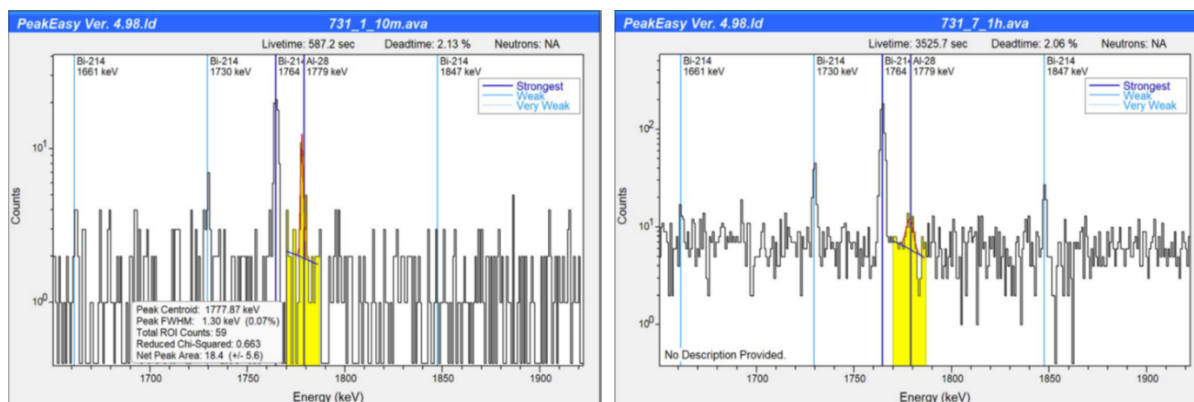
Figure 4 – PeakEasy display showing regions of ^{28}\text{Al} decay gamma energies integrated 0-10 minutes (left) and 60-120 minutes (right) after last neutron exposure.
