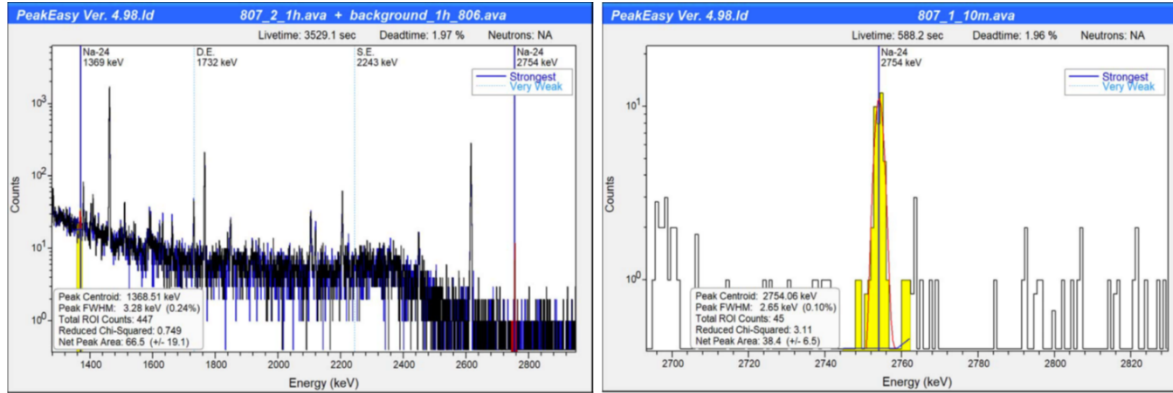
Figure 11 – PeakEasy display of the energy regions expected from the decay of Na-24 at 1368 keV and 2754 keV (left) and a zoom in of a background subtracted spectrum in the region of 2754 keV (right).
