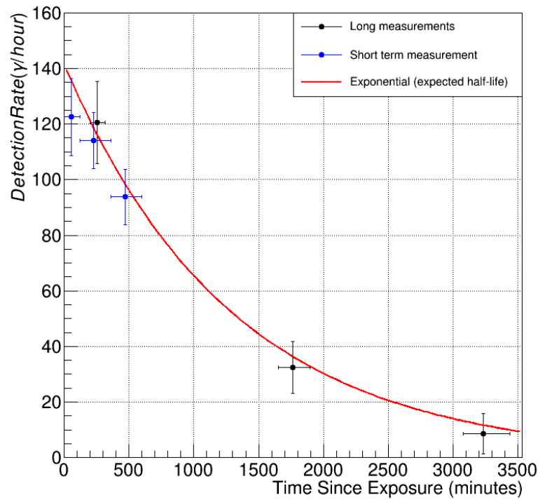
Figure 12 – Sum of net gamma-ray counts per hour in the regions of 1368 keV and 2754 keV as a function of time since last neutron exposure. The black points were taken as course, long term measurements while the blue were short measurements within the first 12 hours after last neutron exposure. The exponential curve has the half-life expected for the decay of Na-24 with a fit to the scaling factor.
