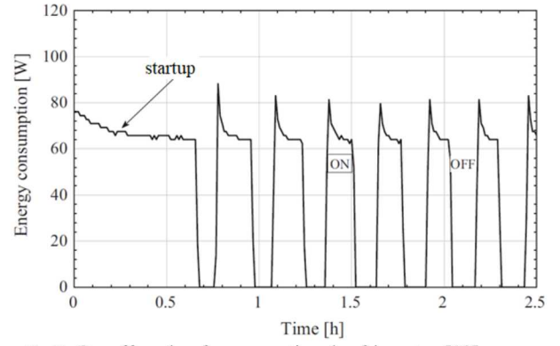
Fig 5. On-off cycle of a conventional refrigerator [12].
