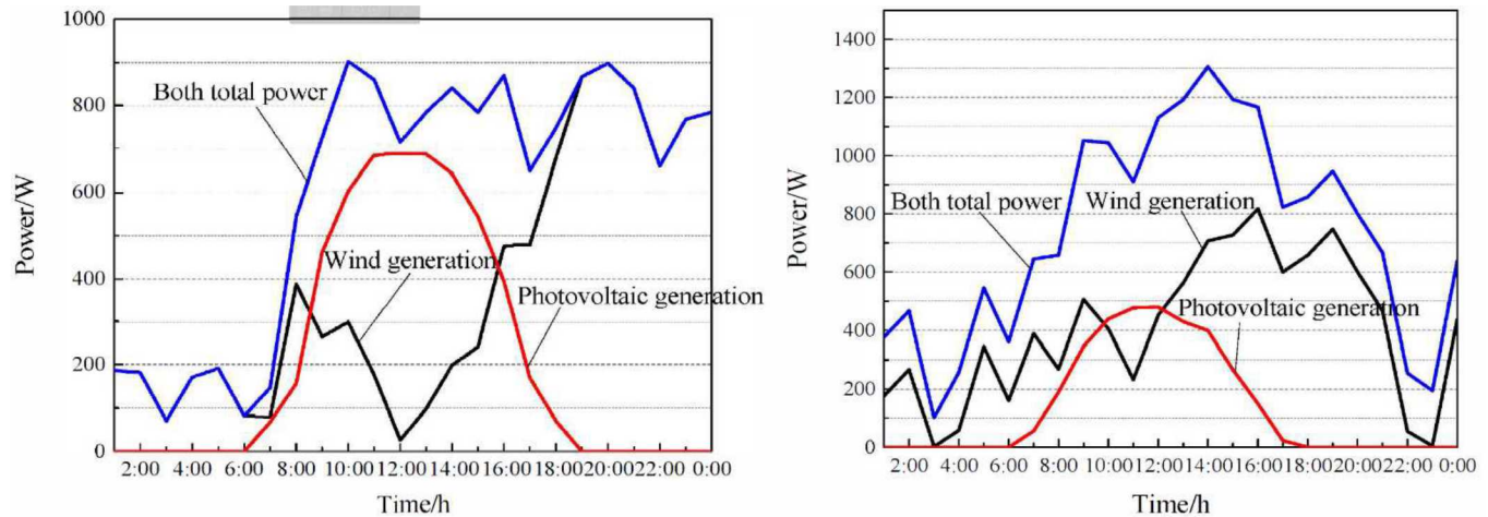
Fig 1. Output power from Wind and Solar PV generation over a 24-hour period in the summer (Left) and in the winter (Right) [11].
