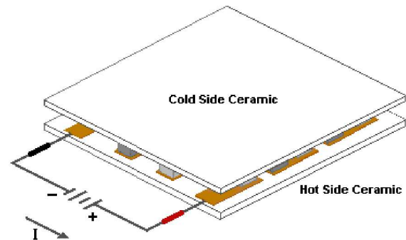
Fig 8. Operation of a thermoelectric refrigerator using the Peltier Effect [18].
