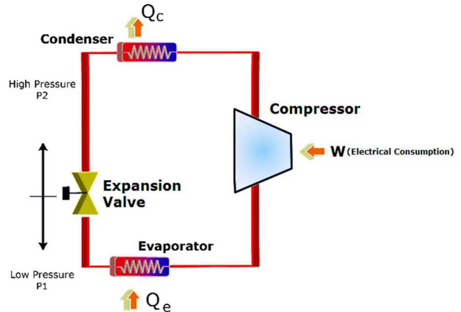
Fig 4. Diagram showing of the vapor compression cycle [13].
