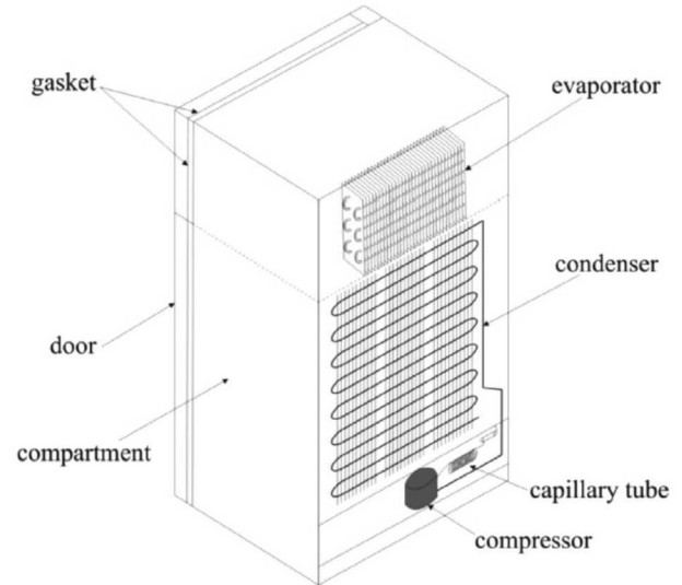
Fig 3. Diagram of a conventional refrigerator which uses the vapor compression cycle [12].
