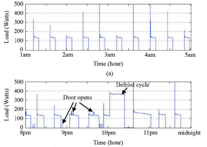
Fig 6. Load profiles of the top-freezer refrigerator unit: (a) no activity; and (b) with door opening and a defrost cycle [14].
