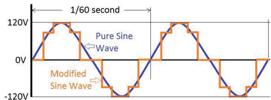
Figure 3. Inverter output with a Modified Sine Wave vs Pure Sine Wave [25].
