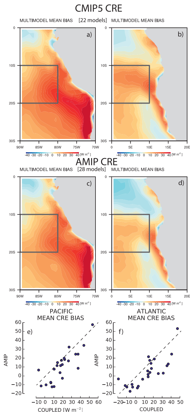
► FIG. 8. (top) Composite annual-mean net CRE biases with respect to CERES values reveal larger cloud radiative biases in (a) the Pacific than in (b) the Atlantic, based on 22 CMIP5 models. The largest biases occur at the coast. (middle) Fixed-SST (AMIP) simulations reveal similar annual-mean cloud biases in (c) the Pacific and (d) the Atlantic, implicating the atmosphere as the source for low-cloud errors, based on 28 models spanning 1950–99 when available, with most simulations beginning in 1979. The AMIP ensemble is composed of different models than the CMIP5 ensemble, based on data availability. (bottom) CREs from atmosphere-only vs coupled simulations of the same model are compared in (e) the Pacific (10°–20°S, 80°–90°W) and (f) the Atlantic (10°–20°S, 0°–10°W), where the dashed line indicates y = x . CMIP5 “historical” simulations span 1950–99, all months, and CERES EBAF [Edition 2.8 (Ed2.8)] spans 2000–13. No attempt is made to account for model independence (Caldwell et al. 2014).
