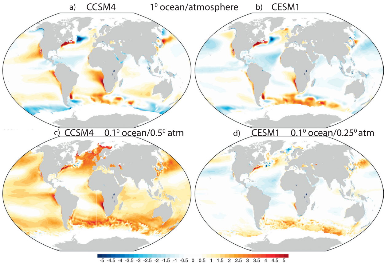
FIG. 11. SST biases from low-resolution (approximately 1° in both the ocean and atmosphere) (a) CCSM4 and (b) CESM1 (CAM5) simulations and from high-resolution (c) CCSM4 (Kirtman et al. 2012) and (d) CESM1 (CAM5) (Small et al. 2014) simulations. The high-resolution CCSM4 coupled simulation uses a 0.1° ocean with 42 oceanic levels and a 0.5° atmosphere, and the high-resolution CESM1 (CAM5) model uses a 0.1° ocean with 62 levels, a 0.25° atmosphere, and a spectral element dynamical core. Both high-resolution simulations use POP2 (Danabasoglu et al. 2012). The low-resolution simulations are averaged from 1850 through 2005 and are compared with the 1850–2005 merged Hadley–Optimum Interpolation Sea Surface Temperature (OISST) climatology (Hurrell et al. 2008). The high-resolution simulations are compared with 10-yr-mean observed SSTs centered on the appropriate observed annual-mean CO 2 concentration [1986–1995 for CCSM4’s imposed CO 2 forcing of 355 parts per million (ppm) and 1996–2005 for CESM1 (CAM5)’s CO 2 367-ppm forcing].
