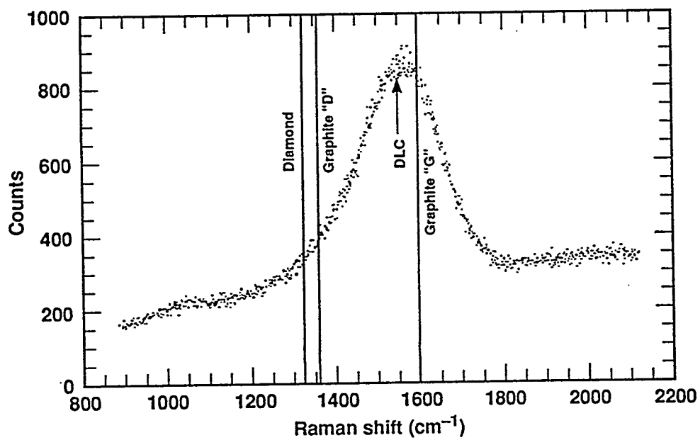
Figure 4. Raman spectrum of DLC film.
