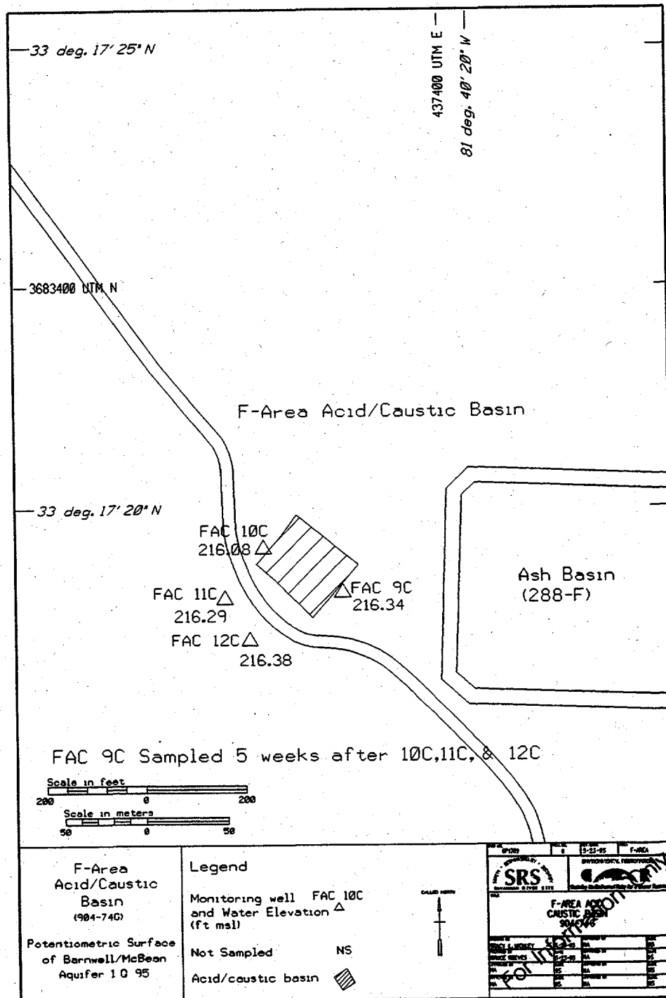
Figure 6. Potentiometric Surface Map of the Barnwell/McBean at the F-Area Acid/Caustic Basin, Monitoring Well Data
