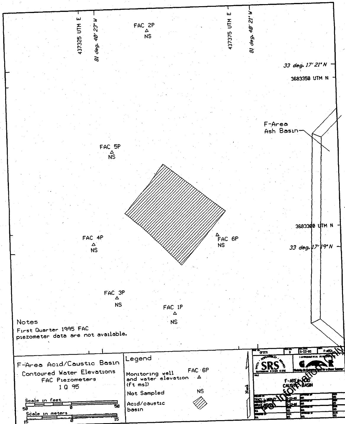
Figure 5. Water-Elevation Contour Map of the Water Table at the F-Area Acid/Caustic Basin, Piezometer Data
