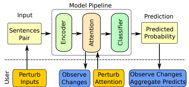
Figure 1: Perturbation-driven interrogation of the end-to-end models that follow the encoder, attention, and classifier structure. The user can generate a small perturbation of the input (i.e., replacing synonyms, paraphrasing), edit the attention, and observe the changes.
