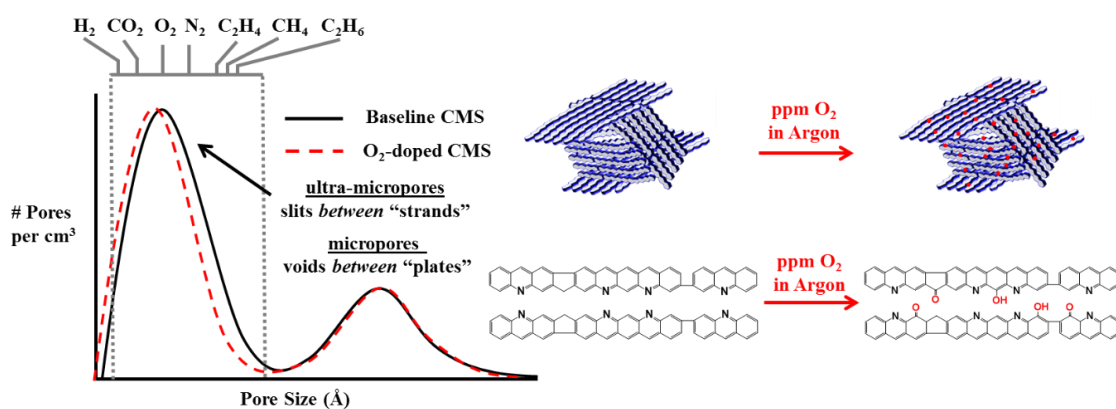
Fig. 4. Tuning of ultramicropore dimensions with O_2 doping (Reproduced with permission from [20])
