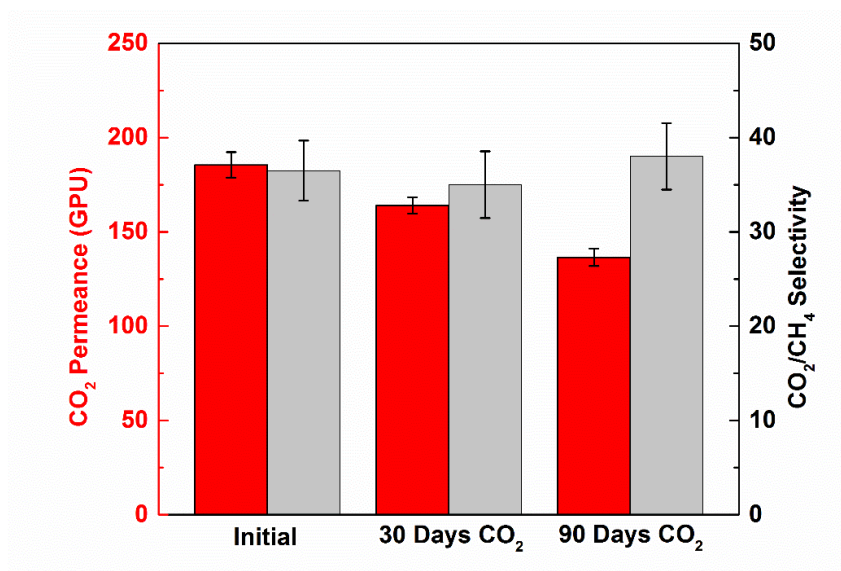
Fig. 12. Long-term stability test of asymmetric 6FDA:BPDA-DAM CMS when stored under 100 psig pure CO 2 . Adapted from [47]
