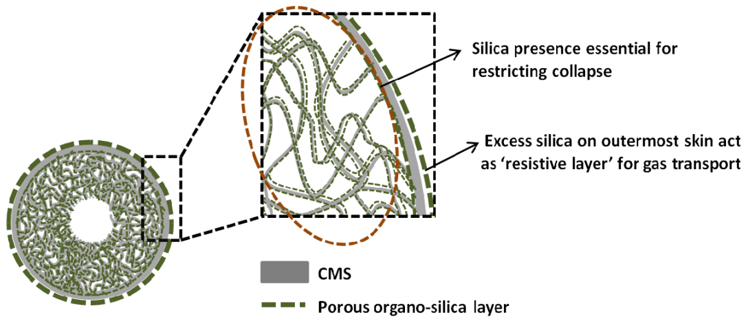
Fig 13. Schematic representation of silica stabilization of an asymmetric CMS hollow fiber membrane (Reproduced with permission from [49])
