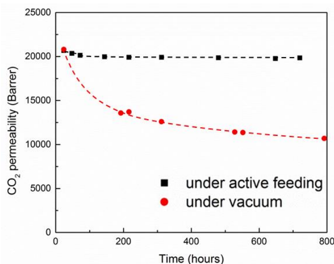
Fig 9. Stability differences of 550 °C/UHP Argon pyrolyzed 6FDA-DETDA:DABA (3:2)-derived CMS under 50:50 CO 2 :CH 4 50 psia active feed and 35 °C vs. sample stored under vacuum and tested periodically for 800 hours.
