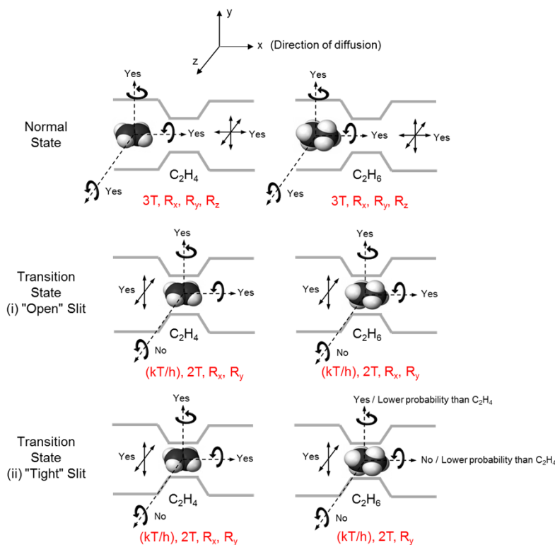
Fig 6. Possible rotational and translational degrees of freedom options in: (i) "loose" and "tight" slit ultramicropores. Double-sided arrows indicate translational ability in the x, y or z directions (Adapted from [40])
