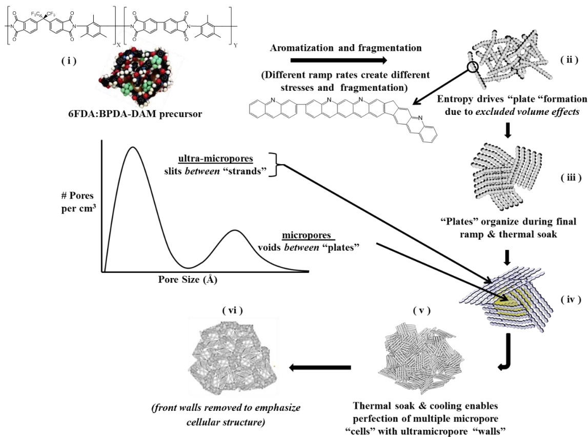
Fig 3. Envisioned steps in transformation from random coil precursor polyimide to organized amorphous CMS material with bimodal distribution of micro pores with ultramicropores (Reproduced with permission from [20])
