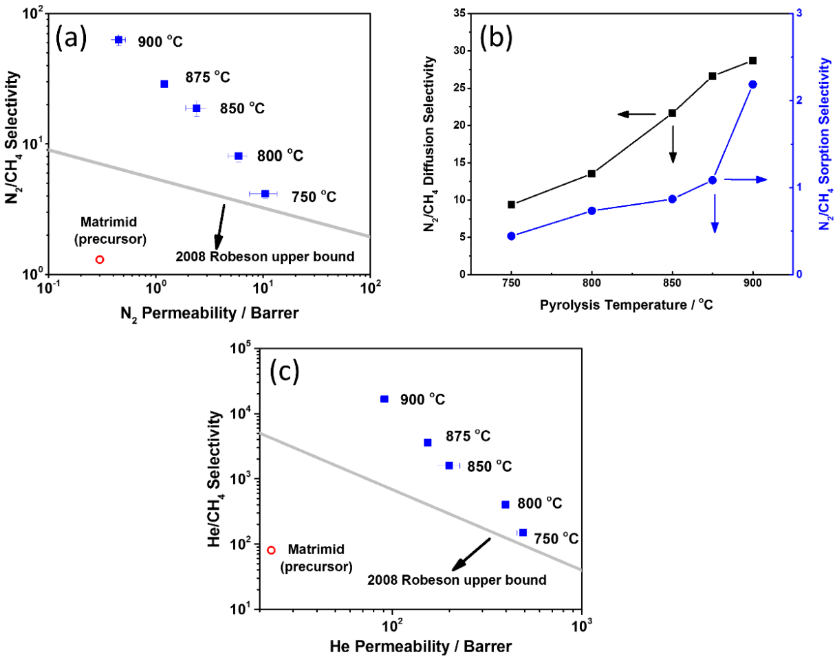
Fig 7(a). Matrimid® CMS N_2/CH_4 permselectivity ( \alpha_p ) and N_2 permeability; (b) deconvolution of \alpha_p into \alpha_D and \alpha_s and (c) He/CH_4 permselectivity ( \alpha_p ) and He permeability (Reproduced with permission from [41])
