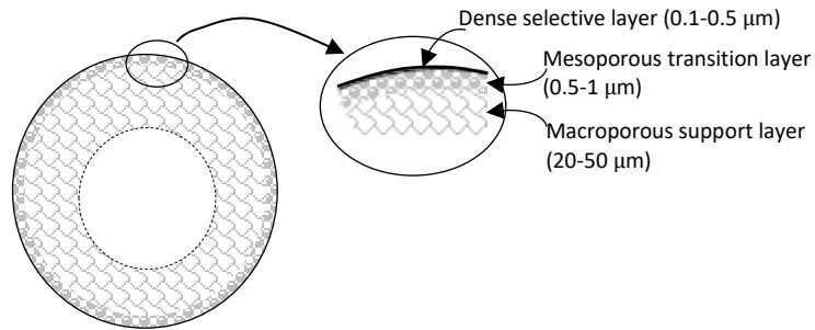
Fig 11. Schematic of asymmetric precursor fiber
