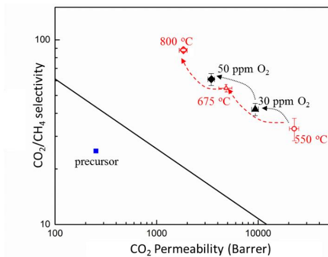
Fig 5. O 2 doping of 6FDA/DETDA: DABA derived CMS for 550 °C pyrolysis
