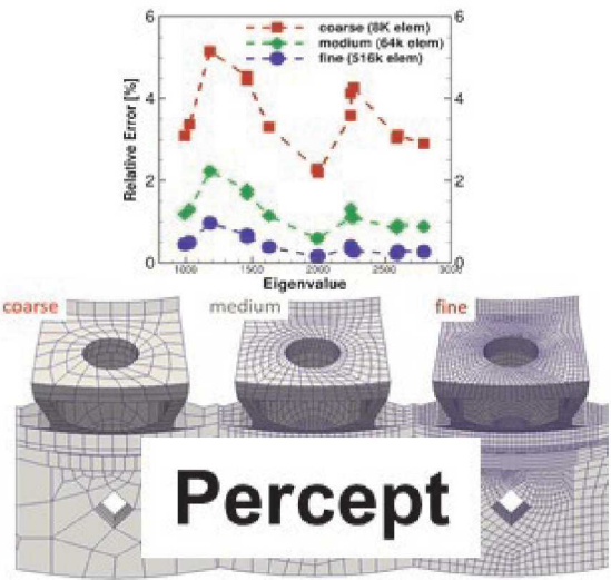
Uniform mesh refinement (UMR) performed with Percept toolkit in Sierra. Percept includes a capability that can refine very large meshes in parallel.
