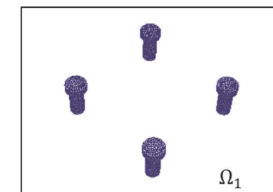
Example of a bolted joint geometry coupled iteratively with the Schwarz Alternating Method.
