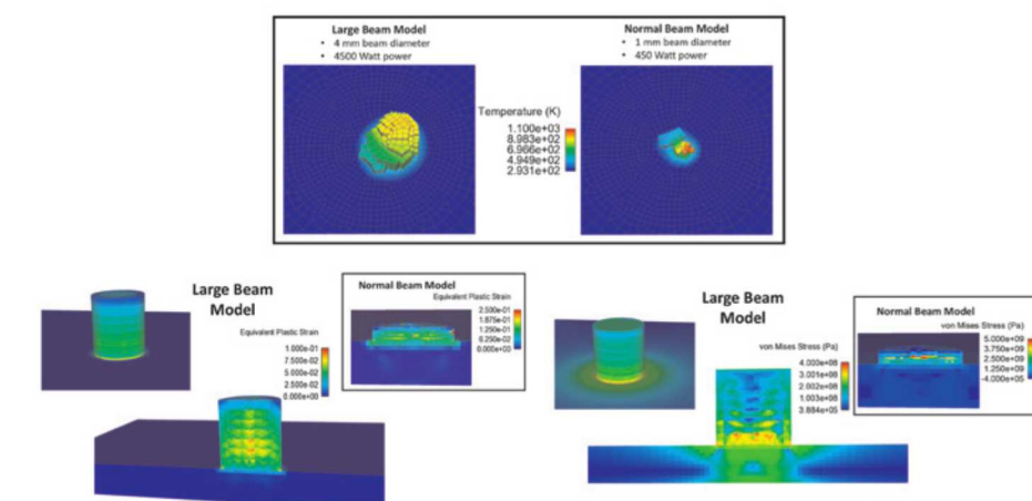
Comparison of temperature profiles, plastic strain, and residual stresses for “lumped laser method” and normal beam model for 304L stainless steel build
