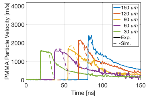
Fig. 10: Experiment and full microstructural simulation particle velocity traces overlay with calibrated Arrhenius parameters ( AT=0.42 , FF=10^{9.3} ).
