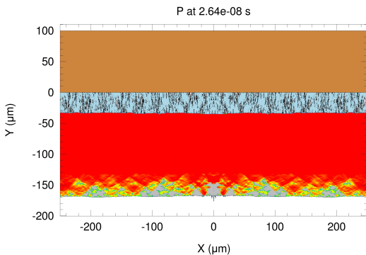
Fig. 8: Pressure field after flyer impact.
