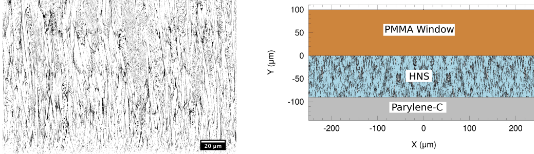
Fig. 2: Binary SEM image of ion-beam faced HNS film (left). Example 2D simulation geometry with inserted microstructure (right).
