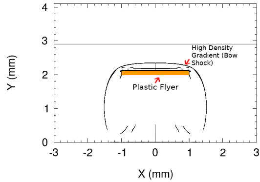
Fig. 5: Density gradient field. Gradient values clipped to only display large gradients (shocks).
