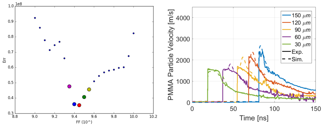
Fig. 7: One-dimensional flyer impact simulation with presence of air. FF and AT parameter calibration space, with minima highlighted (left). Experiment and simulation particle velocity traces overlay with calibrated Arrhenius parameters (right).
