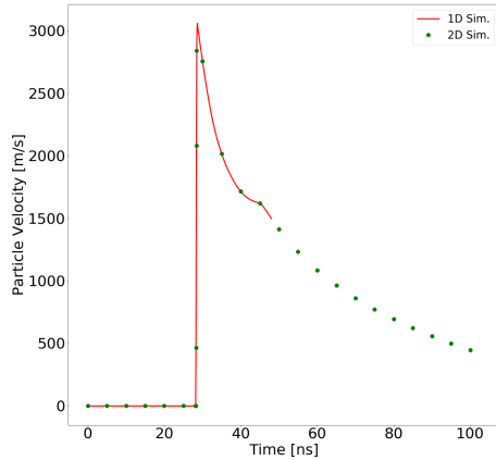
Fig. 3: Particle velocity trace in one and two-dimensional simulations are indistinguishable, demonstrating one-dimensionality in area of interest equivalent to PDV probe spot size for calibration simulations at impact velocity above threshold.
