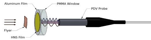
Fig. 1: Schematic of experiment. Image from Olles et al. 5
