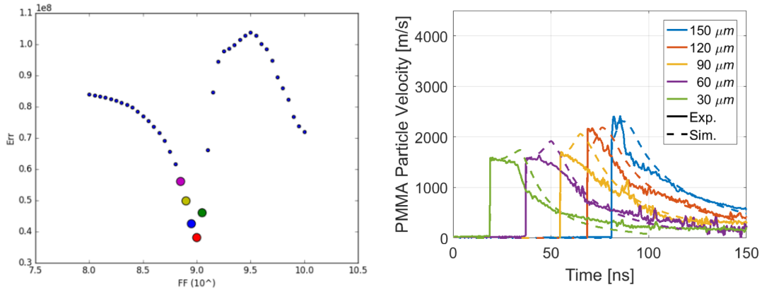
Fig. 6: One-dimensional flyer impact simulation without presence of air. FF and AT parameter calibration space, with minima highlighted (left). Experiment and simulation particle velocity traces overlay with calibrated Arrhenius parameters (right).
