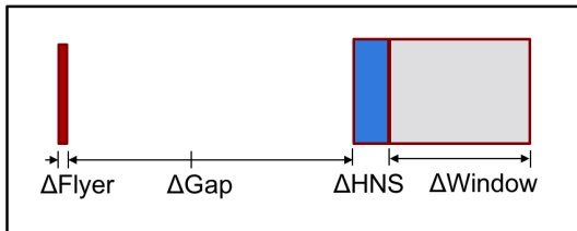
Fig. 4: CTH input geometry sketch.
