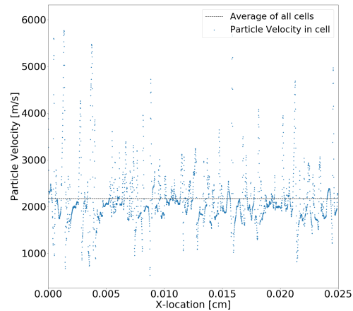
Fig. 9: Particle velocity at every cell at HNS-PMMA interface in PDV probe spot-size.
