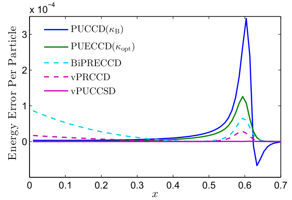
FIG. 7. A comparison of variational and similarity transformed energies for the Lipkin model with 50 particles.
