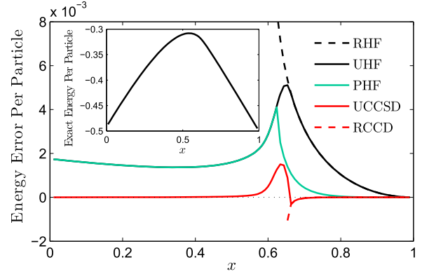
FIG. 2. Errors with respect to the exact result for the 50-particle Lipkin Hamiltonian. By “RHF” and “UHF,” we mean the Hartree-Fock solution which preserves or breaks parity symmetry; “RCCD” and “UCCSD” then refer to coupled cluster on top of the symmetry-adapted or symmetry-broken mean-field. Note that single excitations on the symmetry-adapted reference are zero by symmetry. We also show parity-projected broken-symmetry calculations as “PHF.” The RCCD energy is complex for x \lesssim 2/3 .
