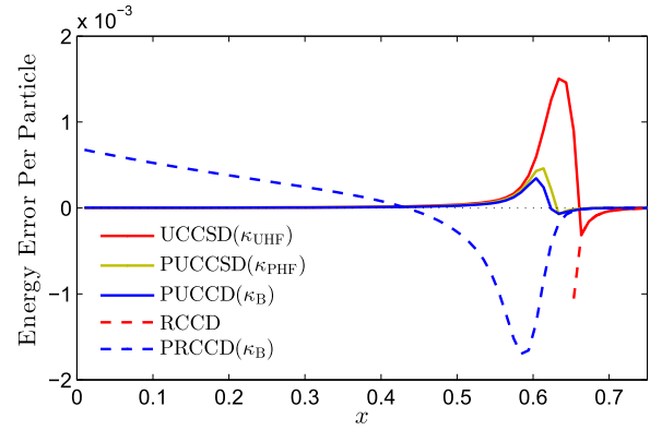
FIG. 4. Projected coupled cluster energies in the 50-particle Lipkin Hamiltonian.
