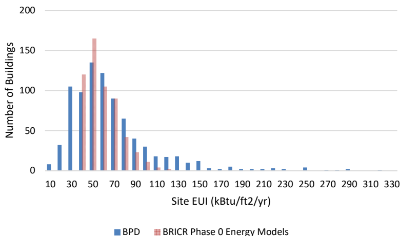
Figure 4. Energy distribution of office buildings from BPD and the BRICR Phase 0 Baseline Simulation Results
