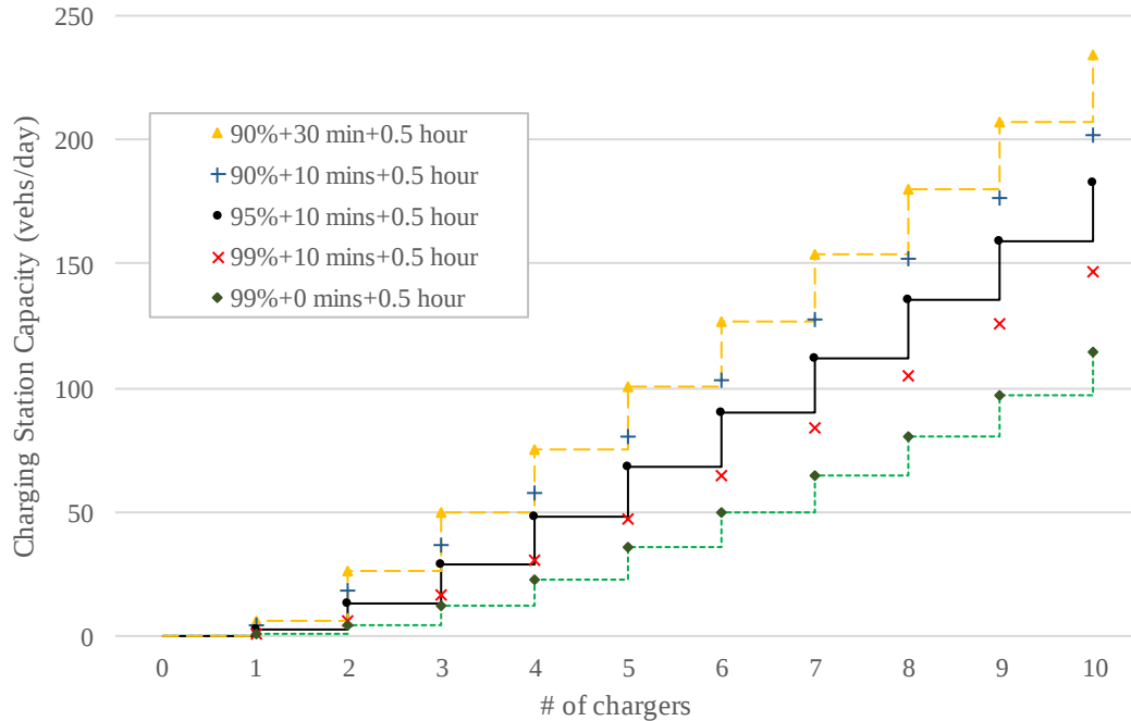
Figure 1. Relationship of Maximum Charging Demand and the Number of Chargers
