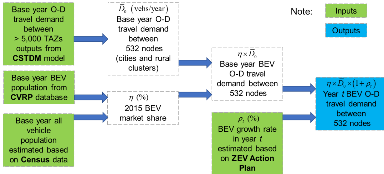
Figure 4. Yearly BEV travel demand estimation procedure
