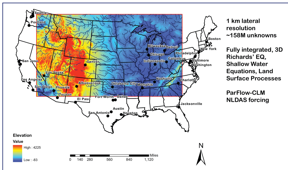
Figure A7. A proof-of-concept, 6.3M km 2 domain of a land surface model fully integrated with a 3D model of subsurface flow covering much of the conterminous U.S.
