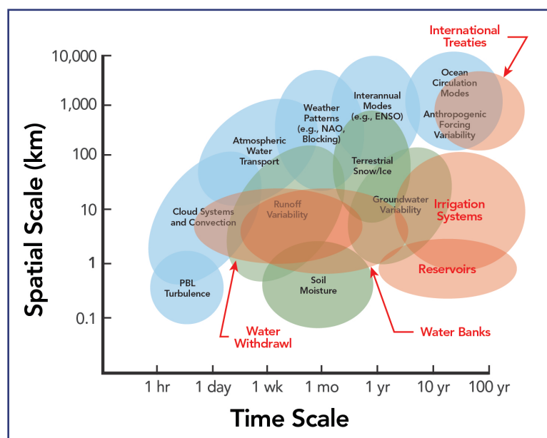
Figure 6. A schematic showing the characteristic space-time scales of atmospheric processes, terrestrial processes, and human systems in the integrated water cycle. These processes span a continuum of scales in both space and time, with significant overlaps among the processes of the three systems.
