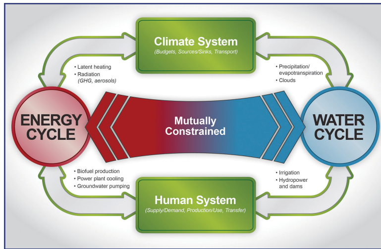
Figure 2. A schematic of the energy cycle and water cycle and their mutual constraints through various natural processes and human system interactions.
