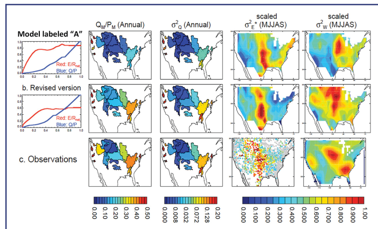
Figure A9. Results from a simple model can be used to inform the functional form of E/R_{\text{net}} used by the model labeled "A" for highly improved simulation of hydrological means and variability.
