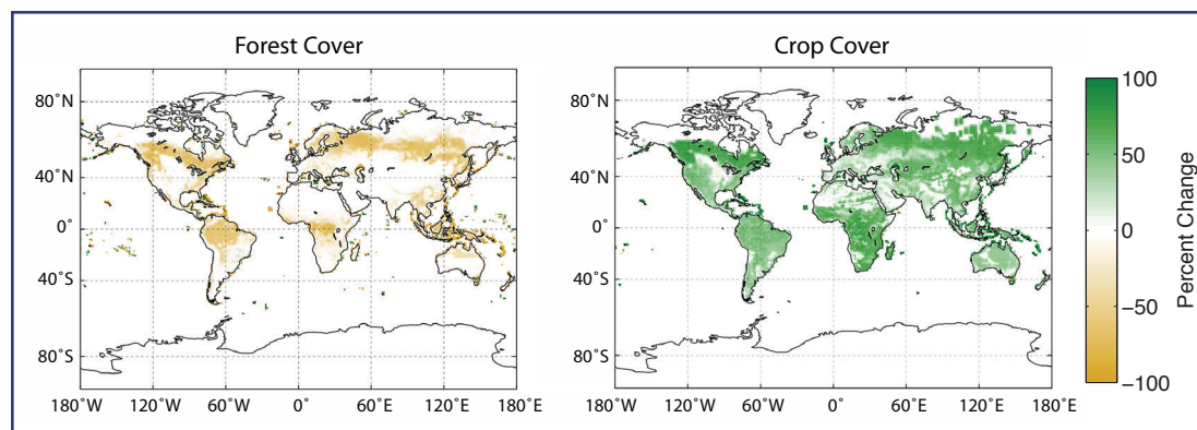
Figure 12. Potential land cover changes by the year 2100 under an energy scenario that does not value carbon on land. Results show significant decreases of forested area (left) and increases in agriculture area (right). (Figure from Jones et al. 2013, in press.)
