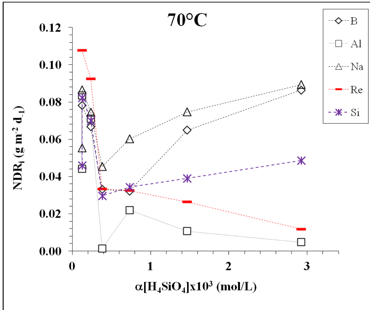
Figure 5.4. \text{NDR}_i as a function of \alpha[\text{H}_4\text{SiO}_4] at 70°C, where i=\text{B, Al, Na, Si, and Re} .
