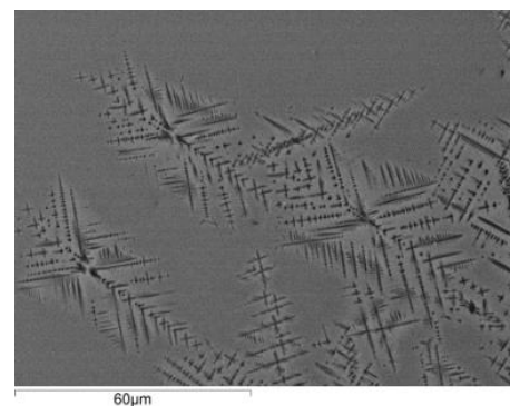
Figure 3.5. SEM micrographs of the crystallized glass layer near the crucible wall in IDF21-EC14CCC showing sodalite crystals (darker grey), probably lazurite.
