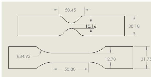
Figure 1: Dimensions of the spot foil (top) and patch foil (bottom). Dimensions are in mm.
