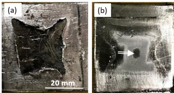
Figure 17: Spot welds of 6061-T4 (a) and 6061-T6 (b) to 4130 steel after pry test. T4 condition failed a nugget and T6 condition was peeled off leaving a hint of welding. The arrow in (b) represents the unwelded region found in the center of the spot weld.
