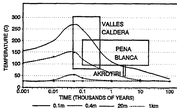
Figure 3-4. Applicability of near-field analogues to time-temperature curves for United States repository
