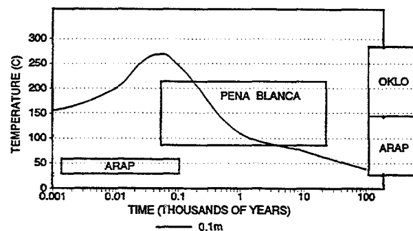
Figure 3-5. Spent fuel analogues versus peak repository temperature
