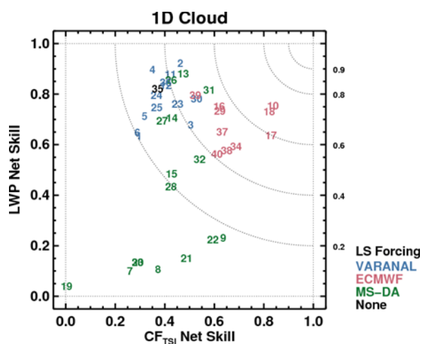
Figure 6. Scatter plot for two single-variable net-skill scores shows S(\text{LWP}) and S(\text{CF}(\text{TSI})) . In this way, simulation performance for two separate skill scores can be visualized. Should Equation 8 use these two skill scores as input, it would result in a single multivariable net skill score for each pairing, S(\text{LWP}, \text{CF}(\text{TSI})) , that is referred to as the 1D cloud skill score.
