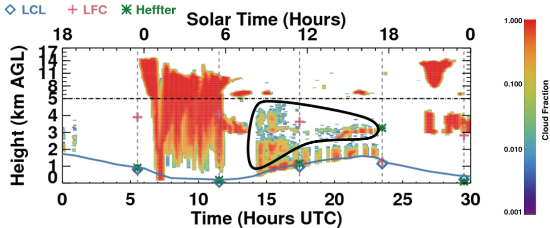
Figure 1. The 2D time-height cloud frequency from ARSCL for 30 June 2017. Based on close inspection of the data, much of the cloud fraction encircled by the black line is likely from insect contamination.
