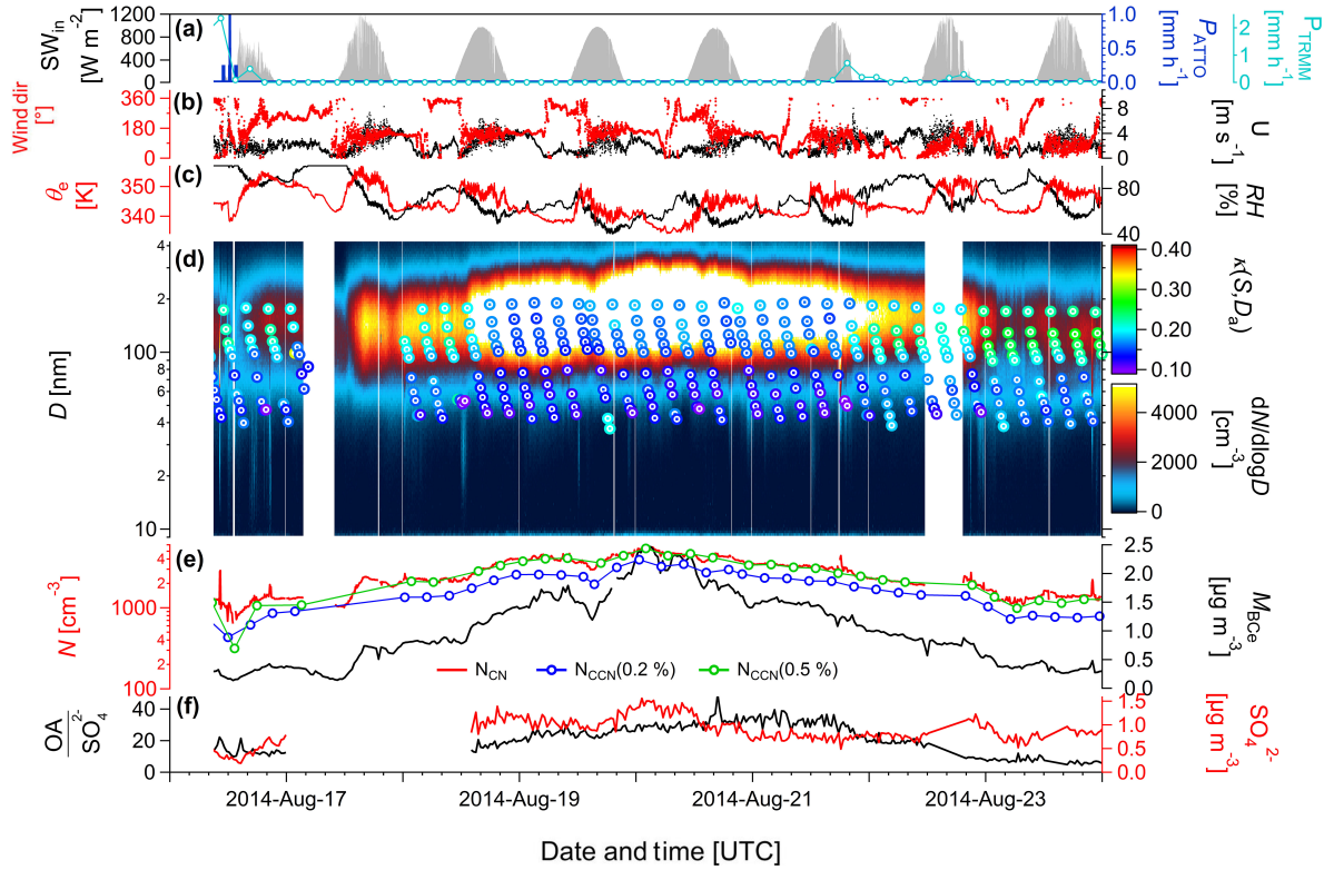
Figure 8. Selected meteorological, aerosol, and CCN time series from ATTO measurements for the biomass burning case study period, BB (see Fig. 4). (a) Incoming shortwave radiation, SW_{in} ; precipitation rates from TRMM satellite mission, P_{TRMM} ; and in situ measurements at the ATTO site, P_{ATTO} . (b) Wind direction and wind speed, U , at ATTO. (c) Equivalent potential temperature, \theta_e , and relative humidity, RH , at ATTO. (d) Overlay of two data layers showing aerosol number size distribution contour plot, dN/d\log D , as well as color-coded markers, representing time series of \kappa(S, D_a) size distributions. (e) CCN concentrations, N_{CCN}(S) , for two selected S levels; total aerosol number concentration, N_{CN,10} ; and BC_e mass concentration, M_{BC_e} . (f) ACSM-derived sulfate mass concentrations and organic-to-sulfate mass ratio.
