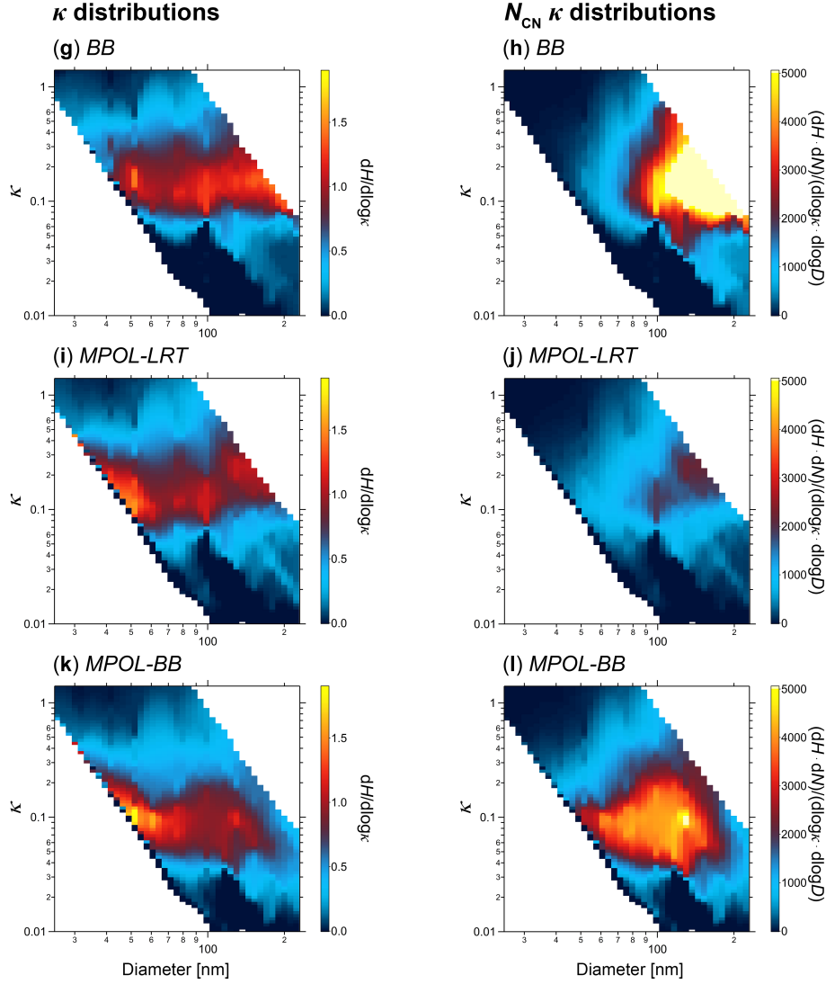
Figure 10. Average probability distribution of particle hygroscopicity, dH/d\log\kappa , on the left side and the same quantity weighted by the particle number size distribution, (dH \cdot dN)/(d\log\kappa \cdot d\log D) , on the right side, plotted over the effective hygroscopicity parameter, \kappa , and dry-particle diameter, D , for (a and b) the entire measurement period as well as (c and d) PR, (e and f) LRT, (g and h) BB, (i and j) MPOL-LRT, and (k and l) MPOL-BB conditions. The particle size distributions used for the weighting are shown in Fig. 6.
