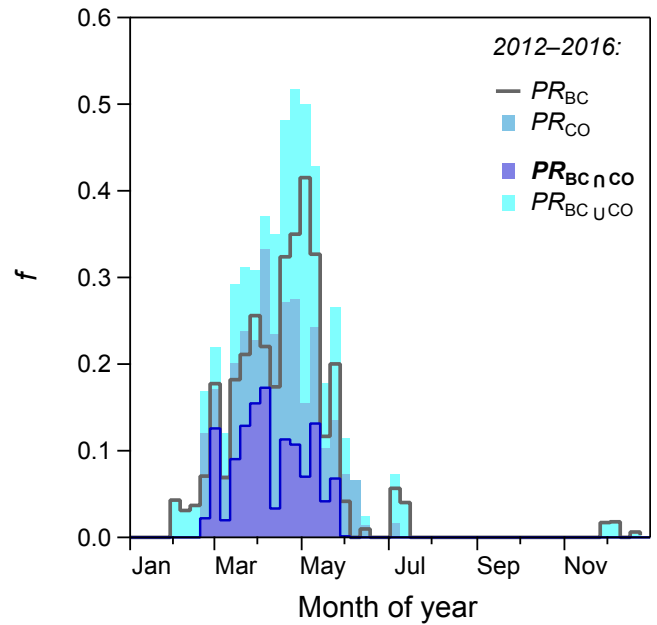
Figure 1. Seasonality of frequency of occurrence, f , of empirically pristine rain forest (PR) aerosol conditions at ATTO by means of PR_{BC} , PR_{CO} , PR_{BC \cap CO} , and PR_{BC \cup CO} filters (see Sect. 2.7). PR_{BC \cap CO} as the most robust case is used as the main PR filter throughout this work. Data are shown as weekly averages for the time period from March 2012 until June 2016. An analogous representation for the year 2014 as the CCN focal period of this study is shown in Fig. S4.
