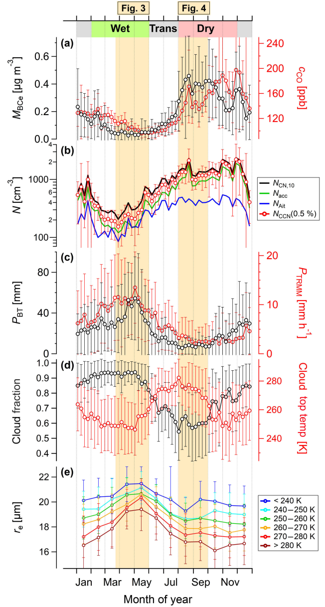
Figure 2. Seasonal cycle of selected trace gas, aerosol, and cloud microphysical parameters. (a) Pollution tracers, M_{BC_e} and c_{CO} . (b) Total aerosol number concentration, N_{CN,10} ; Aitken mode number concentration, N_{Ait} ; accumulation mode concentration, N_{acc} ; and CCN number concentration at S = 0.5 \% , N_{CCN}(0.5 \%) . (c) Precipitation products, P_{BT} , representing cumulative precipitation along BT tracks, and P_{TRMM} , representing TRMM-derived precipitation within the ROI_{ATTO} as defined in Fig. S1. (d) Satellite-derived cloud fraction and cloud top temperature within the ROI_{ATTO} . (e) Satellite-derived cloud droplet effective radius, r_e , within the ROI_{ATTO} . For a detailed characterization of the land use and recent land use change in the ATTO footprint, including the ROI_{ATTO} , we refer to C. Pöhlker et al. (2018). Data in (a) to (d) are shown as weekly averages. Data in (e) are shown as monthly averages. Error bars represent 1 standard deviation. Vertical orange shading represents 2-month time in 2014 frames of representative clean and polluted conditions as shown in detail in Figs. 3 and 4.
