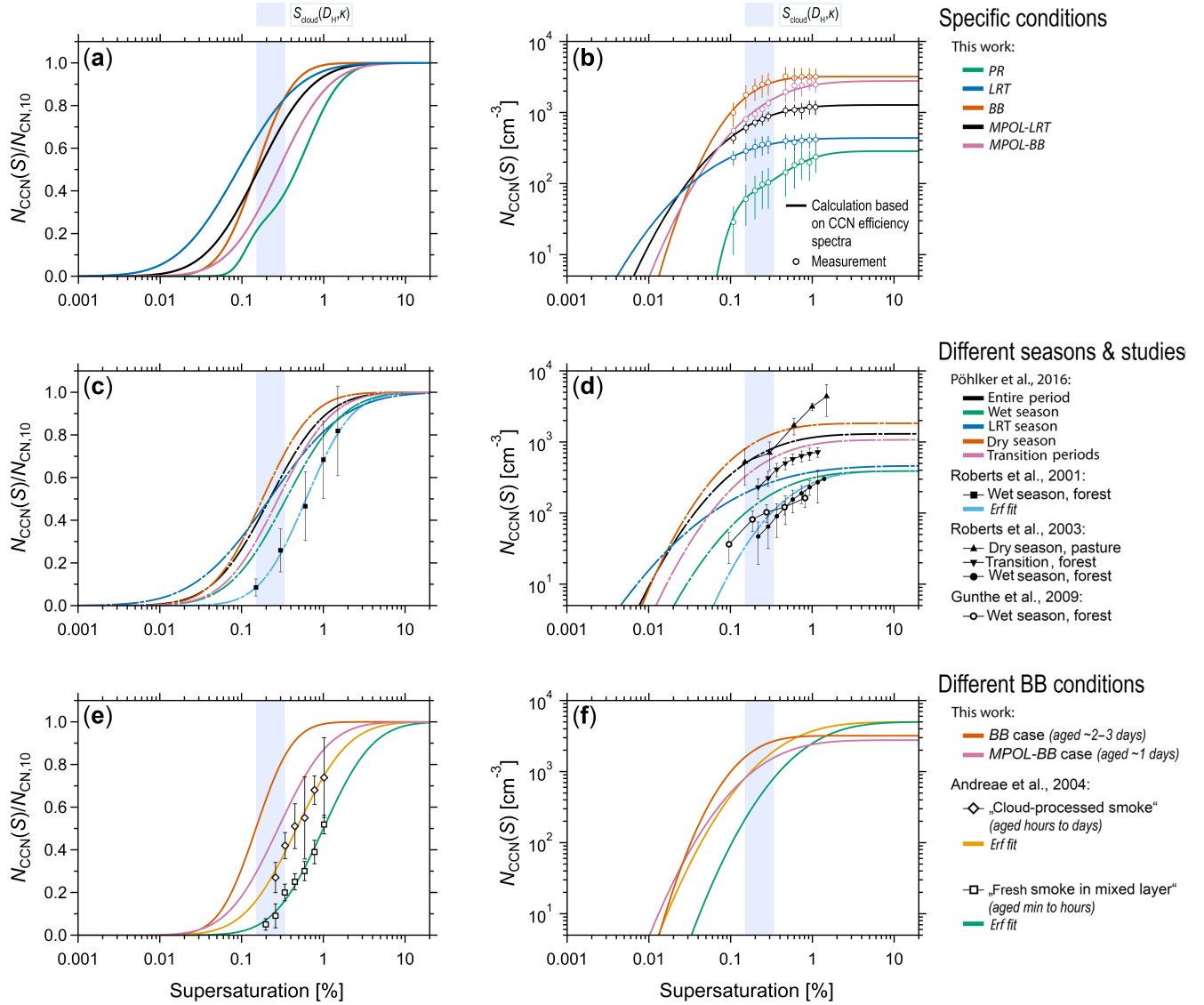
Figure 11. Overview and comparison of normalized CCN efficiency spectra and number-concentration-based CCN spectra for characteristic conditions and seasons. (a and b) PR, LRT, BB, MPOL-LRT, and MPOL-BB conditions as defined in this paper. (c and d) Seasonally averaged spectra from the Part 1 companion paper (Pöhlker et al., 2016), CCN efficiency spectrum from Roberts et al. (2001), and CCN spectra from Roberts et al. (2003) and Gunthe et al. (2009). (e and f) Conditions representing different aging states of biomass burning aerosols based on BB and MPOL-BB conditions from present work and data from a previous study by Andreae et al. (2004). For clarity the erf fit with the pre-defined variable a_1 = 1 was used for the BB case (compare Fig. 6f). CCN spectra in (b) were obtained from multiplication of CCN efficiency spectra in (a) with corresponding average aerosol number concentrations in Table 4. Markers represent measured average CCN concentrations for case study periods. Error bars at markers represent 1 SD. Good agreement of CCN spectra and markers underlines reliability of CCN efficiency spectra in representation of CCN population. Blue vertical shading represents estimated peak supersaturations at cloud base, S_{\text{cloud}}(D_H, \kappa) , in the ATTO region according to Pöhlker et al. (2016) and the present study. The colors were chosen according to Wong (2011).
