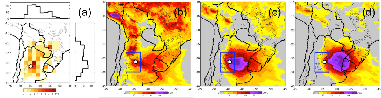
Figure 2. (a) Frequency of initiation for large MCSs (observed by TRMM satellite for November–December 2002–2010) tracked with IR brightness temperature (Tb). Frequency of IR Tb lower than 235 K for systems that initiate near the Sierras de Córdoba (blue rectangle) between 21Z and 3Z is shown for (b) 00Z, (c) +6 hours forward in time, and (d) +12 hours forward in time (Vidal et al. 2014, in prep.). The filled white circle shows the proposed AMF1 location.
