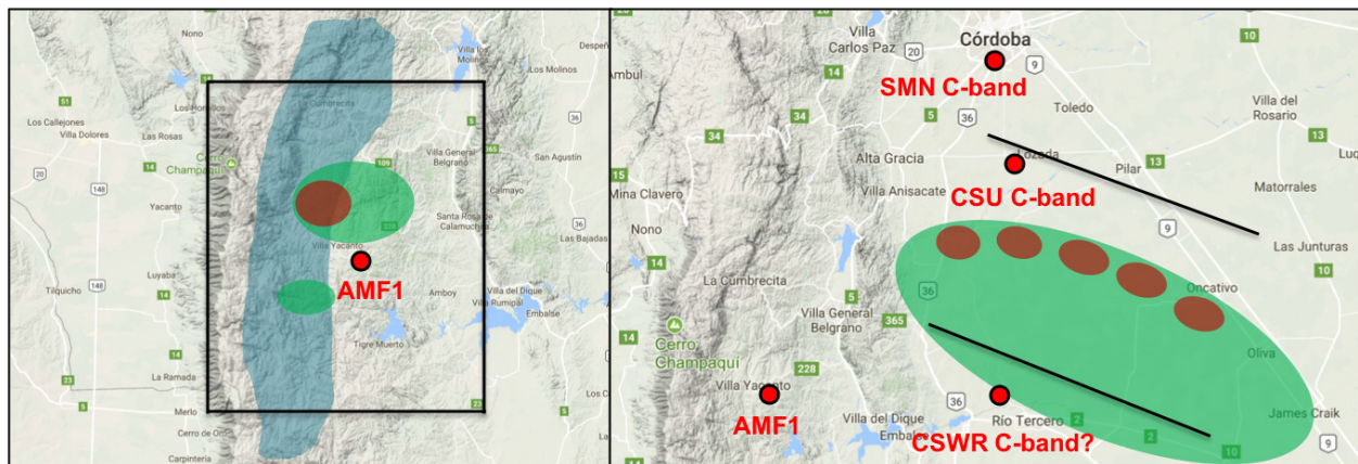
Figure 9. The flight strategy for two deep convective situations in horizontal plan views with precipitation radar locations. The CSU and CSWR C-band radars are being deployed for RELAMPAGO, which significantly overlaps with the G-1 IOP. Light blue indicates cloud, green indicates light precipitation, and red indicates heavy precipitation. Flight legs are shown in black and are flexible to changing depending on the evolution of each event. The G-1 will always remain at a safe operating distance away from deep convection such that these conceptual diagrams are altered for each situation.
