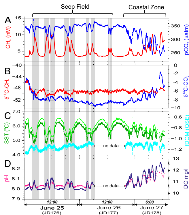
Fig. 5. Surface water time series data for the shallow shelf survey. (A) Dissolved methane concentration and p\text{CO}_2 ; (B) \delta^{13}\text{C}\text{-CH}_4 and \delta^{13}\text{C}\text{-CO}_2 ; (C) SST temperature [dark green, hull-mounted sensor; light green, EXO2 sensor (YSI Incorporated)] and fDOM; and (D) pH and DO. Seep crossings (highlighted with gray bars) are characterized by colder water containing elevated concentrations of ^{13}\text{C} -depleted methane and lower concentrations of ^{13}\text{C} -enriched \text{CO}_2 . Isotopic excursions are demarcated by dashed lines that connect \delta^{13}\text{C} values from the margins of the seep crossings. Within the seep crossings, fDOM, pH, and DO are elevated. The combined evidence suggests upwelling of cold, methane-charged (and presumably nutrient-rich) bottom water originating from the seep-stimulated phytoplankton activity in the surface water that enhanced the consumption of \text{CO}_2 . Similar trends occur within the nearshore coastal zone.
