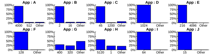
Fig. 15: Job size distribution of top 10 congestion-causing applications.
