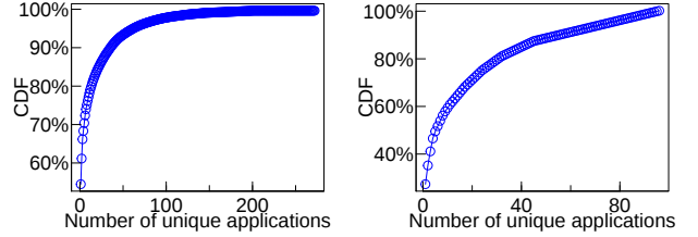
Fig. 13: Distribution of unique applications over congested node events without filter (left), and with 1-hr filter (right).
