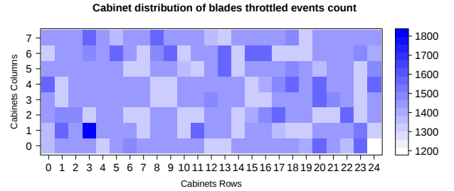
Fig. 9: Spatial distribution of throttled blades without filter.
