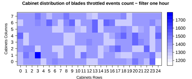
Fig. 10: Spatial distribution of throttled blades with 1-hr filter.
