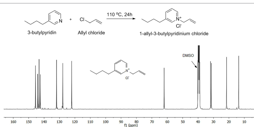
FIGURE 1 | Synthesis pathway and 13 C NMR result for the 1-allyl-3-butylpyridinium chloride ionic liquid.
