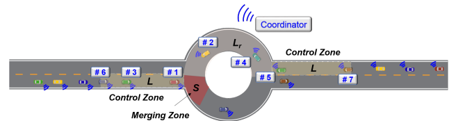
Fig. 1. A roundabout with a traffic flow of CAVs.
