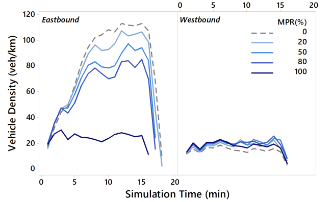
Fig. 3. Vehicle Density.
