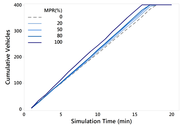
Fig. 4. Cumulative Vehicles.
