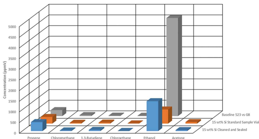
Figure 2 – Gas sampling analysis for hydrocarbons showing the differences of grab samples acquired during ARC evaluation in 18650 formats.
