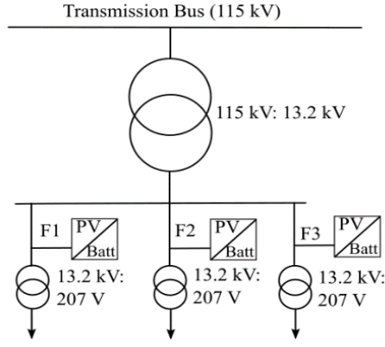
Figure 3: Simple Power Distribution System
