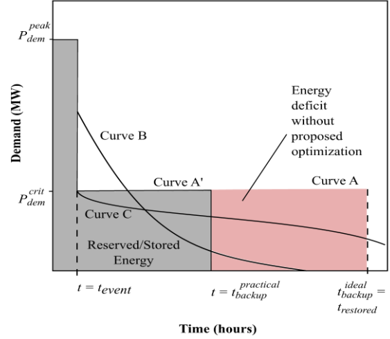
Figure 2: Visual representation of energy deficit under different operation methods
