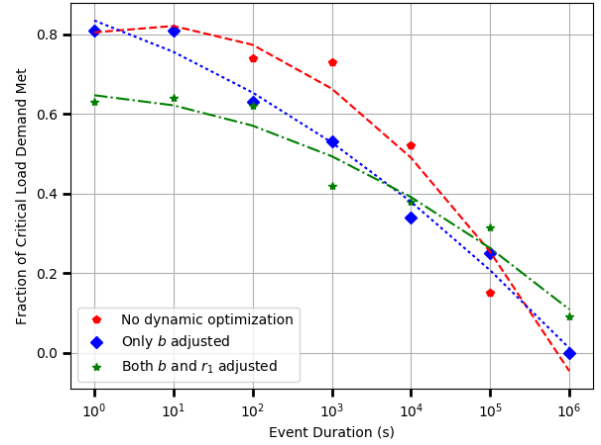
Figure 4: Impact of dynamic optimization for very long duration outages
