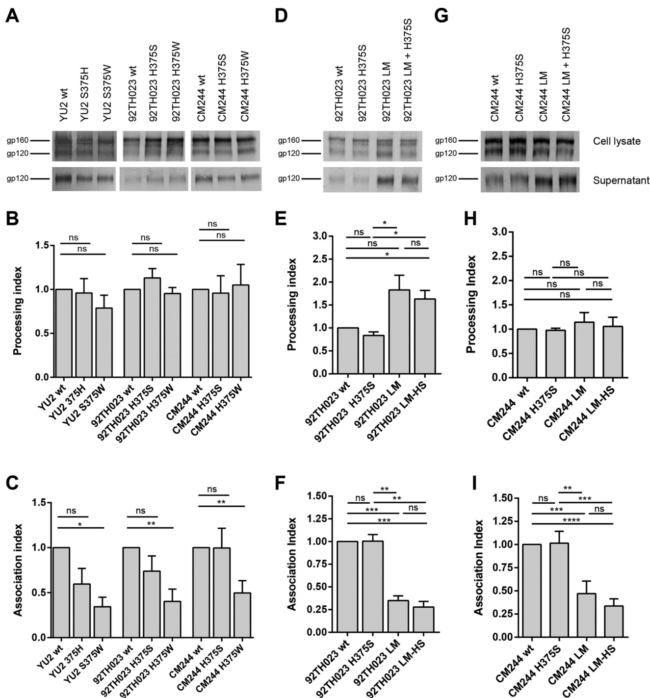
FIG 2 Effects of position 375 changes on processing and subunit association of CRF01_AE 92TH023 and CM244 Envs. Cell lysates and supernatants (SN) of ^{35}\text{S} -labeled cells transiently expressing the HIV-1 YU2 , HIV-1 CRF01_AE 92TH023 , or HIV-1 CM244 wild-type and the indicated mutant envelope glycoproteins were precipitated with HIV + sera. The precipitated proteins were loaded onto polyacrylamide gels (A, D, and G) and analyzed by autoradiography and densitometry (B, C, E, F, H, and I). Processing index (B, E and H) and association index (C, F, and I) values of each envelope, calculated as described in Materials and Methods. Data represent the averages \pm standard errors of the means (SEM) from 3 independent experiments. Statistical significance was tested using unpaired t test (ns, not significant; *, P < 0.05; **, P < 0.01; ***, P < 0.001; ****, P < 0.0001).
