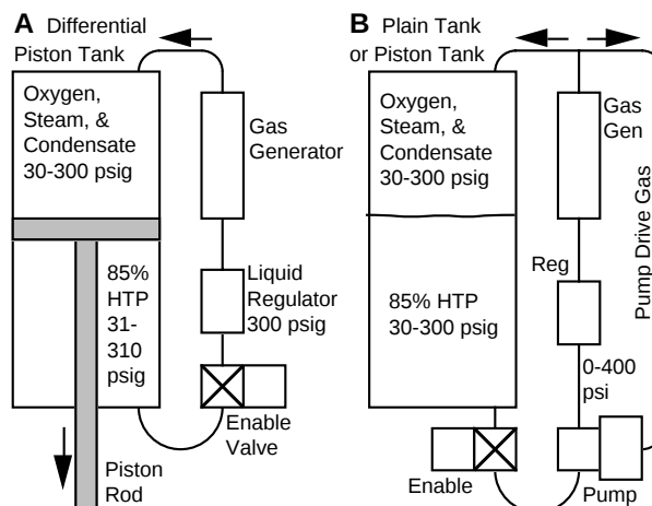
Figure 1. Options for self-pressurizing liquid tanks.
