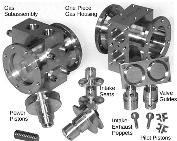
Figure 3. The gas housing and valves consist of 13 parts.
