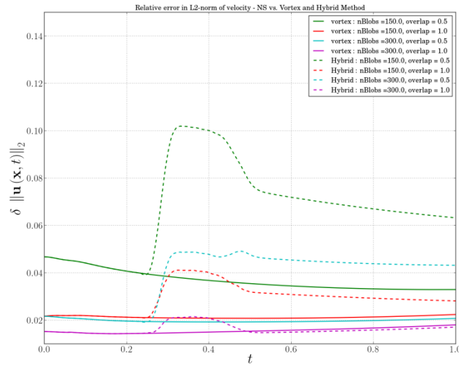
Figure 45. L2 norm error of the velocity between the pure Eulerian solution and the Hybrid solution for different number of blobs and overlap ratios.
