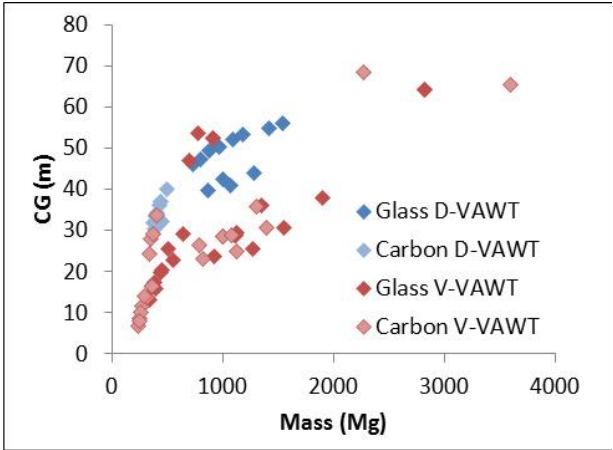
Figure 16. Rotor CG measured from water surface.
