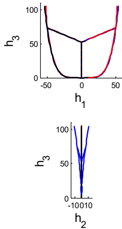
Figure 103. Flutter mode shape for VC2N5LC.
