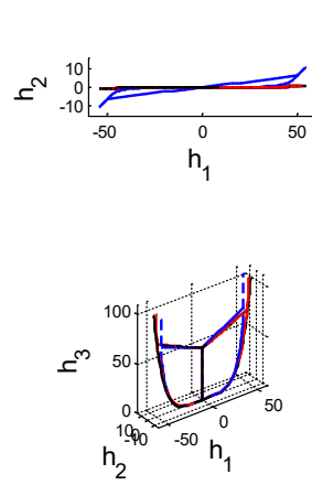
Figure 103. Flutter mode shape for VC2N5LC.
