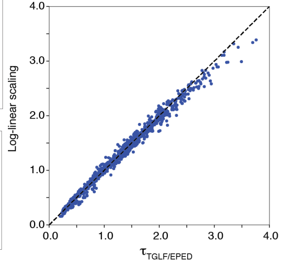
Fig 4. Accuracy of the log-linear scaling of \tau_{\text{TGLF/EPED}}
