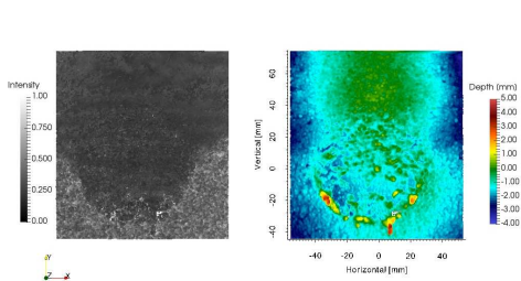
Asphalt Shingles
