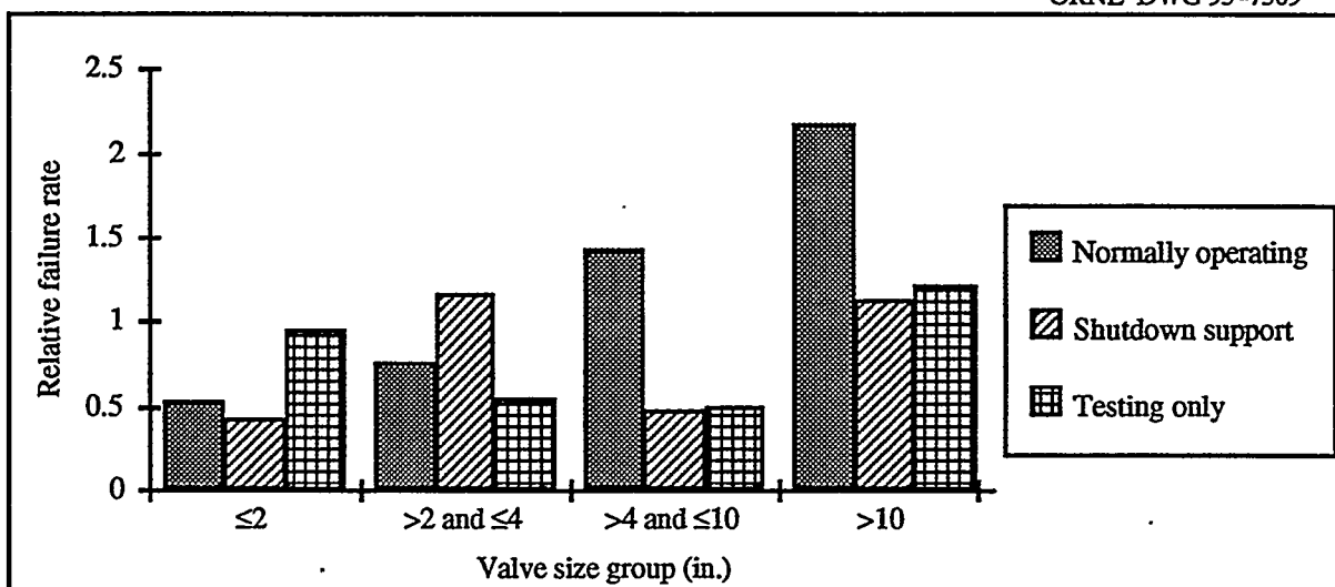
Figure 3.24 Relative failure rate by valve size group and system usage
