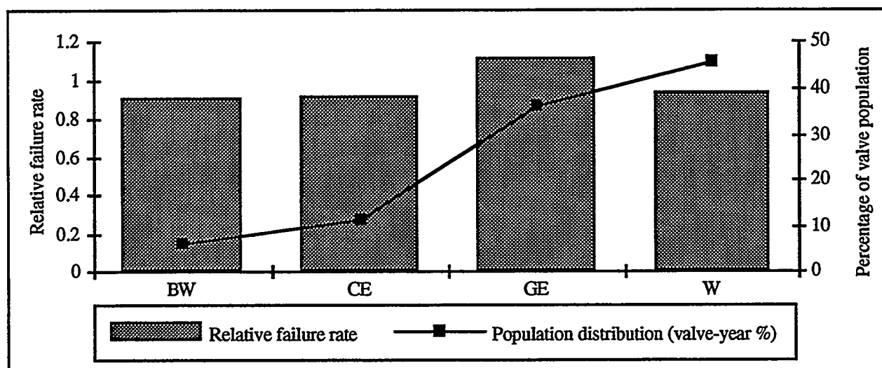
Figure 3.6 Relative failure rate and population distribution by NSSS
