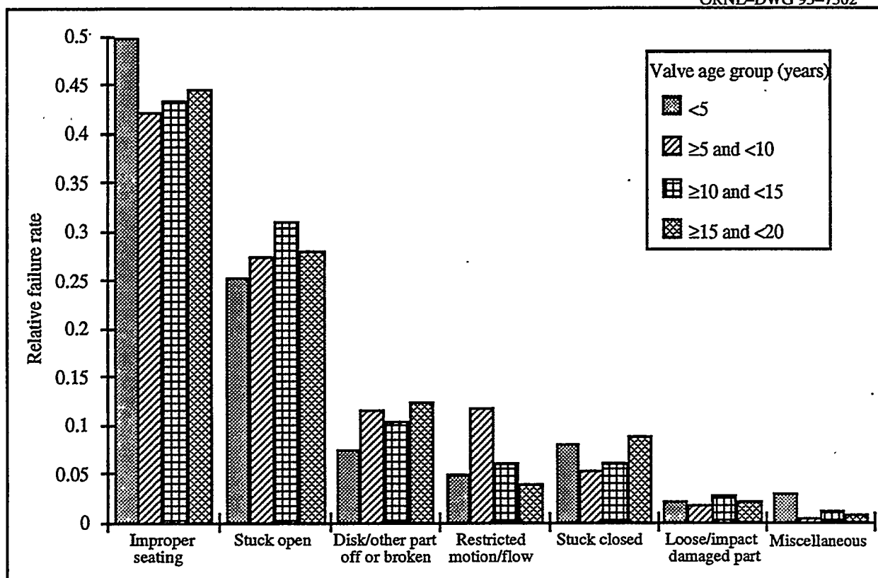
Figure 3.17 Distribution of failures by failure mode and valve age group
