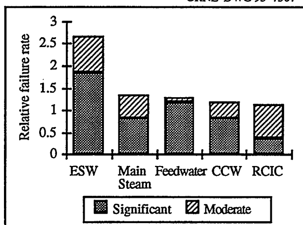
Figure 3.22 Relative failure rate and extent of degradation for valves in > 4- and ≤ 10-in. size group
