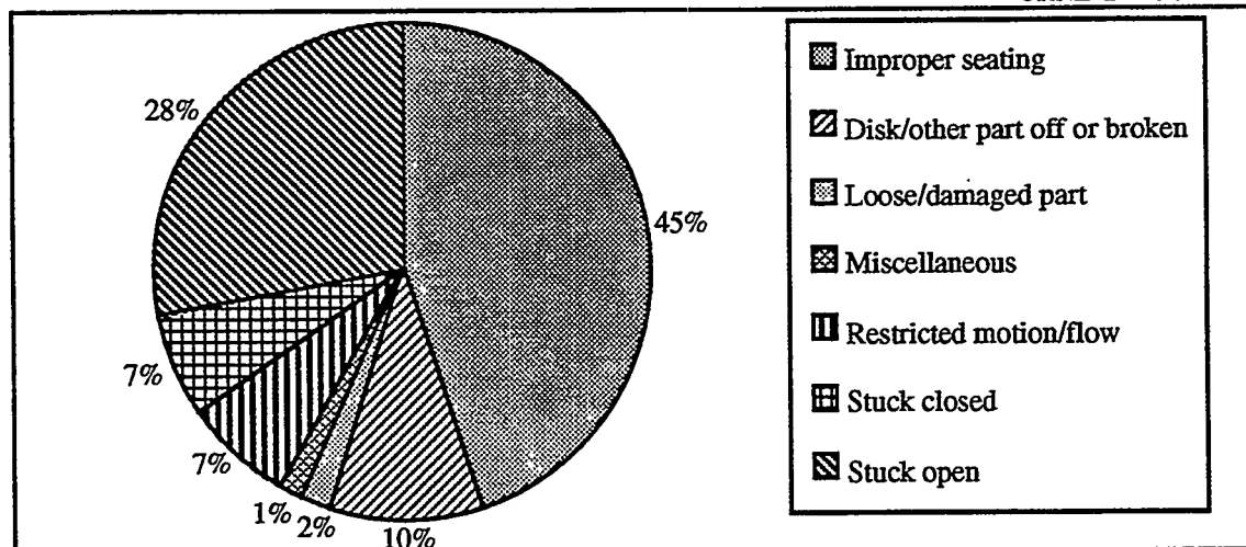
Figure 3.8 Distribution of failures by failure modes
