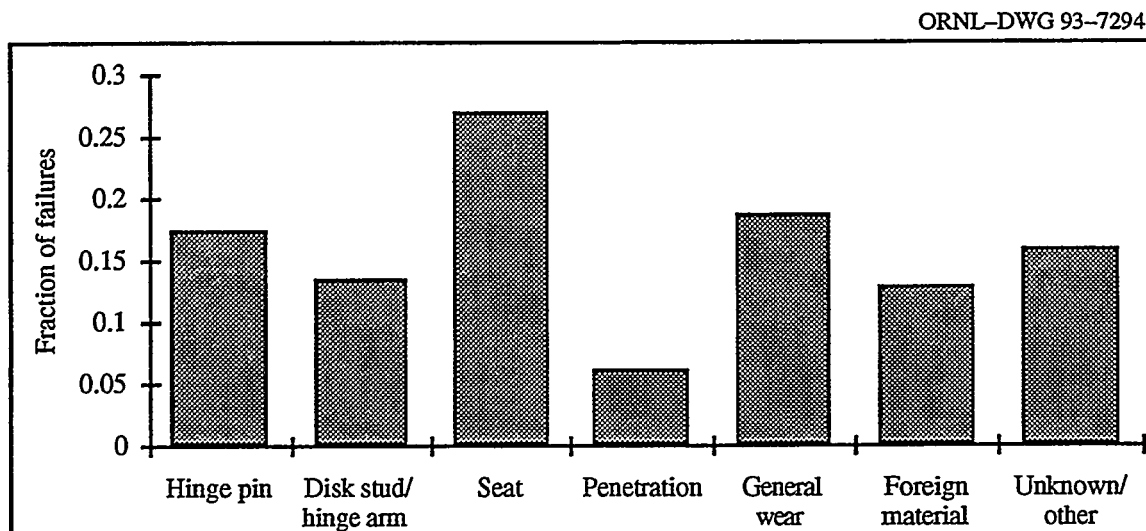
Figure 3.9 Distribution of failures by failure area or source
