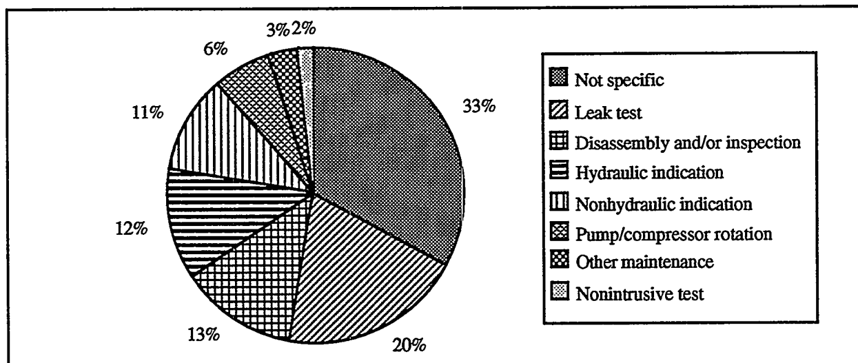
Figure 3.11 Distribution of failures by specific detection method
