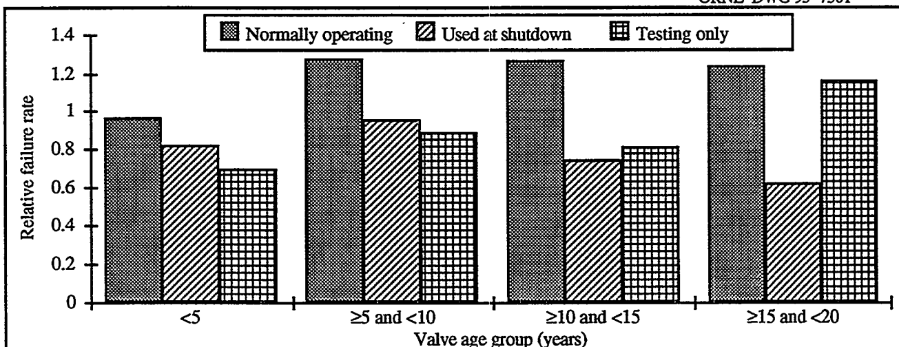
Figure 3.16 Cross-correlation of valve age group and normal system usage
