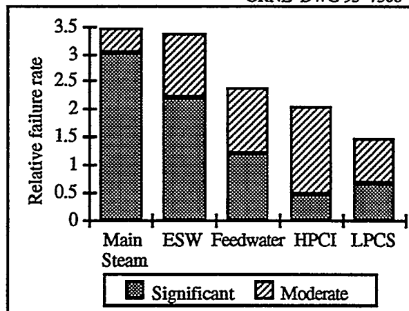
Figure 3.23 Relative failure rate and extent of degradation for valves in >10-in. size group
