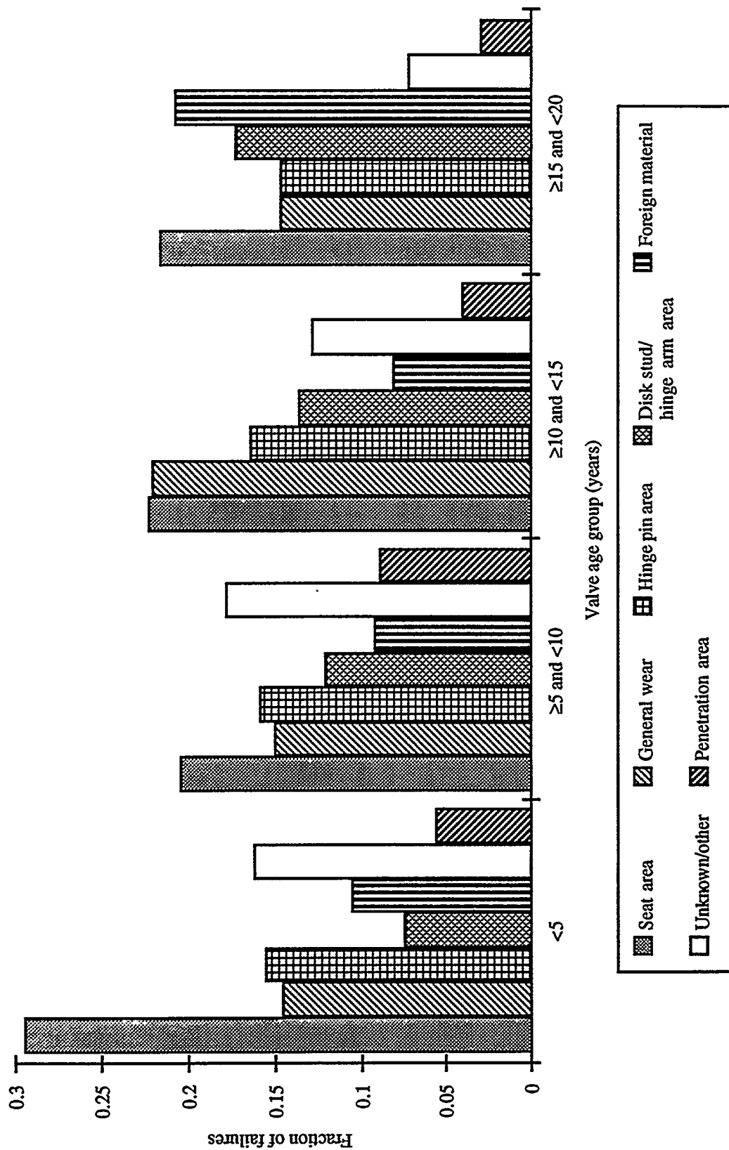
Figure A.1.9 Distribution of failures by valve age group and failure area
