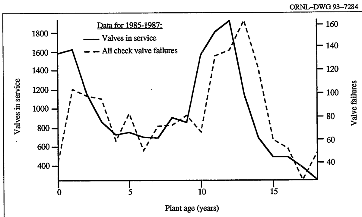
Figure 1.2 Comparison of all check valve failures and valves in service
