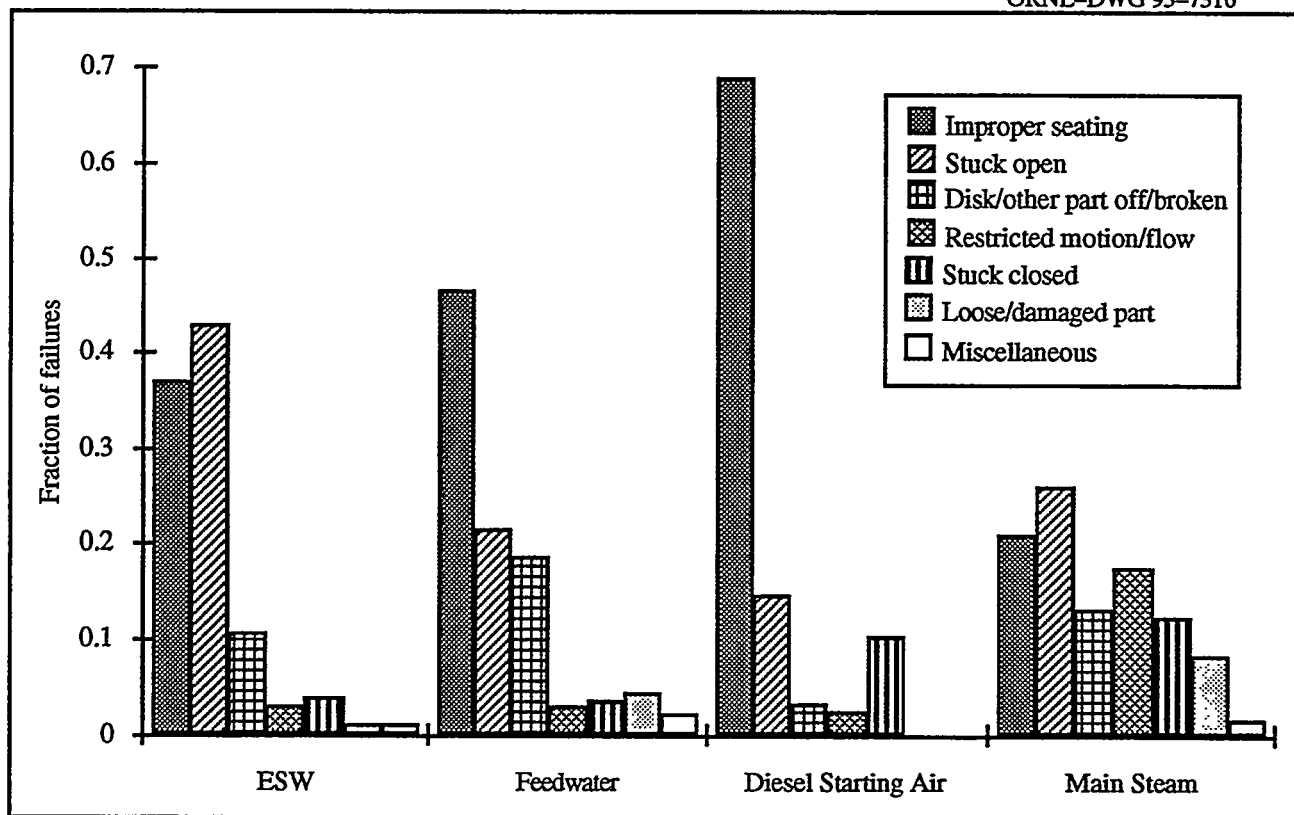
Figure 3.31 Distribution of failures by failure mode for four systems with the highest overall failure rate
