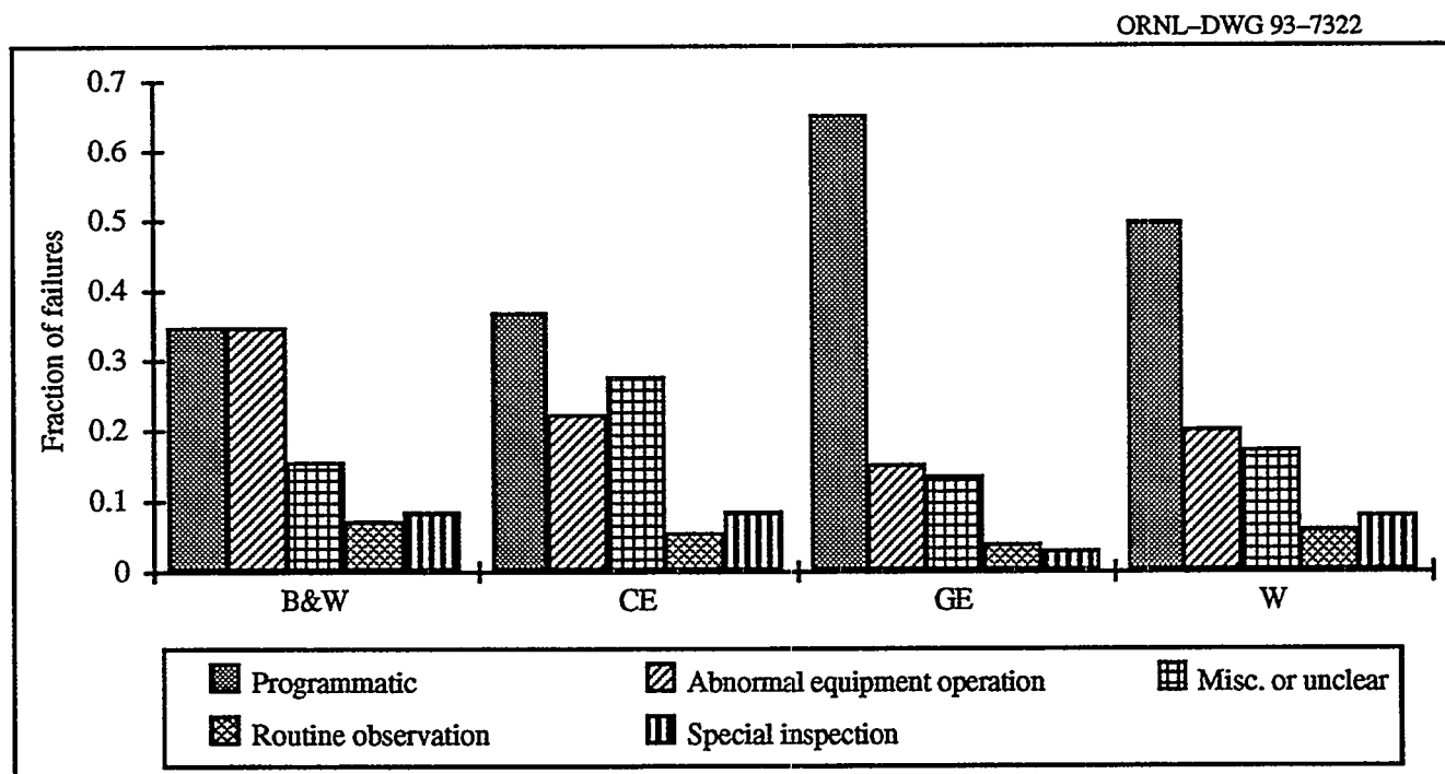
Figure 3.37 Distribution of failures by general detection method and NSSS
