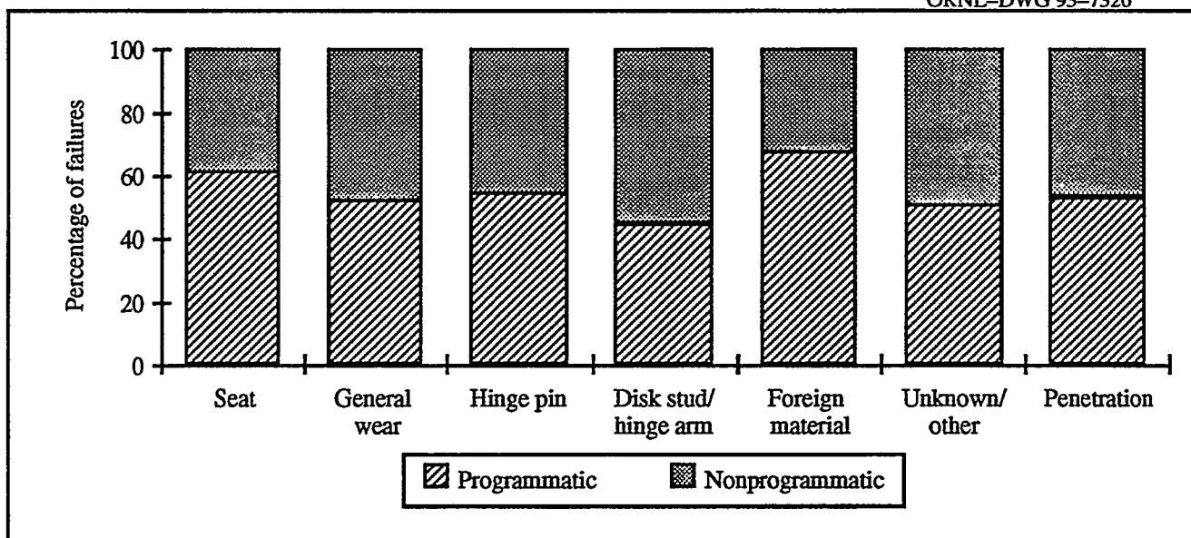
Figure 3.41 Distribution of failures by failure area and discovery process
