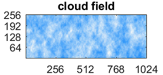
Figure 5: Initial cloud field created by summing all the interpolated fields (right plots in Figure 4).
