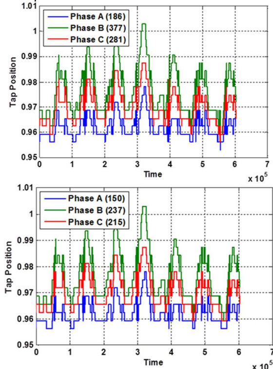
Figure 11. Voltage regulator tap change operations in a sample week for [top] a single irradiance profile used at all interconnection points and [bottom] unique irradiance profiles used at each interconnection point.
