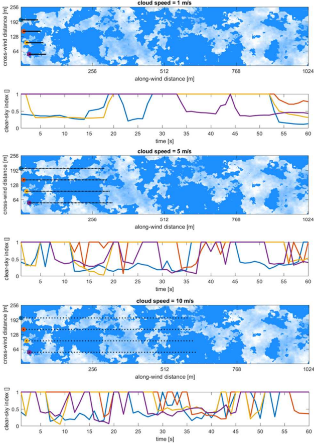
Figure 8: Timeseries created from sampling the same cloud field at different intervals corresponding to different cloud speeds.
