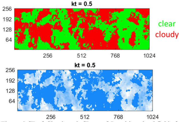
Figure 6: [Top] Cloud mask. [Bottom] Resulting cloud field after mask is applied.
