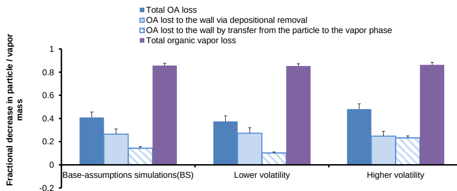
Figure 6. The organic species mass budgets for the base-assumption simulations and two sensitivity studies using bounding volatility distributions. All other variables as in Fig. 3b.
