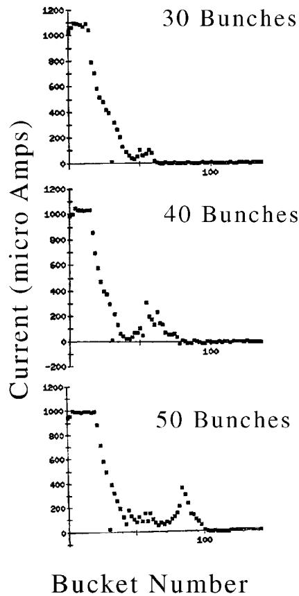
Figure 18: Measured current distribution along bunch trains of variable length after turning off the transverse feedback loops as measured by a beam current detector. The spacing between bunches was two buckets, or 4.2 ns.
