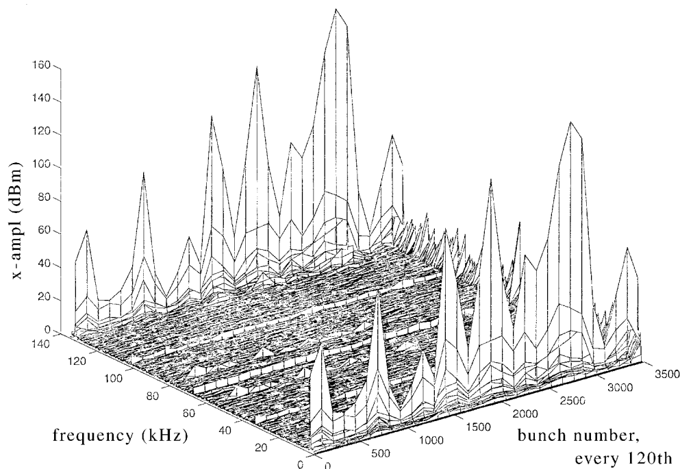
Figure 36: Horizontal Fourier spectra obtained using BPMs sampling a single bunch in a 291 bunch uniform fill as a function of distance along the fill pattern. The total beam current was 200 mA.
