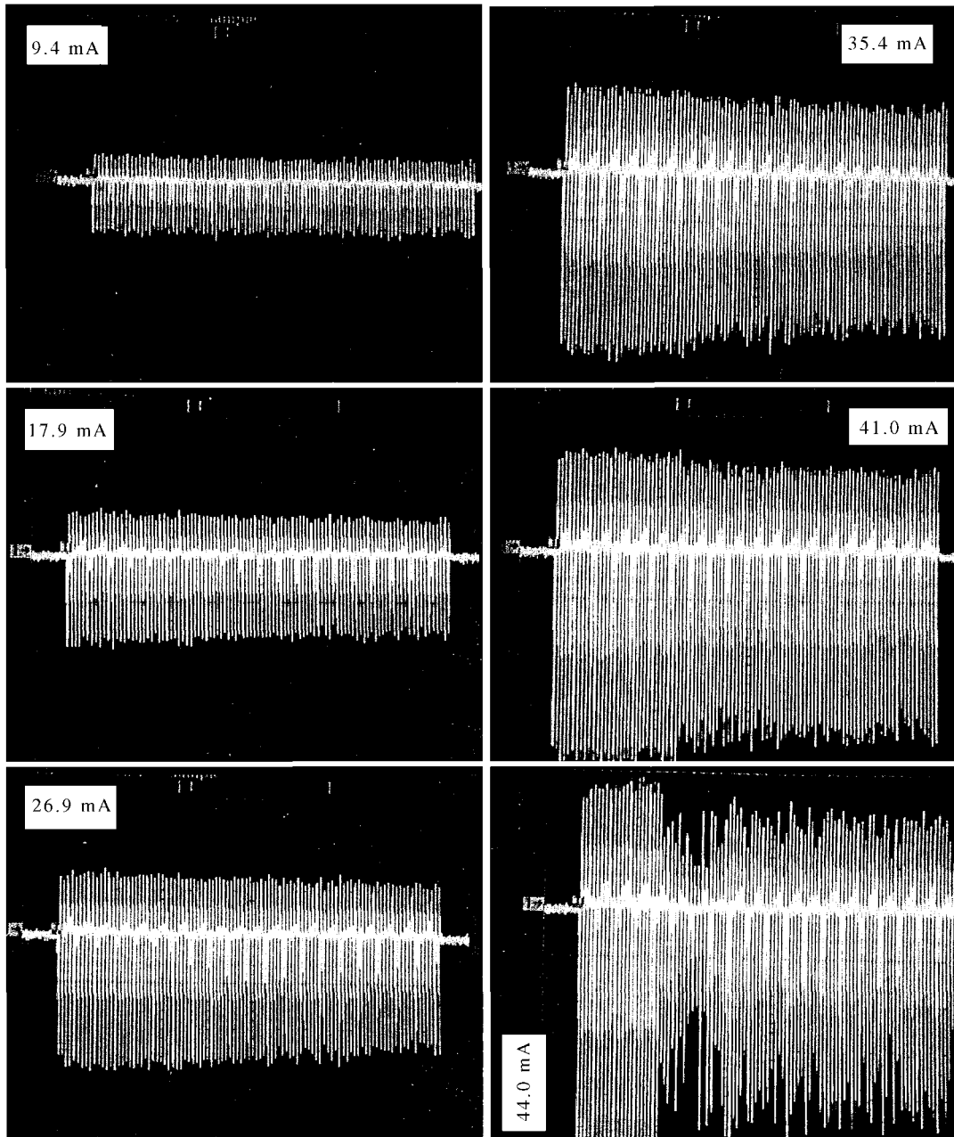
Figure 27: Bunch intensity monitor data with a 100 bunch train spaced by 4 buckets with transverse feedback off at different beam currents.
