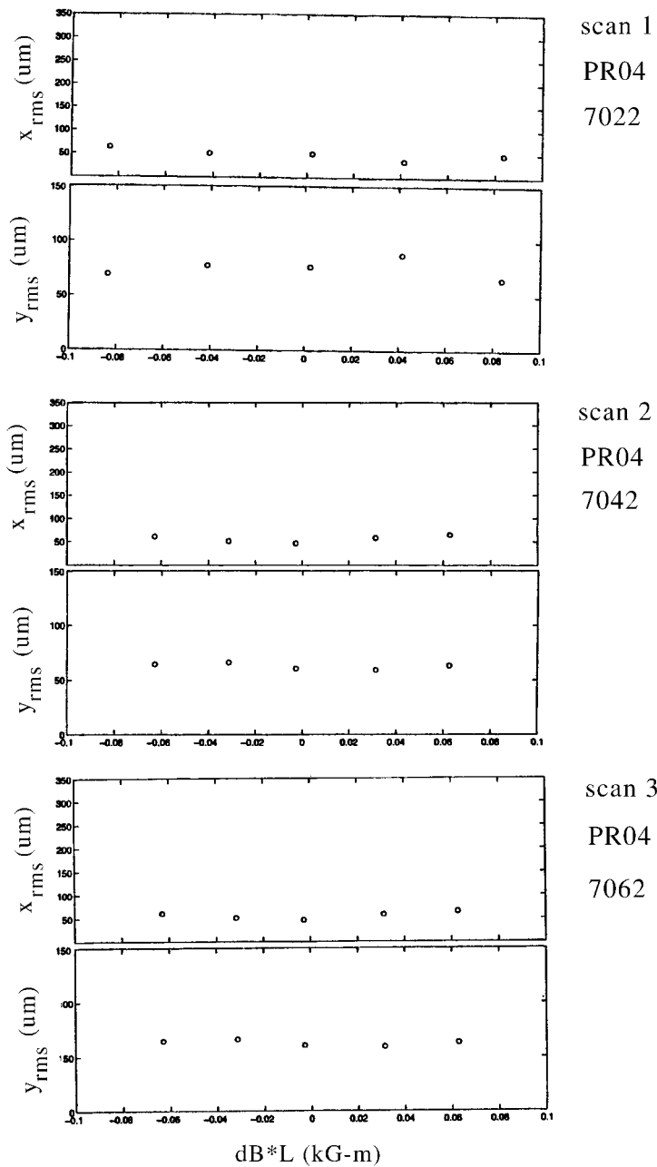
Figure 10: Measured BPM rms versus horizontal global orbit distortion with a 97-10 bunch fill pattern. Three correctors were used to fully span the HER 60° lattice. The full scale on the horizontal axis corresponds to \pm 5 mm. The betatron tunes were \nu_x = 0.6098 and \nu_y = 0.6283 . Transverse feedback was off.
