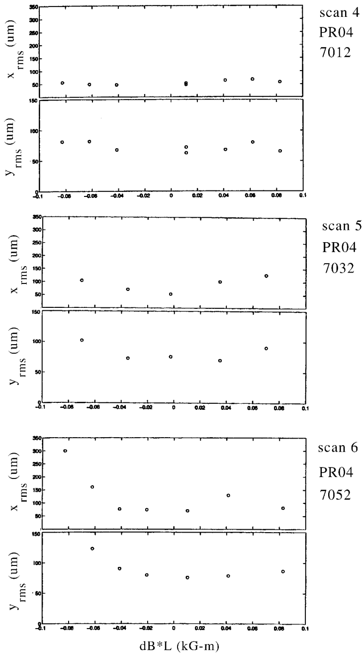
Figure 11: Measured BPM rms versus vertical global orbit distortion with a 97-10 bunch fill pattern. Three correctors were used to fully span the HER 60^\circ lattice. The full scale on the horizontal axis corresponds to \pm 5 mm. The betatron tunes were \nu_x = 0.6098 and \nu_y = 0.6283 . Transverse feedback was off.
