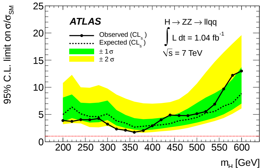
Figure 4: The expected (dashed line) and observed (solid line) upper limits on the total cross section divided by the expected SM Higgs boson cross section, calculated using CL_s at 95%. The green and yellow bands, obtained from interpolating pseudoexperiments, indicate the one- and two-sigma ranges in which the limit is expected to lie in the absence of a signal. The dotted red line shows the SM value of unity.
