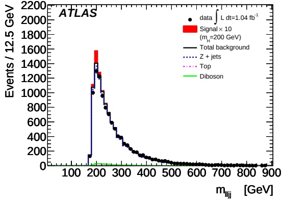
(a) Low- m_H , untagged selection.
