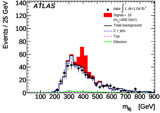
(c) High- m_H , untagged selection.
