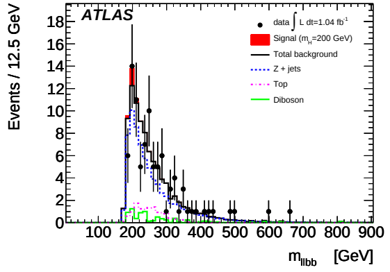
(b) Low- m_H , tagged selection.
