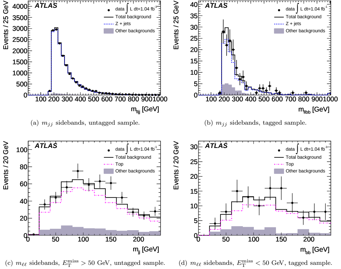
Figure 2: Distributions from the background control samples, after application of scale factors. Top row: the \ell\ell jj invariant mass for 40 \text{ GeV} < m_{jj} < 70 \text{ GeV} or 105 \text{ GeV} < m_{jj} < 150 \text{ GeV} after the jet and E_T^{\text{miss}} requirements, for (a) the untagged and (b) the tagged sample. Bottom row: the invariant mass of the jj system for events with 60 \text{ GeV} < m_{\ell\ell} < 76 \text{ GeV} or 106 \text{ GeV} < m_{\ell\ell} < 150 \text{ GeV} for (c) the untagged sample with the additional requirement E_T^{\text{miss}} > 50 \text{ GeV} and (d) the tagged sample with E_T^{\text{miss}} < 50 \text{ GeV} .
