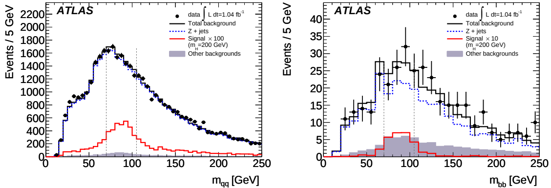
Figure 1: Distributions of the invariant mass of selected dijet pairs, m_{jj} , for the data and the MC simulation, for the untagged (left) and tagged (right) samples. The signal has been scaled up to make it more visible. The vertical lines show the range of the m_{jj} selection.
